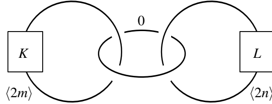
Figure 3: The surgery diagram for the upside-down cobordism \bar{W} from S_{2m}^3(K)\#S_{2n}^3(L) to S_{2(m+n)}^3(K\#L) . The coefficients in brackets represent the negative boundary \partial_- W .
