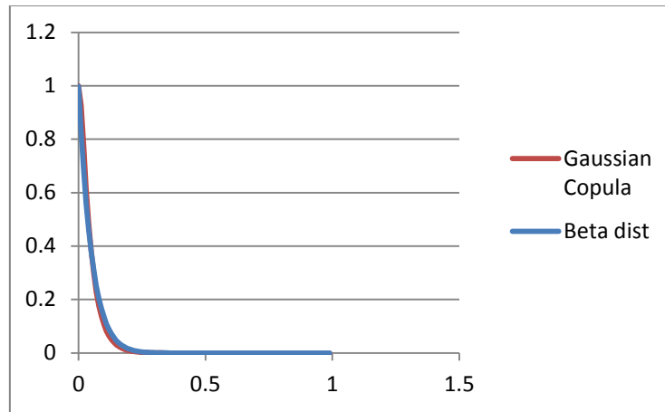
Figure 7. Densities for beta with c.d.f. F(x) = 1 - (1-x)^{19} and the Gaussian copula distribution with probability of default PD = 0.05 and \rho = 0.13 .
