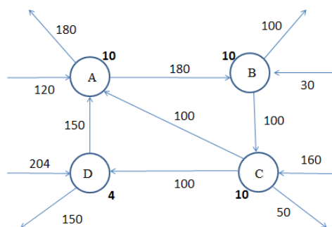
Figure 3. A hypothetical financial network showing payments due. The net worth of each node is shown in bold. The outside sector consists of households and nonfinancial firms.
