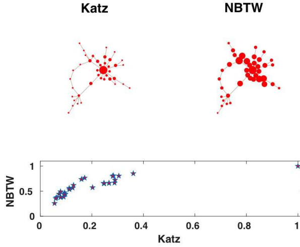
FIG. 12.1. Centrality measures for a preferential attachment network. Upper pictures have node size proportional to Katz (left) and NBTW (right) centrality. Lower picture scatter plots the two centrality measures.
