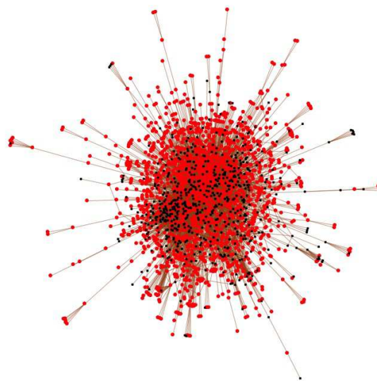
FIG. 12.6. The yeast protein interaction network from [17, 18, 21]. Essential nodes are marked with a darker symbol. (Color online.)
