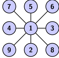
FIG. 3.1. A star graph with n = 9 vertices.
