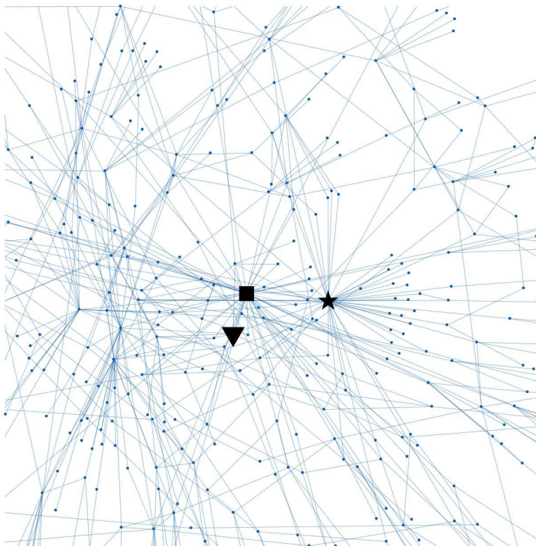
FIG. 12.5. Zoom of the visualization in Figure 12.3.
