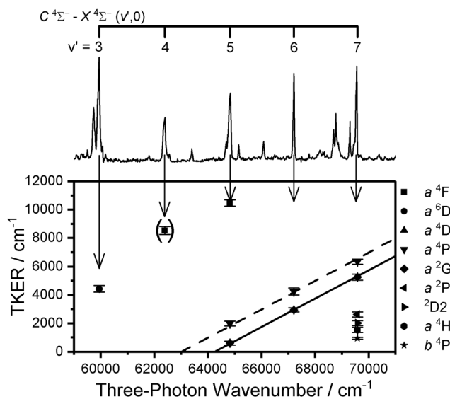
Fig. 7 Bottom: Peak positions in the TKER spectra extracted from \text{V}^+ images recorded at energies corresponding to the C^4\Sigma^-(v' = 3-7)-X^4\Sigma^-(v'' = 0) vibronic transitions of VO plotted as a function of three-photon energy. Top: The (1 + n ) REMPI spectrum of VO included for visual comparison. The error bars represent the FWHM of the peak in consideration. The dashed and solid lines represent the simulated TKER for the a^4\text{P} and a^2\text{G} series, respectively. The TKER peak corresponding to the energy of the v' = 4 vibronic band is shown in parentheses to indicate the poor quality of the \text{V}^+ image recorded at this band position.
