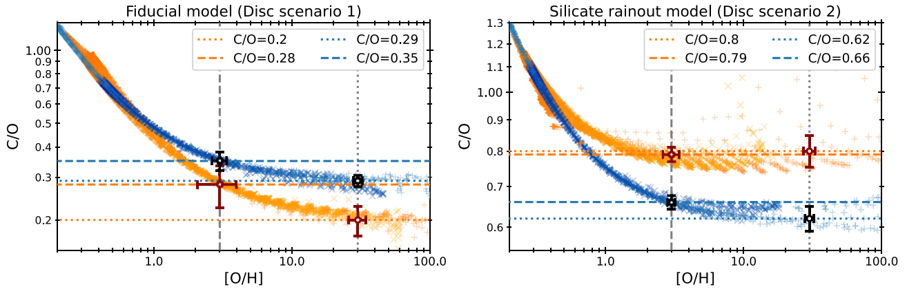
Figure 4. The C/O and [O/H] ( = Z ) results of two models from the suite of models run in Penzlin & Booth et al. (2024). Left panel: The C/O and [O/H] from the fiducial model (disc scenario 1), showing that aligned, disc-migrated planets (orange points) tend towards lower C/O than misaligned, high-eccentricity migrated planets (blue points) due to the accretion of O-rich ices in the inner disc. The dashed and dotted lines indicate the two values of metallicity and four values of C/O that were adopted in our simulation setup here. The white circles with uncertainties show the precision with which we’ll be able to measure these values from an eight-planet sample. Specifically, the uncertainties are the result of co-adding four aligned planets (red error bars) and four misaligned planets (black error bars), assuming each planet has the same mean C/O and [O/H] , as set by the dashed/dotted lines. Right panel: The C/O and [O/H] from the silicate rainout model (disc scenario 2), whereby silicates do not release their O into the atmospheres of exoplanets upon accretion. In this case, aligned, disc-migrated planets (orange points) tend towards higher C/O than misaligned, high-eccentricity migrated planets (blue points). Again, the dashed and dotted lines indicate the two values of metallicity and four values of C/O that were adopted in our simulation setup here.
