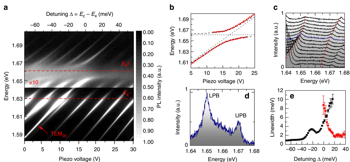
Figure 2 | Observation of strong exciton-photon coupling in a MoSe 2 single-QW heterostructure. (a) A clear anticrossing in PL is observed between the discrete cavity mode energies and the neutral exciton energy at 4.2 K. The longitudinal resonance is labelled TEM 00 . (b) The upper and lower polariton branches are fitted for the longitudinal mode with a vacuum Rabi splitting of 20 meV. (c) PL spectra of the longitudinal mode at various exciton-photon detunings from \Delta = -16 meV (bottom) to \Delta = +12 meV (top). (d) The PL spectrum on resonance shows the UPB and LPB well resolved. (e) The linewidth of the LPB and UPB as a function of detuning (black and red symbols, respectively). On resonance, the linewidth for LPB and UPB is around 4.8 and 8.5 meV, respectively. At a negative detuning of \Delta = -25 meV, the LPB is broadened due to weak coupling with the charged exciton state.
