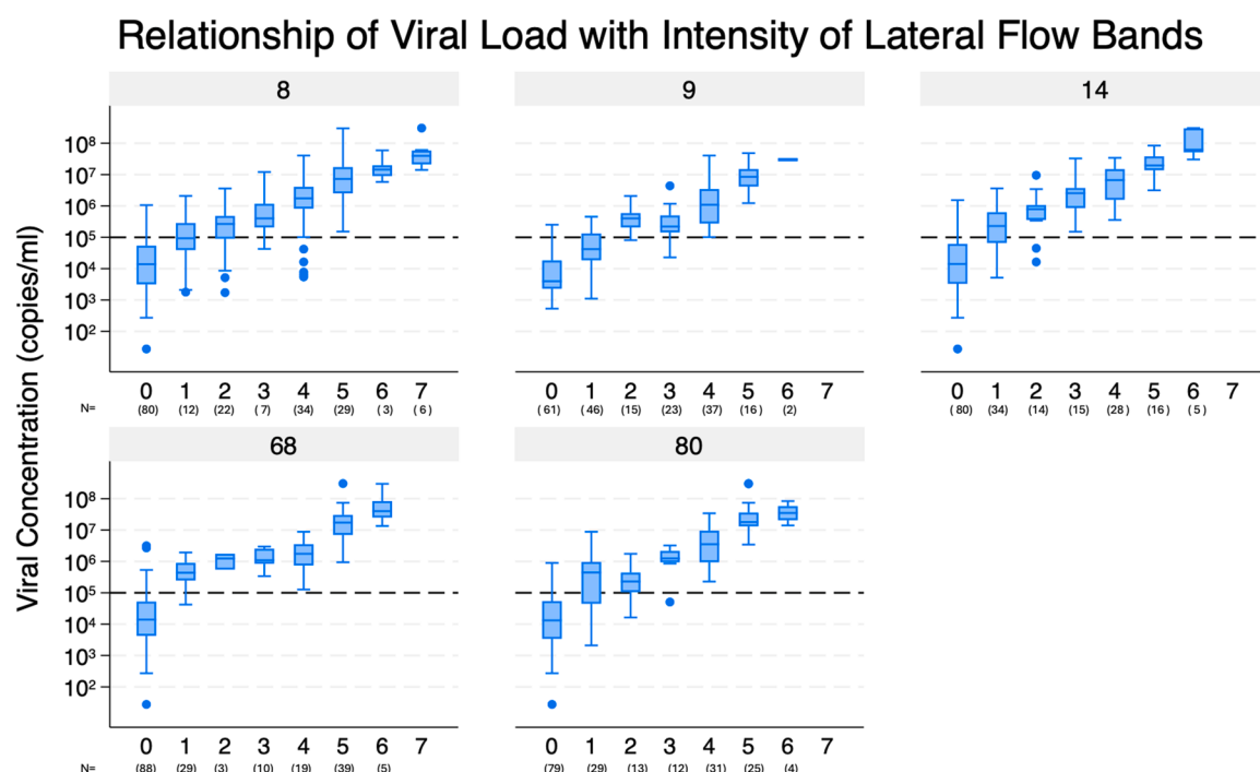
Fig. 3: Relationship of viral concentration with intensity of LFD bands for the five kits purchased by the UK government. Individual graph number = kit reference listed in Supplementary Table S1 , x-axis 0–7 = LFD band intensity values (negative to very strong) N = number of LFDs with that band value in phase 3 sensitivity testing, y-axis = viral concentration (log RNA copies/ml), dashed line represents phase 2 sensitivity pass cut-off. Higher band values with lower viral concentration indicate more sensitive tests. Box plot shows the median, IQR, the whiskers are 1.5*IQR and the outliers are outside the 1.5*IQR range.
