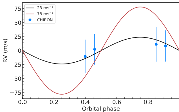
Figure 8. CHIRON RV data (blue points with error bars). A model with semi-amplitude of 23 \text{ m s}^{-1} (corresponding to the median of the credible interval) is shown with a black line. A model with semi-amplitude of 78 \text{ m s}^{-1} (corresponding to the 99% credible interval) is shown with a red line.
