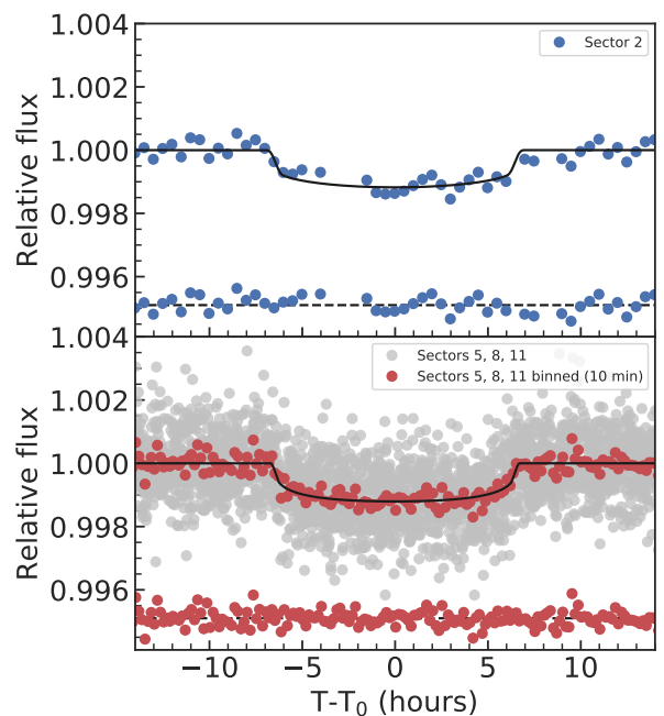
Figure 9. Phase-folded TESS light curve of TOI 813 b with the best-fit transit model overplotted and residuals.
