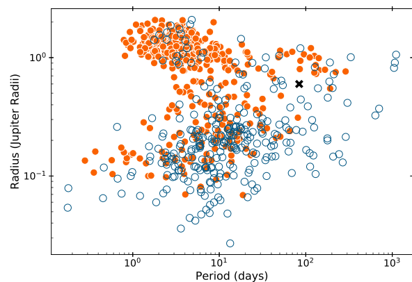
Figure 10. A log-log plot of the period vs radius of transiting exoplanets as they appear in the TEPICAT catalogue (Southworth 2011). The filled orange circles represent planets that have an at least 3-sigma mass measurement. The black cross denotes the properties of TOI813b.
