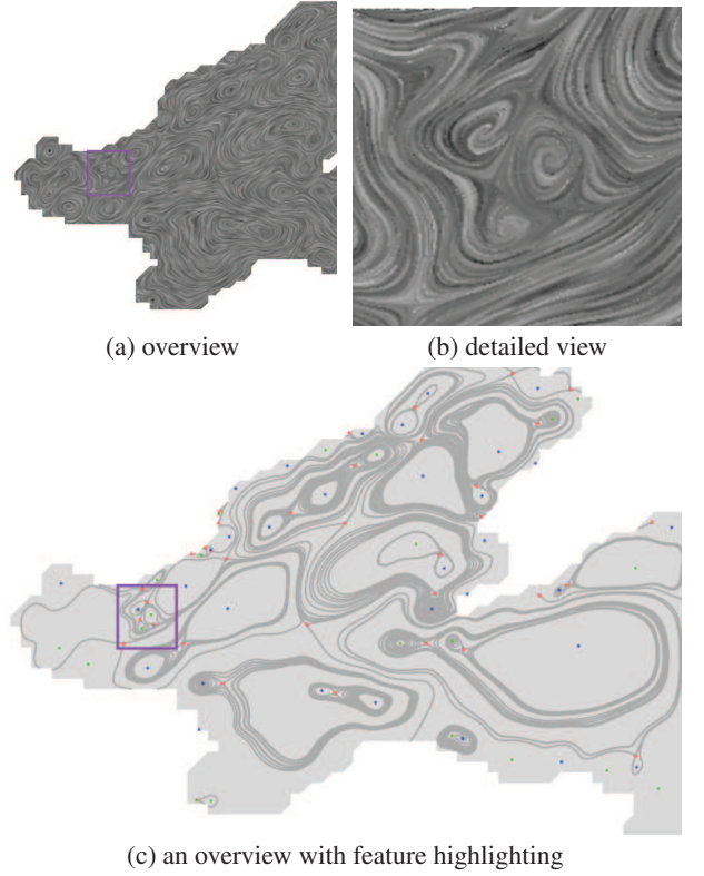
Fig. 3. An example flow visualization, where the overview in (a) may not show enough information to encourage a user to explore the detailed view in (b). Using feature extraction and highlighting, the new overview in (c) contains more feature-related mutual information about (b).
