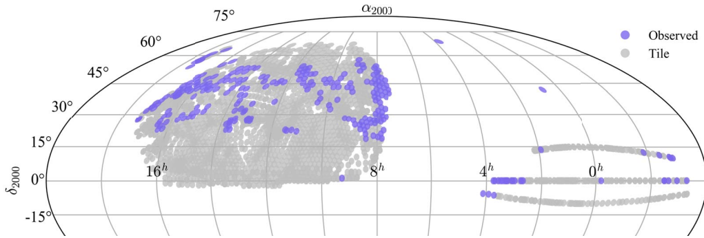
Figure 1. The sky distribution (Mollweide equatorial projection for decl. > -20^\circ ) of MaNGA plates released in DR15 (purple). This is overlaid on a plot of all possible MaNGA plates (in gray). MaNGA targets are selected from a sample with SDSS-I photometry and redshifts; hence, this footprint corresponds to Data Release 7 imaging data (Abazajian et al. 2009). Each plate contains 17 MaNGA targets, and around 30% of all possible plates will be observed in the full six-year survey. The most likely final footprint is indicated in Figure 2.
