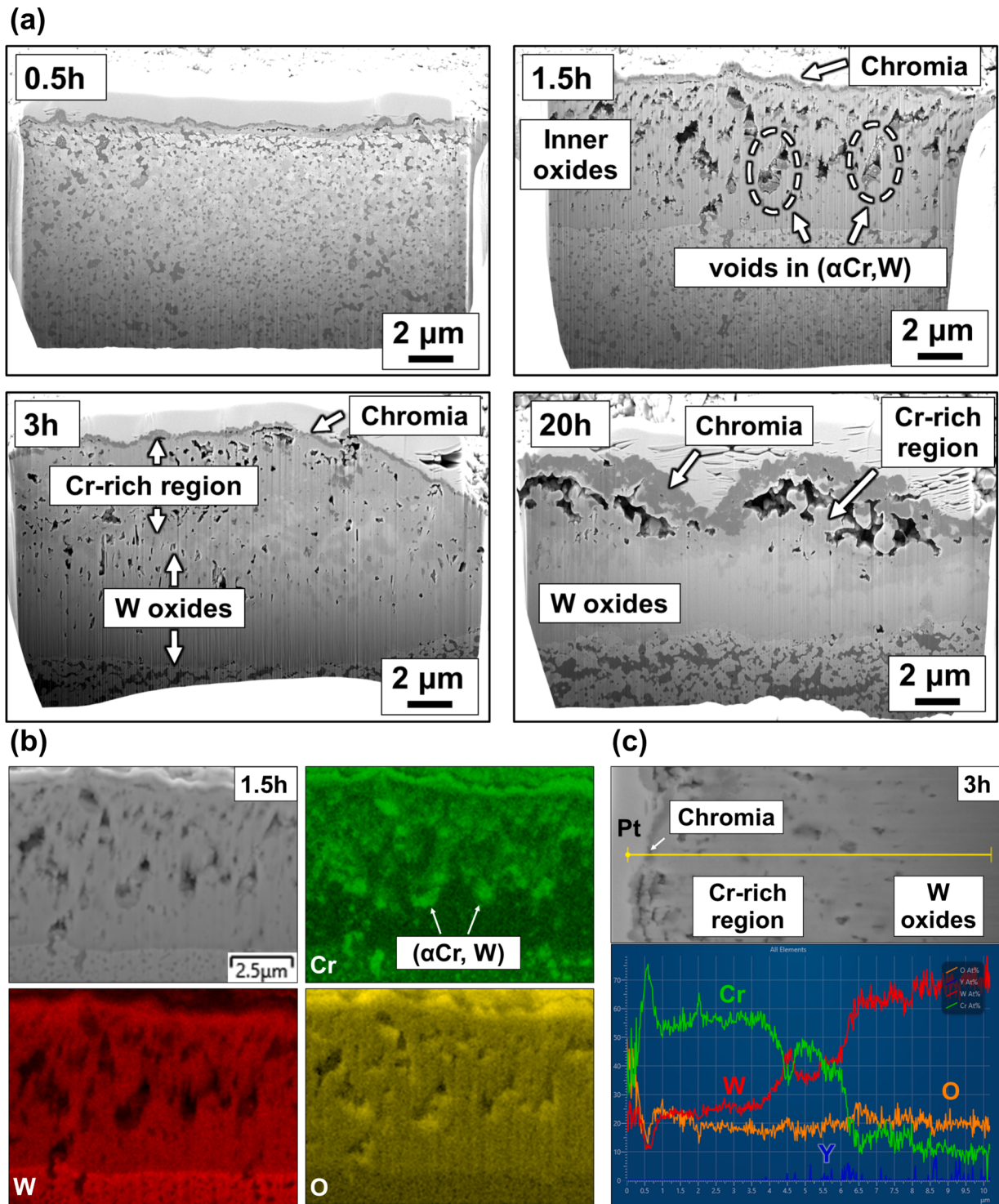
Fig. 10. (a) Cross section views of microstructural evolution at different oxidation stages of the 100 h-annealed material. (b) EDS mapping of the cross section at 1.5 h. ( \alpha\text{Cr} , W) is present in the inner oxide layer. (c) EDS line scan of the cross section at 3 h, from top (left) to bottom (right). The variation in elemental concentrations shows a Cr-rich region in the upper area of the inner oxide layer.
