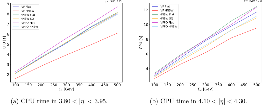
Figure 6.11: CPU consumption resulting from the validation of the new fast simulation procedure in two pseudorapidity regions, comparing different Faiss methods.
