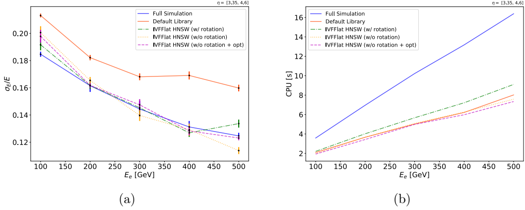
Figure 6.13: Resolution (a) and CPU consumption (b) resulting from the validation of the new fast simulation procedure, using the IVFFlat HNSW method.
