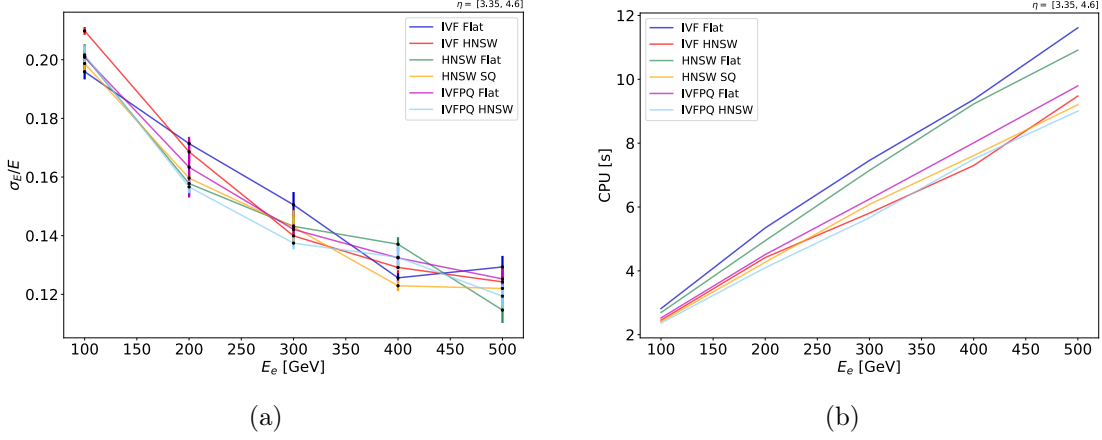
Figure 6.10: Resolution (a) and CPU consumption (b) resulting from the validation of the new fast simulation procedure, comparing different Faiss methods.
