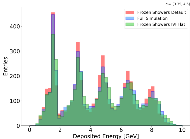
Figure 6.7: Distribution of the energy deposited by the showers originated by the low-energy electrons in the FCal calorimeter.
