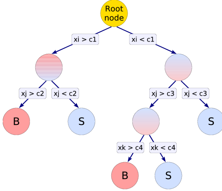
Figure 3.1: Schematic structure of a simple decision tree. Starting from the root node, the dataset is split according to a set of decision rules that determine cuts on the discriminating variables x_i . Each event of the dataset ends up in one of the leaf nodes at the bottom end of the tree, labelled S for signal and B for background. Image source: [49].
