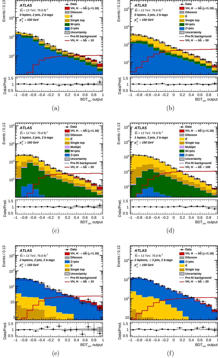
Figure 7.18: The BDT output post-fit distributions in the 0-lepton (top), 1-lepton (middle) and 2-lepton (bottom) channels for 2 b -tag events, in the 2-jet (left) and exactly 3-jet (right) categories in the high- p_T^V region.
