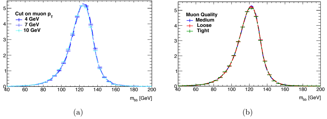
Figure 7.12: Invariant mass m_{bb} distributions for different p_T cuts (a) and muon types (b), evaluated with the ZH \rightarrow \nu\nu b\bar{b} sample.
