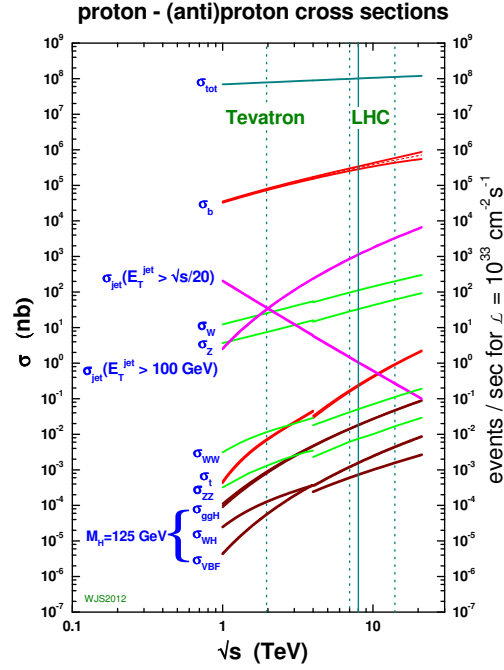
Figure 7.1: Standard Model cross sections of pp and p\bar{p} collision processes as a function of collider energy, with 125 GeV Higgs. Image source: [154].
