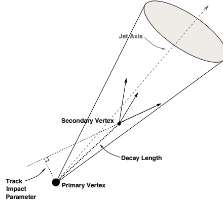
Figure 5.6: Illustration of the principle of b -hadron decay. Image source: [119].
