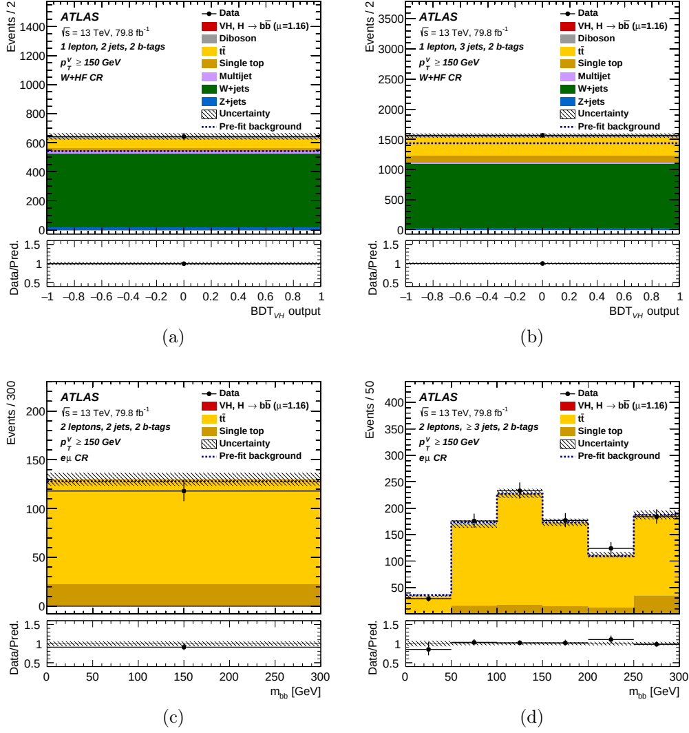
Figure 7.4: Control region distributions used as input to the global likelihood fit for the MVA analysis to extract the normalisation of the main backgrounds. Image sources: [5].
