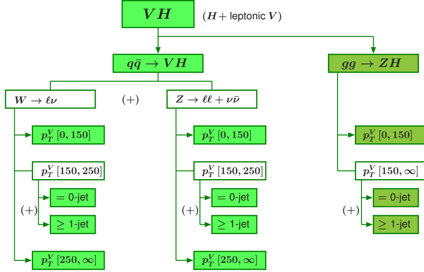
Figure 8.2: STXS stage-1 binning for associated production with vector bosons. Image source: [27].
