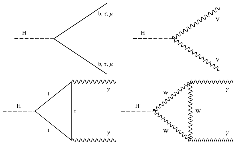
Figure 2.5: Examples of LO Feynman diagrams for the Higgs boson decay modes: H \rightarrow b\bar{b} , H \rightarrow \tau\tau , H \rightarrow \mu\mu (top left), H \rightarrow ZZ , H \rightarrow WW (top right), H \rightarrow \gamma\gamma channels (bottom row). Image source [26].
