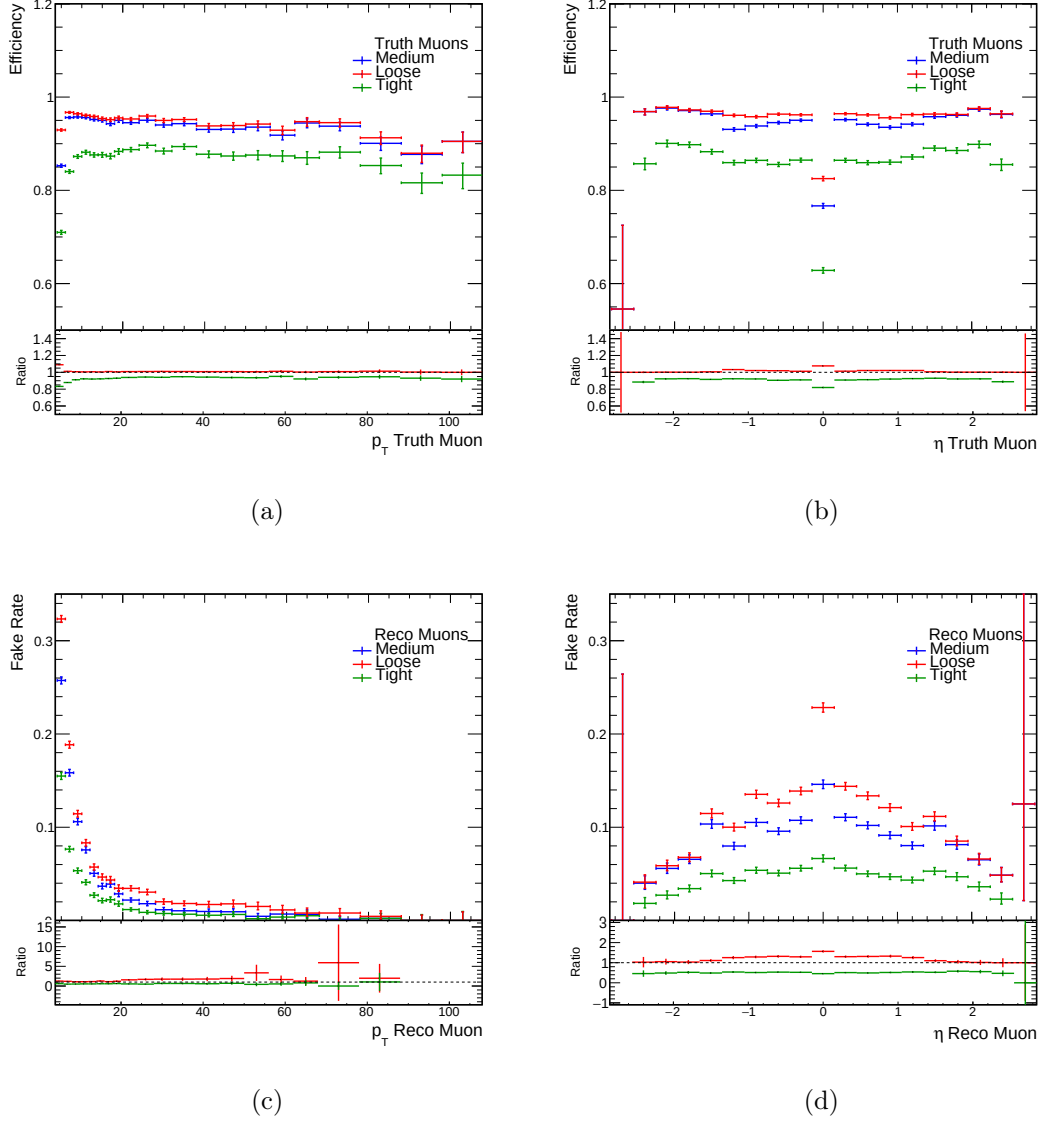
Figure 7.11: Top row: efficiency of the muon-in-jet candidates as a function of the truth muon p_T (a) and as a function of \eta (b), for various muon types. Bottom row: fake rate of the muon-in-jet candidates as a function of the reco muon p_T (c) and as a function of \eta (d), for various muon types. The lower insert of the plots represents the ratio with respect to the efficiency or fake rate corresponding to the medium selection.
