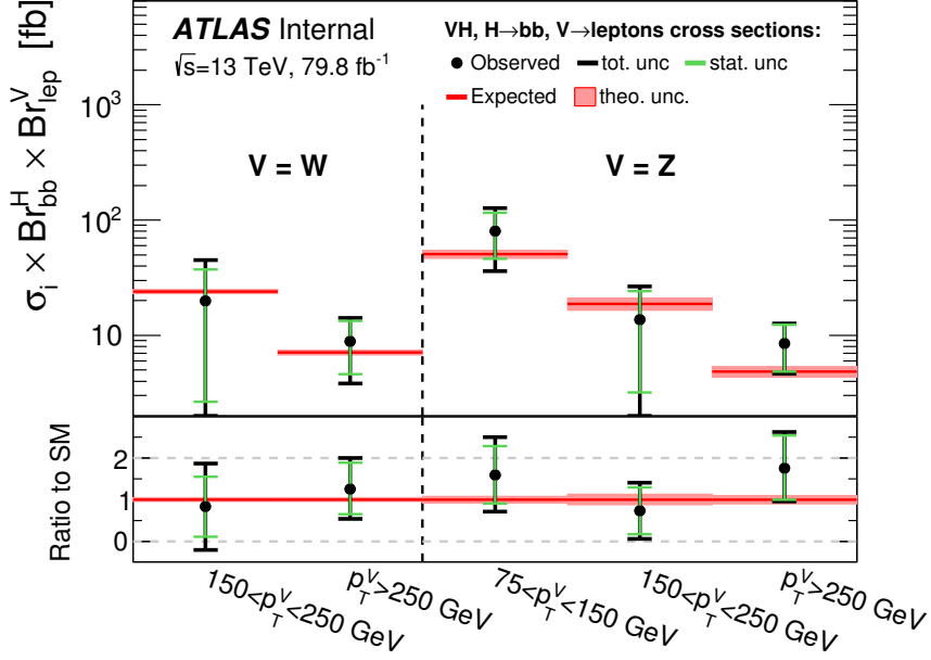
Figure 8.5: Measured VH cross sections times the H \rightarrow b\bar{b} branching ratio.
