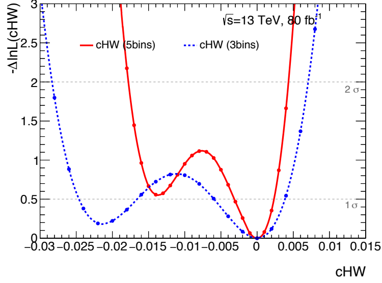
Figure 8.11: Profile likelihood for the \bar{c}_{HW} coefficient. The main results from the 5-POI model (red) are compared to the results of the 3-POI model parametrisation (blue).
