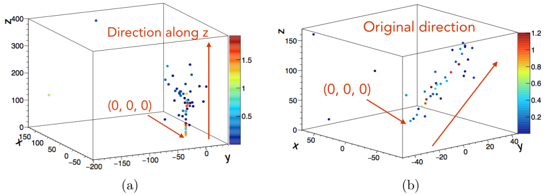
Figure 6.12: Electromagnetic showers originated by electron starting points with energy E < 1 GeV. The shower in (a) is stored in the library after translation and rotation, while the shower in (b) is stored without receiving rotation.
