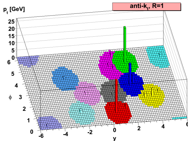
Figure 5.3: Simulation of jet reconstruction as results with the anti-k_T algorithm. Image source:[113].
