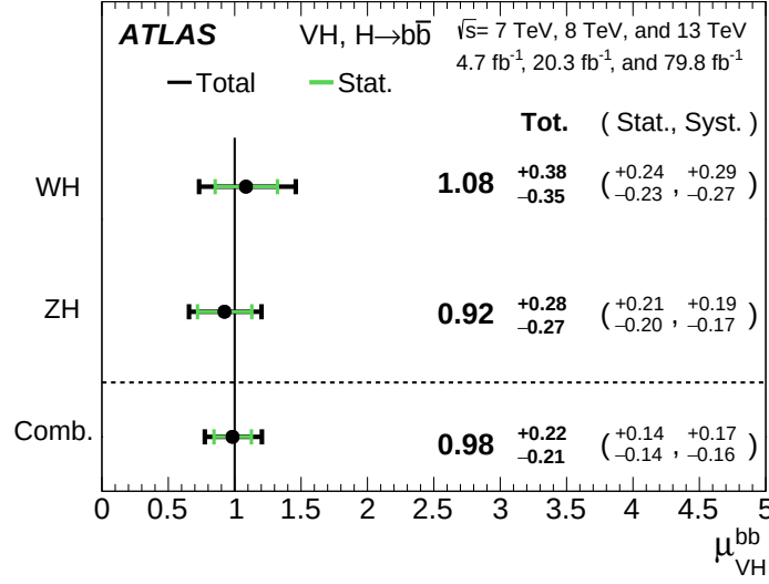
Figure 7.23: Higgs boson signal strength \mu_{VH}^{bb} for the WH and ZH processes in the combination of Run-1 and Run-2, using the 7 TeV, 8 TeV and 13 TeV data. The displayed values are the result of a global likelihood fit where the individual signal strengths of WH and ZH are left floating.
