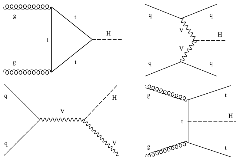
Figure 2.3: Examples of LO Feynman diagrams for the main Higgs boson production modes: gluon fusion (top left), vector boson fusion (top right), associated production with a vector boson V (bottom left) and with a pair of top quarks (bottom right). Image source [26].
