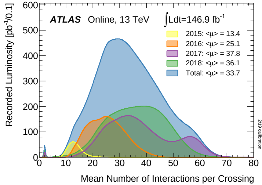
Figure 4.3: Luminosity-weighted distribution of the mean number of interactions per crossing for 2015 (yellow), 2016 (orange), 2017 (purple), 2018 (green) and total (blue), obtained with data of pp collisions at \sqrt{s} = 13 TeV. Image source: [71].
