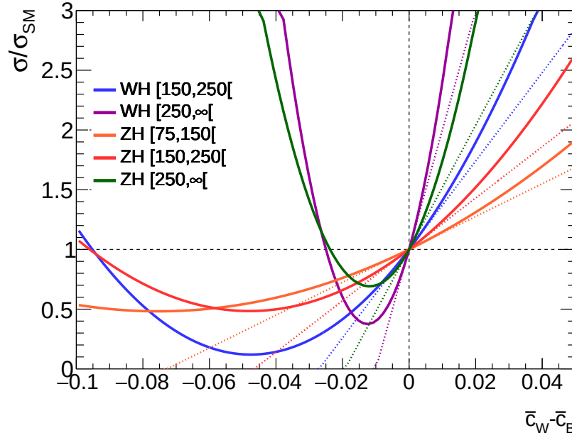
Figure 8.6: Cross section variations for each kinematic region introduced by the \bar{c}_W - \bar{c}_B coefficient. The combined linear and quadratic contributions are illustrated by solid lines, while linear contributions only are illustrated by dashed lines.
