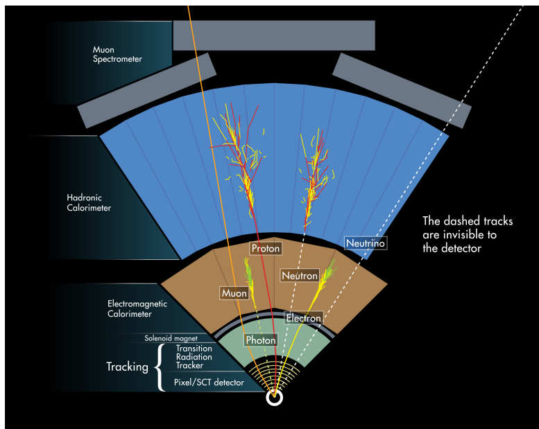
Figure 5.1: Transversal view of the particle paths in the ATLAS detector. Particles of different nature interact in different ways and in different sectors of the detector. Image source: [96].
