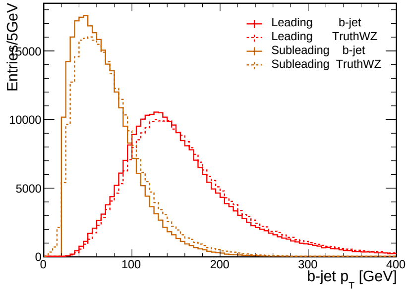
Figure 7.8: Distribution of the b -jet transverse momentum p_T , shown separately for leading (red) and sub-leading (orange) jets. The distributions of the reconstructed jets (continuous line) are compared to the truth jets (dashed line).
