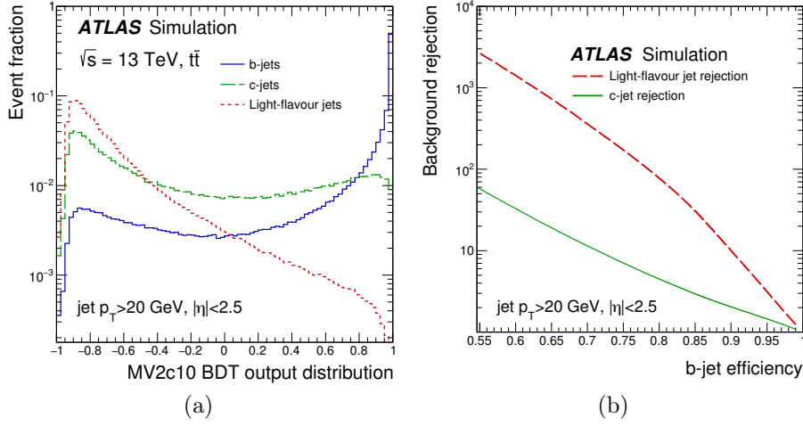
Figure 5.9: The MV2c10 output for b -jets (solid line), c -jets (dashed line) and light-flavour jets (dotted line) in simulated t\bar{t} events (a). The light-flavour jet (dashed line) and c -jet rejection factors (solid line) as a function of the b -jet tagging efficiency of the MV2c10 b -tagging algorithm (b). Image sources: [125].
