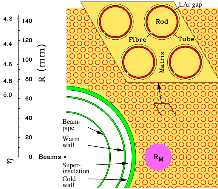
Figure 4.9: Front-face view of the electrode arrangement of a portion of the forward calorimeter (FCal) in ATLAS. Image source: [87].
