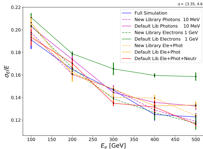
Figure 6.15: Resolution response obtained with the new (dashed lines) and the old (full lines) libraries. The photon library (purple), electron library (green) and their combination (yellow), both for the default and the new approach, are compared with the full simulation (blue) and the default simulation which uses a neutron library during the fast simulation (red).
