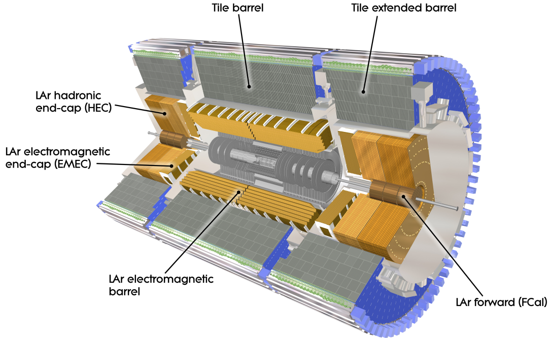
Figure 4.7: Cut-away view of the ATLAS calorimeter system. Image source: [82].
