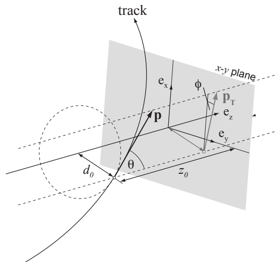
Figure 5.2: Transverse d_0 and longitudinal z_0 impact parameters of a track with respect to the interaction point. Image source: [102].
