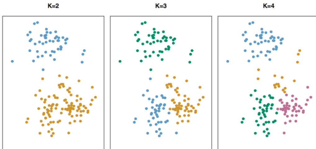
Figure 3.2: Results for K -means clustering on an unlabelled dataset. Each panel corresponds to a different K used for clustering. The different colours are assigned after the algorithm partitions the dataset. Image source: [51].
