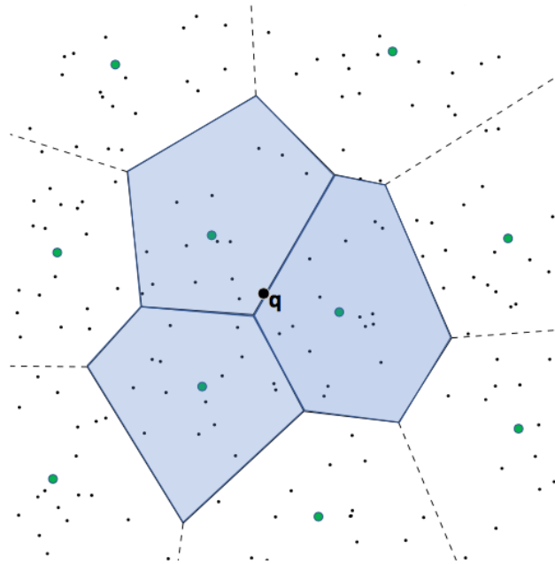
Figure 3.4: The Inverted Index partitioning obtained on a dataset of 200 two-dimensional points (small black dots). The three closest cells to the query point ( q ) are indicated in light blue. Image source: [61].
