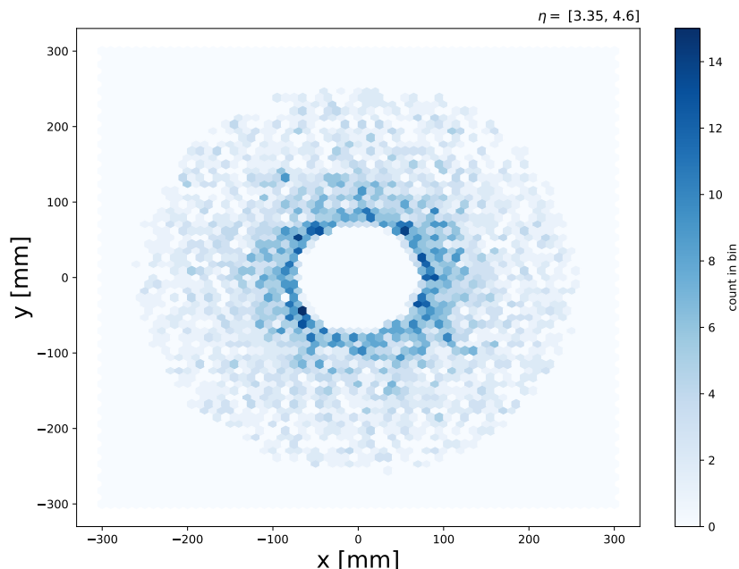
Figure 6.6: Spatial distribution of the generated high-energy electrons entering the FCal front face.
