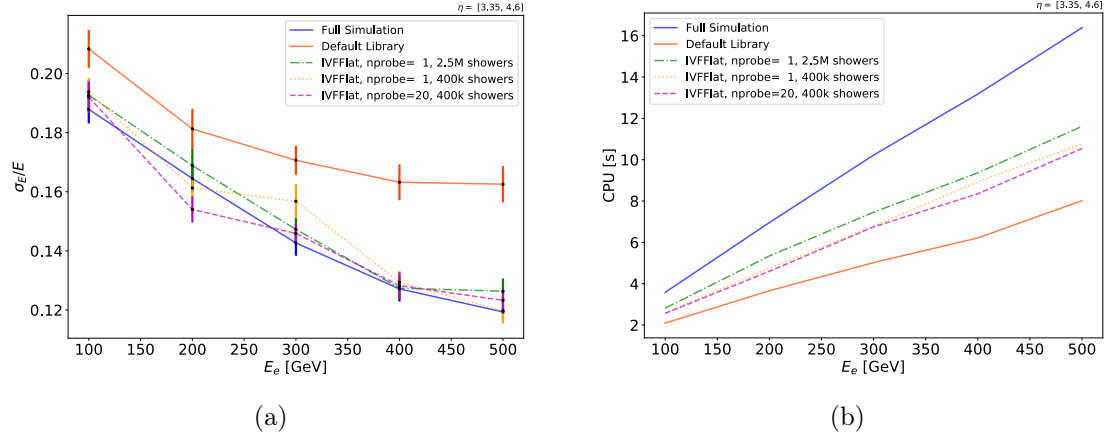
Figure 6.9: Resolution (a) and CPU consumption (b) resulting from the validation of the new fast simulation procedure, using the IVF Flat method. Results obtained with different libraries and different nprobe (green, yellow, purple) have been compared with Full Simulation (blue) and Default Library (red) results.
