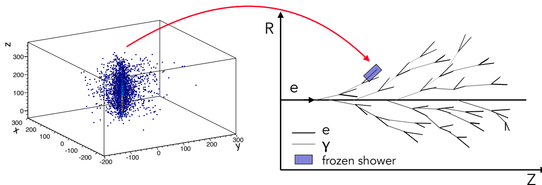
Figure 6.2: Sketch of the frozen shower substitution. On the left side, a shower (collection of hits) is shown as it is stored in the library. On the right, a low-particle produced in simulation is replaced with the stored shower.
