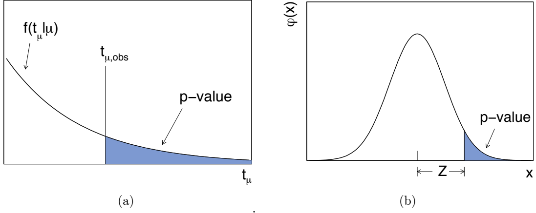
Figure 7.17: Relation between the p-value and the test statistic t_\mu (a). Relation between the p-value and the significance Z (b). Image source: [166]
