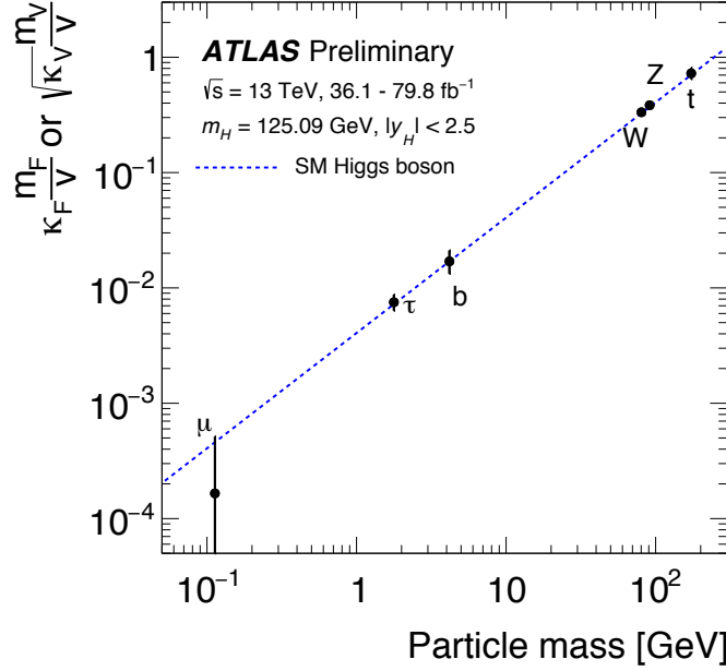
Figure 2.6: Measured coupling-strength modifiers defined as \sqrt{\kappa_V} \frac{m_V}{v} for weak bosons and as \kappa_F \frac{m_F}{v} for fermions. All the coupling scale factors are compatible with their SM expectation (dotted line). Image source [30].
