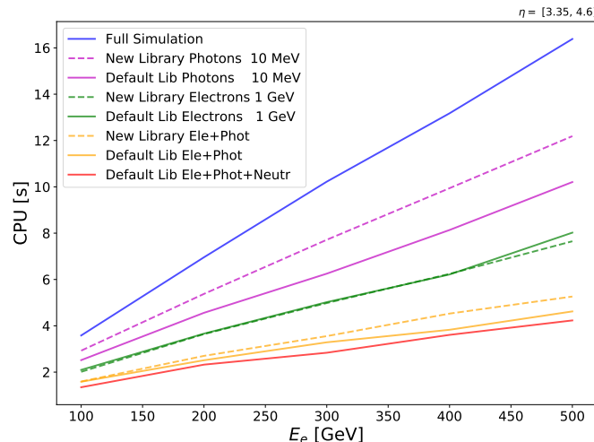
Figure 6.14: CPU response obtained with the new (dashed lines) and the old (full lines) libraries. The results come from simulations where the photon library (purple) and the electron library (green) are used individually for the fast simulation. In yellow is the response obtained with the simultaneous use of the two libraries. The results are compared with full simulation (blue) and the total default simulation which uses also a neutron library during the fast simulation (red).
