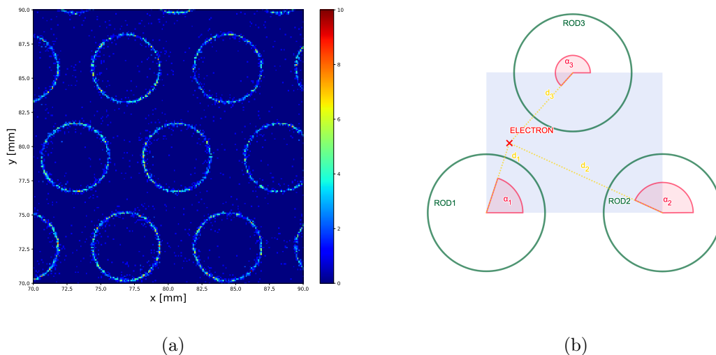
Figure 6.3: Transversal position of the shower hits collected in the FCal sub-detector (a). Scheme of three rods defining a unit cell in the structure of FCal: within the unit cell, the distance to the closest rod centre and the corresponding angle with respect to the x -axis are identified (b).
