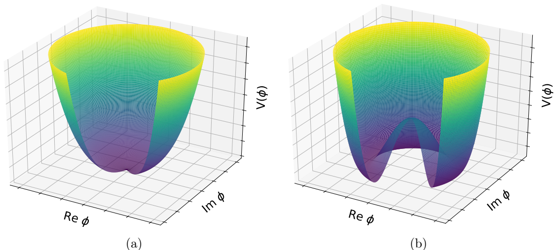
Figure 2.2: V(\phi) = \mu^2 \phi^\dagger \phi + \lambda (\phi^\dagger \phi)^2 potential for a complex scalar field, in case \mu^2 > 0 (a) and \mu^2 < 0 (b). The former case has a unique minima in \phi = 0 , while the latter corresponds to the Higgs potential, and presents a set of degenerated minima.
