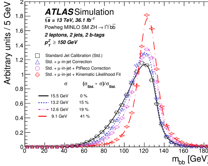
Figure 7.13: Comparison in 2-lepton channel of the m_{bb} distribution as additional energy corrections are included in the jet correction. Image source: [161].
