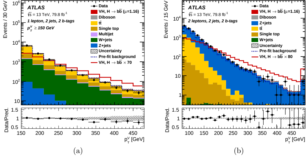
Figure 7.3: Distribution of the p_T^V for the 2-jet category of 1-lepton (a) and 2-lepton channels (b). The distributions are obtained after performing the final fit to data. The Higgs boson signal and the backgrounds are normalised with the factors extracted in the fit and shown as a filled histograms. The signal is also shown unstacked as an unfilled histogram, scaled by the factor indicated in the legend. The dashed histogram shows the total pre-fit background.
