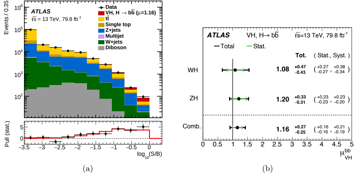
Figure 7.19: Figure (a) shows the event yields as a function of \log_{10}(S/B) for data, background and a Higgs boson signal with m_H = 125 GeV. Figure (b) shows the fitted values of the Higgs boson signal strength \mu_{VH}^{bb} for m_H = 125 GeV. The results are obtained from a simultaneous fit with the signal strength for each of the lepton channels floating independently.
