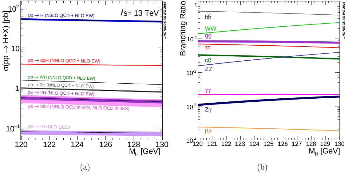
Figure 2.4: Cross sections of the Higgs production modes (a) and branching ratios of the main decay modes (b) in pp colliders as a function of the Higgs boson mass value. Image source [27].
