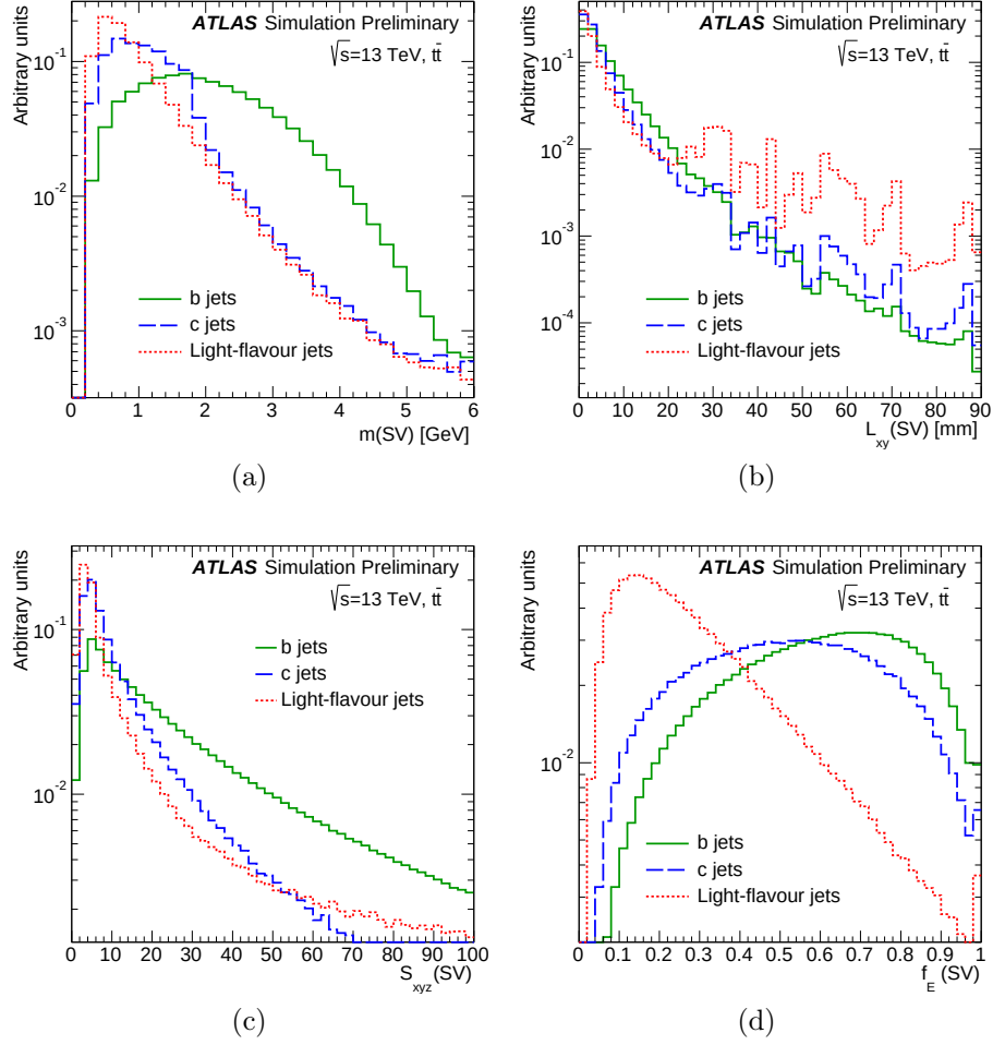
Figure 5.8: Properties of the secondary vertices reconstructed by the SV algorithm for b (solid green), c (dashed blue) and light -flavour (dotted red) jets: the invariant mass (a), the transverse decay length (b), the 3D decay length significance (c) and the energy from the tracks in the displaced vertex relative to all the tracks reconstructed within the jet (d). Image source: [123].
