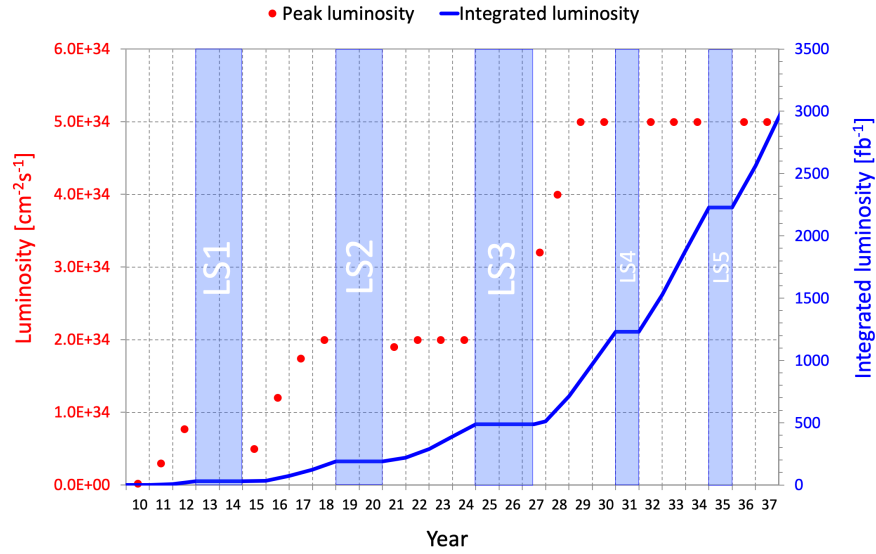
Figure 4.4: Projected LHC performance through 2037, showing preliminary dates for long shutdowns of the LHC and projected luminosities. Image source: [72].
