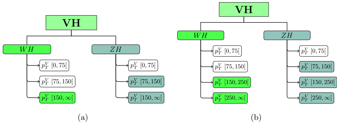
Figure 8.3: Figure (a) shows the 3-POI scheme used for the VH(H \rightarrow b\bar{b}) cross section measurements. Similarly, figure (b) shows a finer bin splitting used to perform 5-POI cross section measurements.
