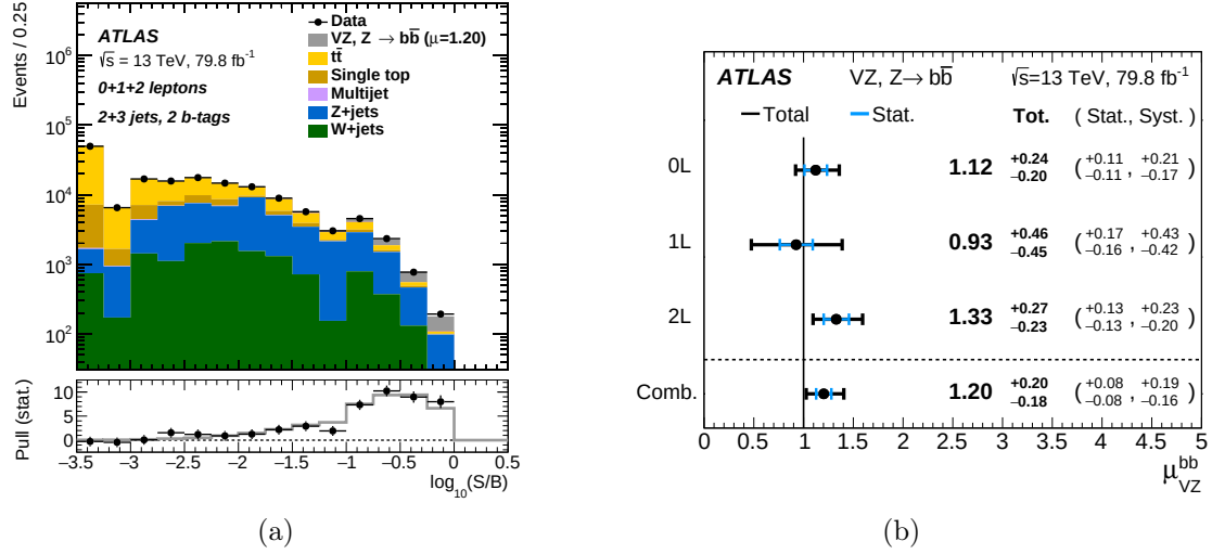
Figure 7.22: Figure (a) shows the event yields as a function of \log_{10}(S/B) for data, background and diboson ( VZ ) signal. Figure (b) shows the fitted values of the VZ signal strength for the 0-lepton, 1-lepton and 2-lepton channels. The results are obtained from a simultaneous fit with the signal strength for each of the lepton channels floating independently.
