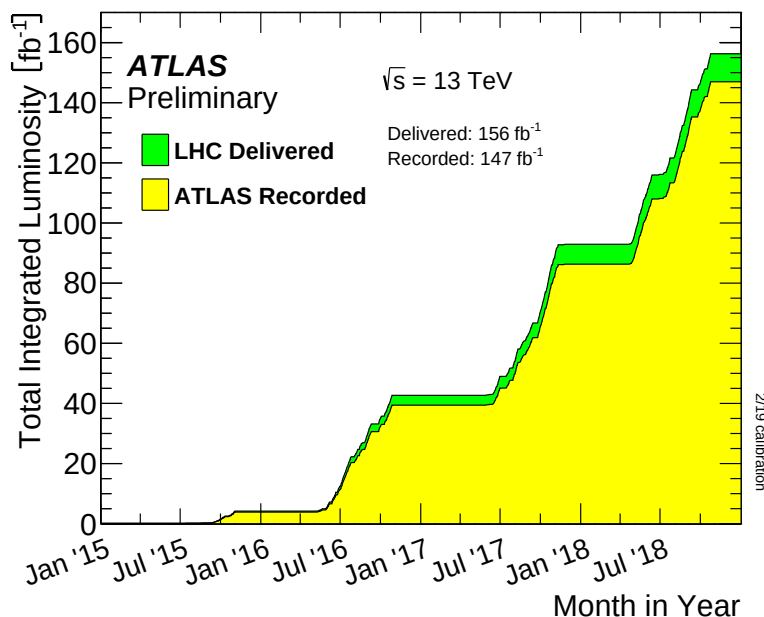
Figure 4.2: Integrated luminosity versus time delivered by the LHC (green) and collected by ATLAS (yellow) during stable beams for pp collisions at \sqrt{s} = 13 TeV in Run-2. Image source: [71].
