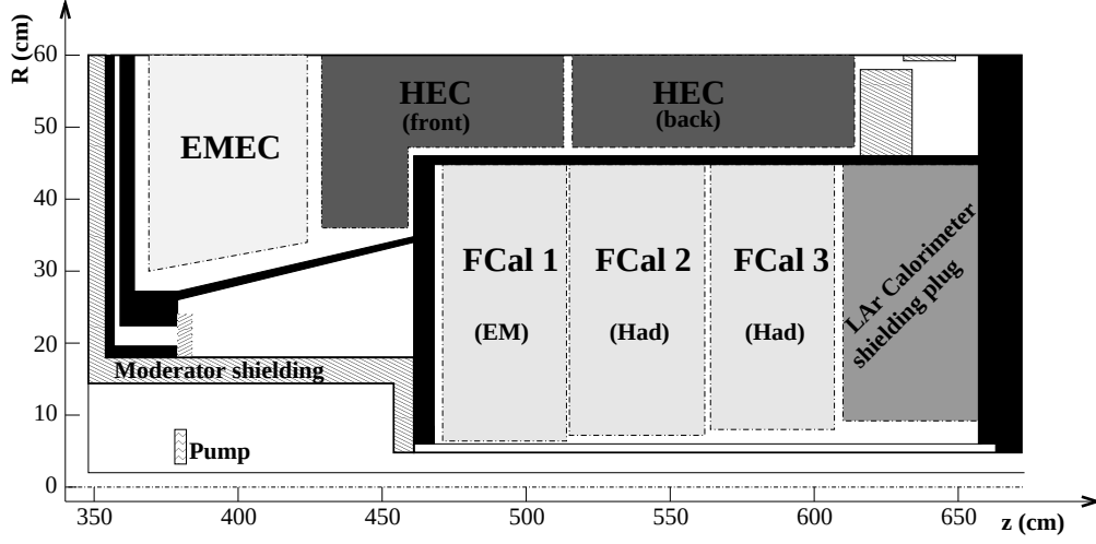
Figure 4.8: Transversal view of the ATLAS calorimeter system showing the transition from the EMEC and HEC calorimeters to the FCAL calorimeter. Image source: [87].
