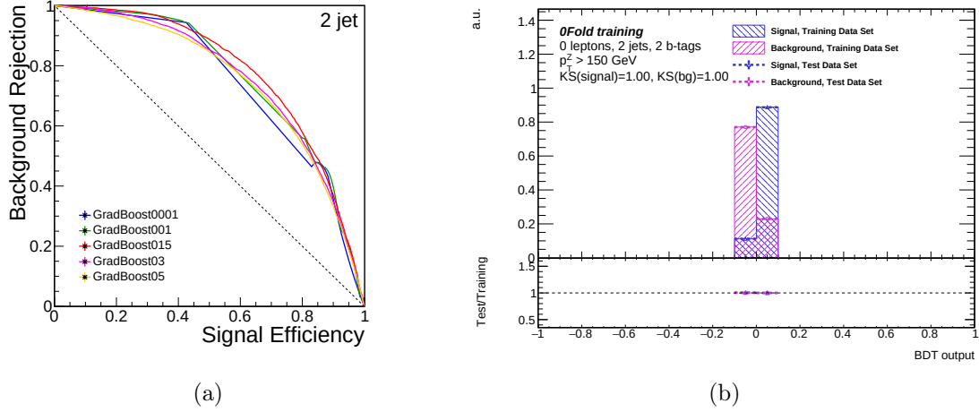
Figure 7.16: ROC comparison between different learning rates used with GradBoost, in 2-jet (a) category. In Figure (b) the BDT distribution obtained with a learning rate of 0.001 is shown.
