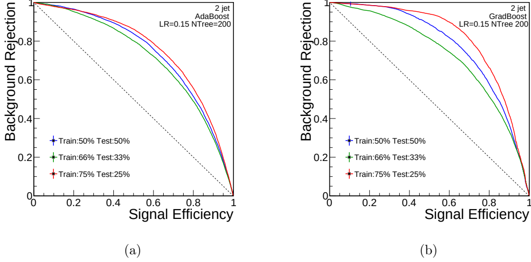
Figure 7.15: ROC comparison between different training statistics used with AdaBoost (a) and GradBoost (b). The blue curve is obtained with a 2-fold scheme, the green with 3-fold and the red curve with 4-fold . The results are shown only for the 2-jet category.
