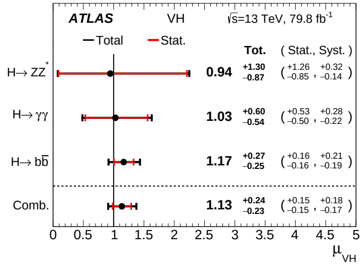
Figure 7.25: Higgs boson signal strength \mu_{VH}^{bb} for the H \rightarrow b\bar{b} , H \rightarrow ZZ^* and H \rightarrow \gamma\gamma decay modes and VH production. The displayed values are the result of a global likelihood fit where the individual signal strengths of the different decay modes are left floating.
