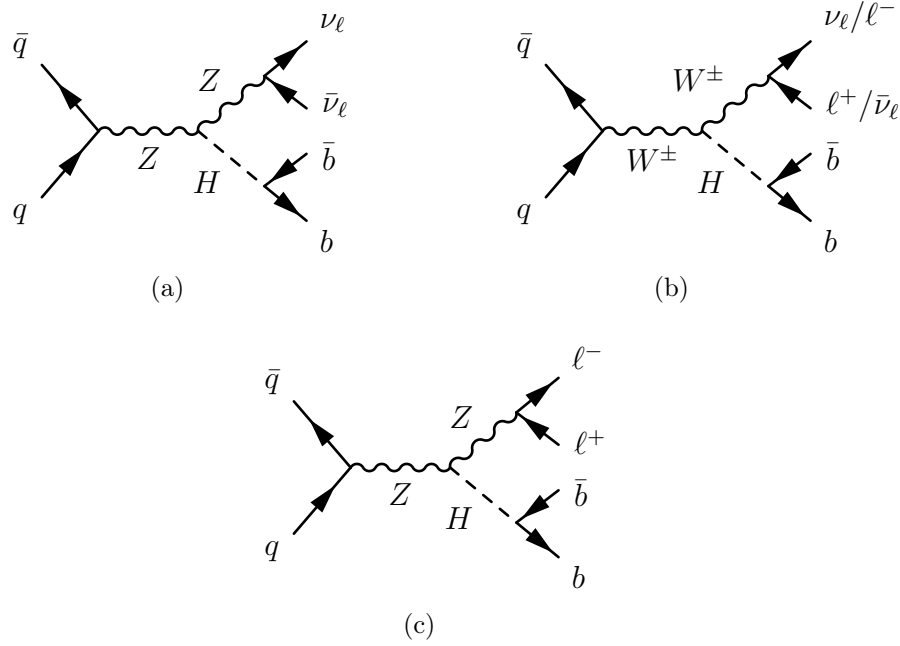
Figure 7.2: Feynman diagrams for the LO quark initiated SM VH(H \rightarrow b\bar{b}) processes, with V decaying leptonically.
