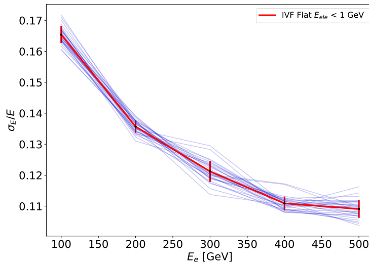
Figure 6.8: Detector resolution as a function of the energy of the initial electron. The estimation is obtained with the bootstrap method by sampling the initial dataset consisting of the output of the fast simulation.
