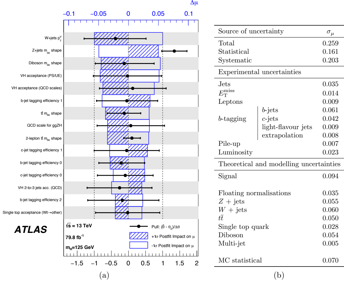
Figure 7.20: Figure (a) show the impact of the individual systematic uncertainties on the measured signal strength \mu_{VH}^{bb} . Figure (b) shows the breakdown of the uncertainty in \mu_{VH}^{bb} when the individual contributions are combined in categories.
