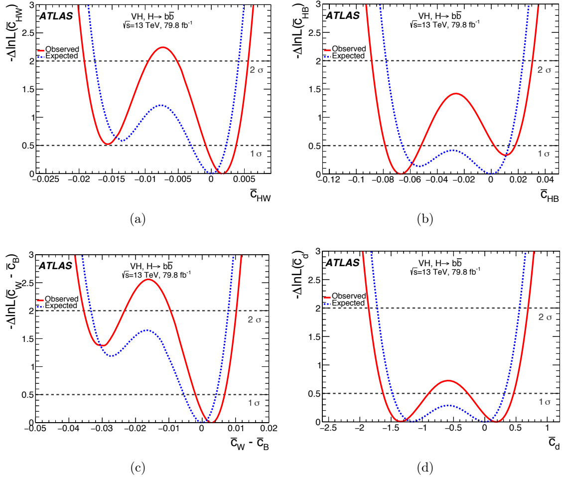
Figure 8.7: Expected (blue) and observed (red) profile likelihoods of the fitted EFT coefficients. The parametrisation used includes both linear and quadratic contributions.
