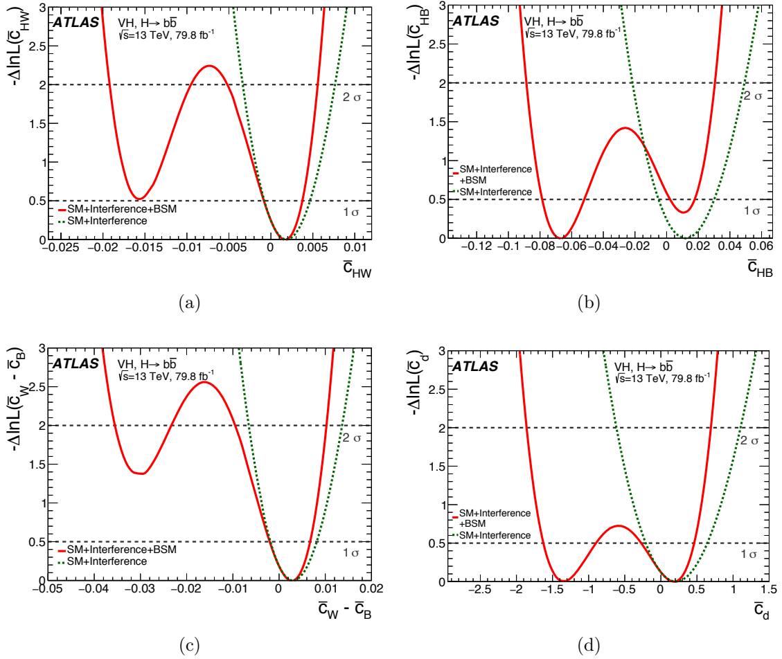
Figure 8.8: Observed profile likelihoods of the fitted EFT parameters. Comparison between the result obtained with the only linear parametrisation (green) and the result with the full (linear+quadratic) one (red).
