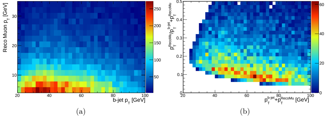
Figure 7.7: Distribution of the candidate muon p_T as a function of the b -jet p_T (a). About 10% of the jet momentum is carried by the muon (b).
