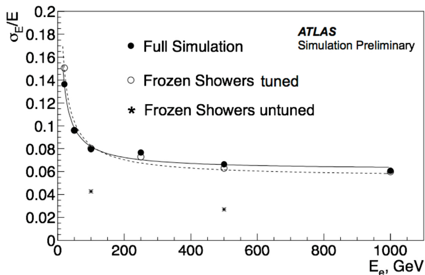
Figure 6.4: Energy resolution obtained in fast simulation using the default library (star points) compared to the result obtained with full simulation (black dots). The parameters in the library need to be tuned in order to obtain a result consistent with the full simulation. The empty circles correspond to the fast simulation response obtained with tuned library. Image source:[147].
