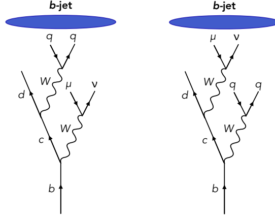
Figure 7.6: Examples of b -jet semileptonic decays at quark-level. A b -jet may contain at least one muon in \sim 21\% of cases due to the decay of virtual W bosons.
