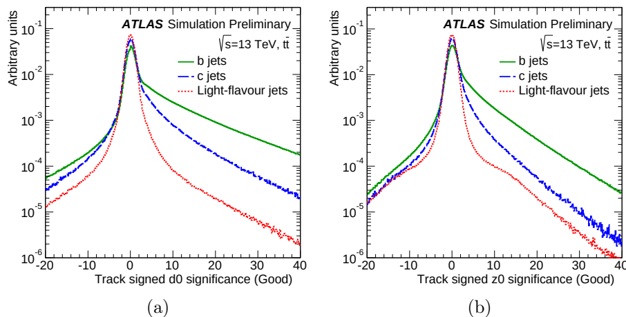
Figure 5.7: The transverse (a) and longitudinal (b) signed impact parameter significance of tracks in events associated with b (green), c (blue) and light -flavour (red) jets. Image sources: [123].
