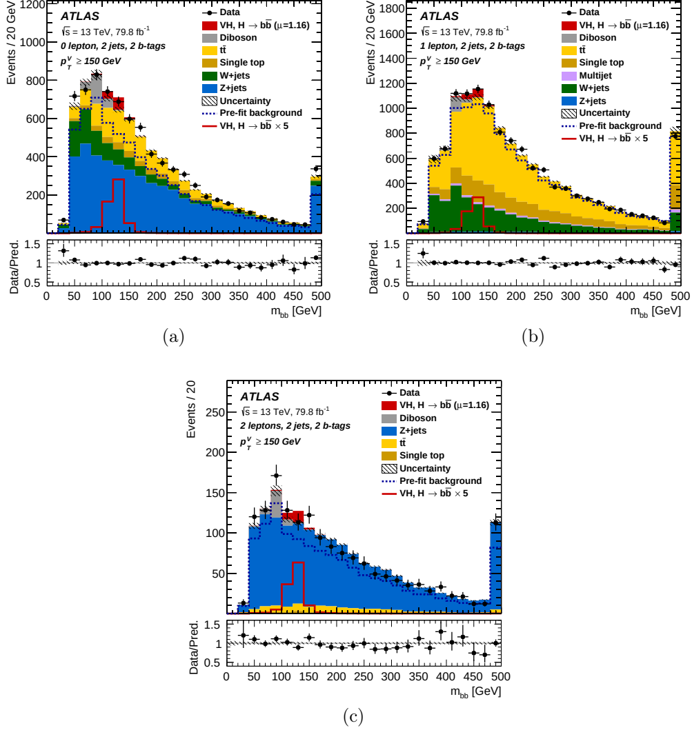
Figure 7.5: Invariant mass distribution of the two b -jets in 0-lepton (a), 1-lepton (b) and 2-lepton (c) channels. The distributions have been obtained after performing the final likelihood fit, therefore the extracted normalisation factors are applied. The dashed histogram shows the total pre-fit background. The background contributions are shown as filled histograms. Image sources: [5].
