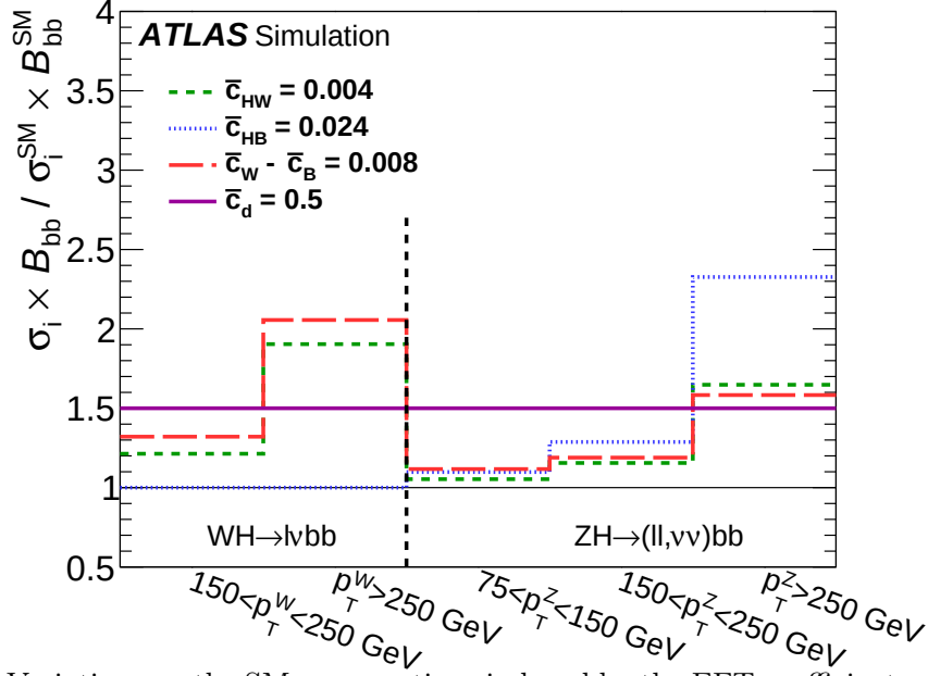
Figure 8.9: Variations on the SM cross sections induced by the EFT coefficients considered in the VH(H \rightarrow b\bar{b}) measurements.
