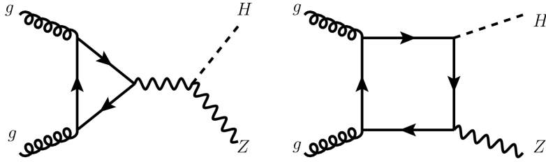
Figure 8.10: Feynman diagram topologies contributing to the gg \rightarrow ZH production.
