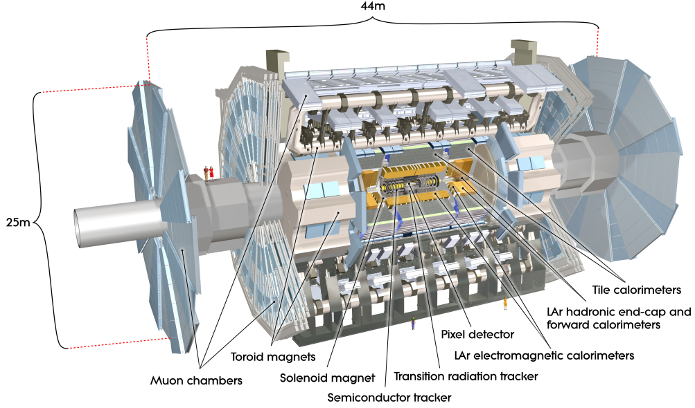
Figure 4.5: The ATLAS detector. The main sub-systems are indicated. Image source: [73].
