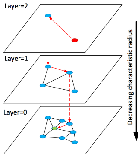
Figure 3.5: Illustration of an HNSW structure composed by three layers. Image source: [64].
