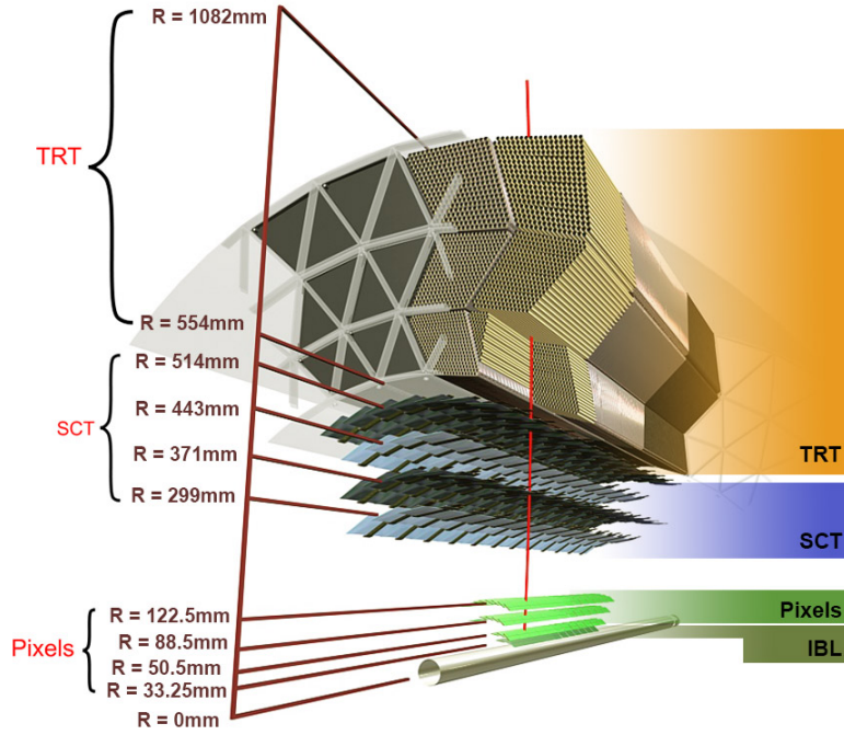
Figure 4.6: Cut-away view of the ATLAS inner detector. Image source: [76].
