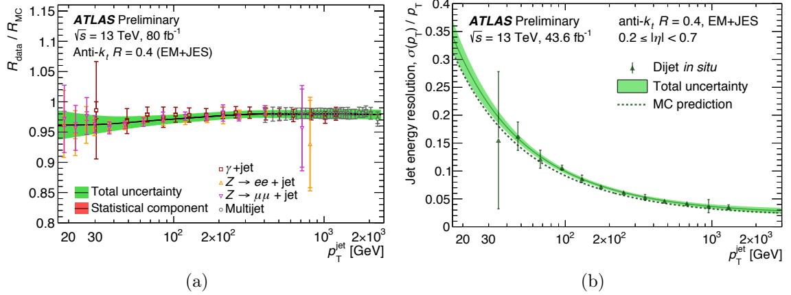
Figure 5.4: Data-to-MC ratio of the average jet p_T response as a function of jet p_T . The combined result is based on three in-situ techniques: the Z +jet balance method, \gamma +jet balance method and the multijet balance (a). The relative JER \sigma_{p_T}/p_T as a function of p_T . The results are obtained for anti- k_t jets with a radius parameter of R = 0.4 , calibrated following the JES scheme, including the residual in-situ calibration and using the 2017 dataset (b). Image sources: [116, 117].
