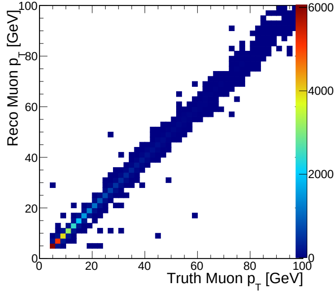
Figure 7.9: Transverse momentum of the reconstructed muon candidates versus the momentum of the matched truth muons that are originated from a b -hadron.
