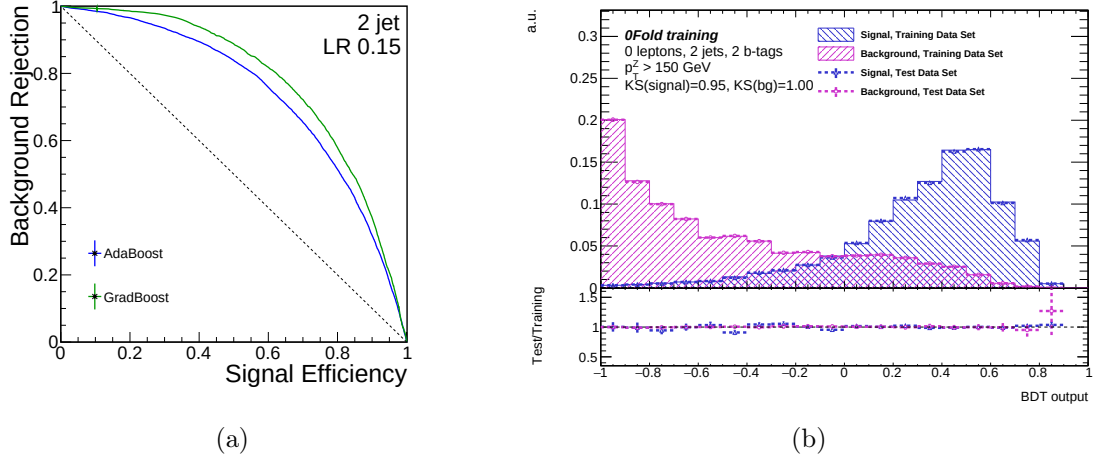
Figure 7.14: ROC comparison between AdaBoost and GradBoost performances in 2-jet (a) and distribution of the BDT discriminant obtained with the GradBoost algorithm (b). The learning rate is fixed at the default value ( \text{LR} = 0.15 ), as well as the other parameters.
