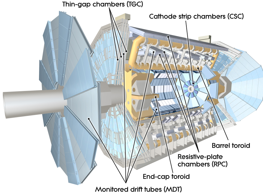
Figure 4.10: Cut-away view of the ATLAS muon spectrometer. Image source: [90].
