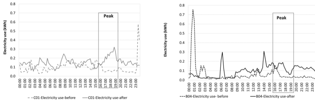
Figure 10. Daily average electricity use profiles in C01(left) and B04 (right) before and after heat pump
