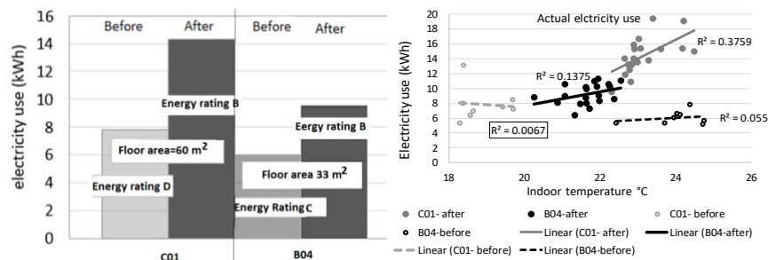
Figure 11: Daily average electricity use (kWh) in C01 and B04 before and after heat pump installation in relation to type of dwelling, energy rating and floor area (left), and scatter plot of mean indoor temperature and daily electricity use (kWh) in C01 and B04 before and after heat pump installation (right)
