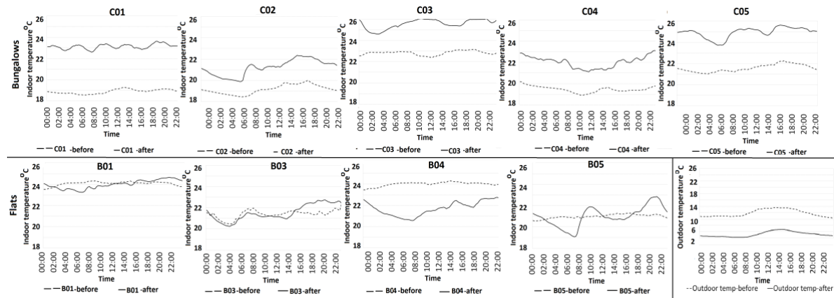
Figure 5. Daily mean temperature profiles in bungalows (top) and flats (down) before and after heat pump
