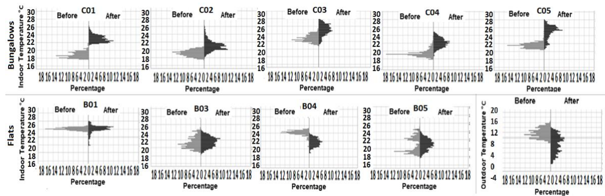
Figure 4. Distribution of indoor temperature in bungalows (top) and flats (down) before and after heat pump
