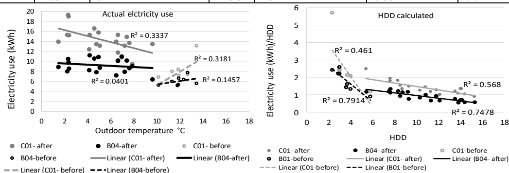
Figure 9. Correlation between total electricity use (kWh) and mean outdoor temperature (left) and normalised electricity use (kWh)/HDD and HDD (right)
