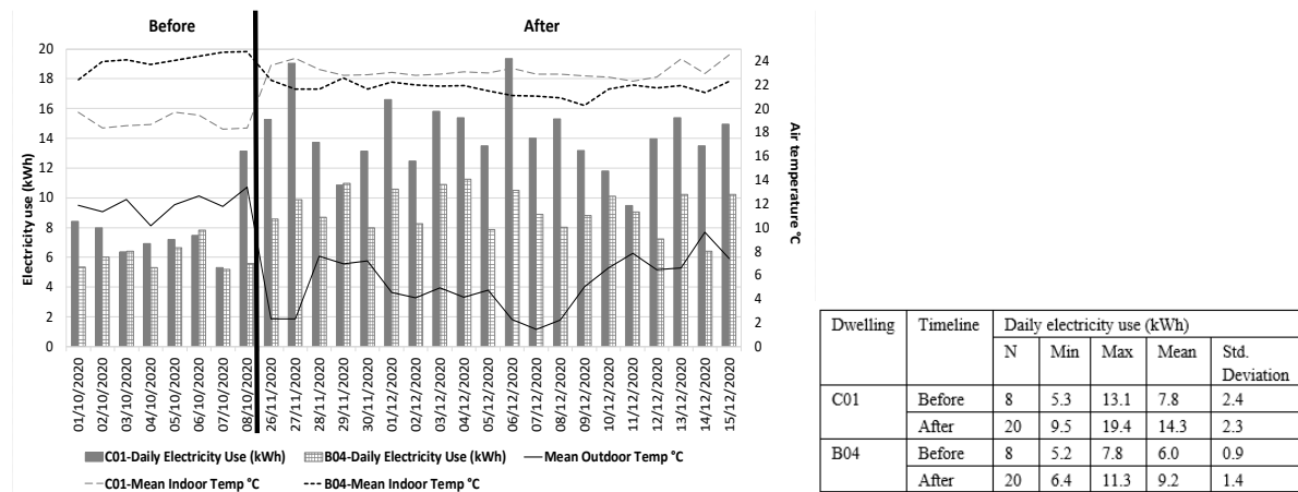
Figure 8. Daily electricity use (kWh) and daily average indoor and outdoor temperature profiles in C01 and B04 before and after heat pump installation (left), and descriptive statistics analysis for daily electricity use (right)
