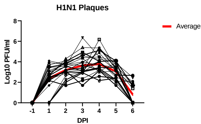
Suppl. Figure 2. Experimental design and pH1N1 viral load for the efficacy study. Twenty-four pigs were infected with pH1N1 Influenza A virus, four weeks later immunized with ChAdOx-NPM1-NA2 intramuscularly (IM), intranasally (IN) or by aerosol (AE) and four weeks later boosted with MVA-NPM1-NA2. After four weeks all pigs were challenged with H3N2 and four days later culled. Control (C) animals were infected but not immunized. Weekly blood samples were collected (a) . pH1N1 virus load was determined by plaque assay of daily nasal swabs at the indicated days post infection (DPI) following pH1N1 inoculation on D0 (b) .
