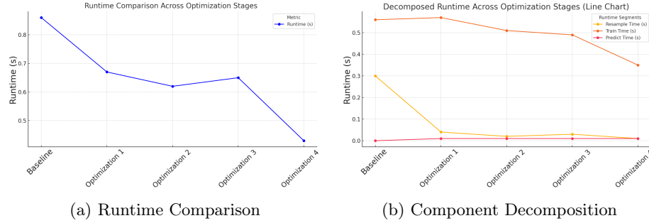
Fig. 2: (a) Runtime Comparison and (b) Components Decomposition
