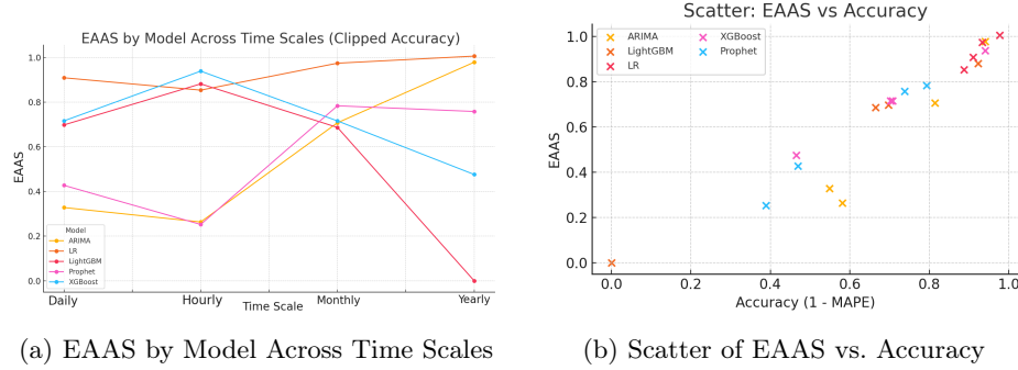
Fig. 1: EAAS performance: (a) Across time scales (b) Relative to accuracy.
