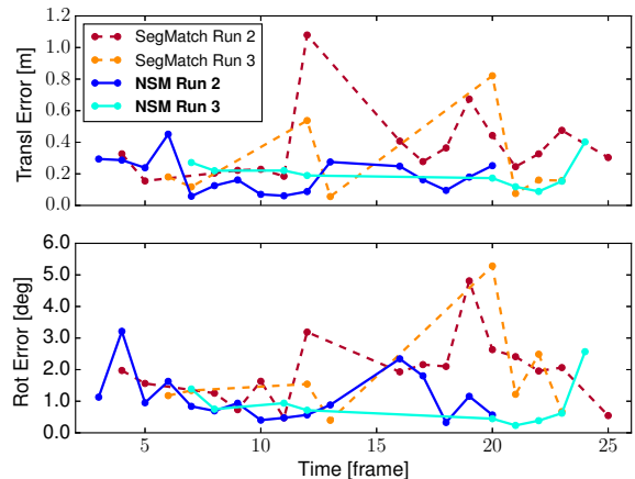
Fig. 8: Translation (top) and rotation (bottom) errors for the proposed approach (continuous lines) and the baseline algorithm (dashed lines) tested on the GS dataset from two sequential runs. Run 1 was used to create the map.
