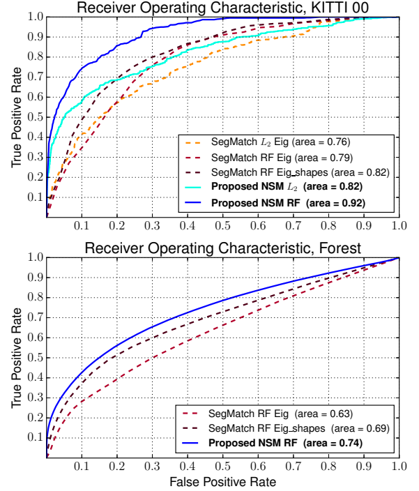
Fig. 6: Receiver Operator Characteristic curves for NSM and SegMatch [2] evaluated on Seq 00 of the KITTI dataset (top) and a forest dataset, similar to GS (bottom). The proposed approach was evaluated with both k-NN in feature space ( L_2 , cyan) and a pre-trained Random Forest (RF) classifiers (blue). The baseline was evaluated with Eigenvalue-based (Eig) features and Eigenvalue with ESH (Fig. 6) features.
