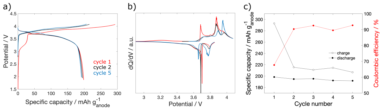
Figure 6: KMF | KFSI in Pyr 1,3 FSI | graphite full cell cycling results. (a) and (b) the first, second and fifth galvanostatic profiles and differential capacity plots for the full cell cycled at C/10. (c) Specific capacity and coulombic efficiency of the full cell. The mass ratio of KMF:graphite was 3.6:1.
