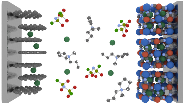
Figure 1: A schematic of the full-cell potassium-ion chemistry consisting of a graphite anode, potassium bis(fluorosulfonyl)imide in N-butyl-N-methylpyrrolidinium bis(fluorosulfonyl)imide electrolyte, and potassium manganese hexacyanoferrate cathode.
