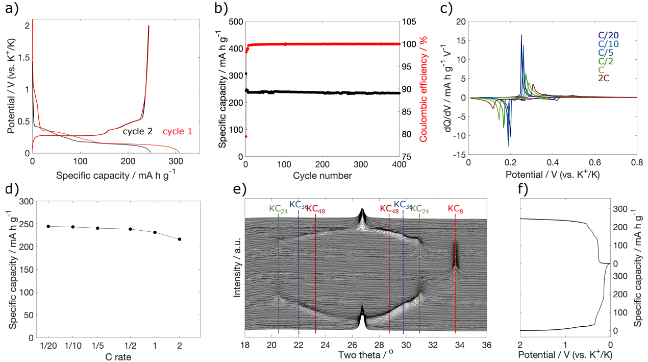
Figure 5: Galvanostatic cycling results for the graphite anode. (a) First and second cycle galvanostatic profiles of graphite. (b) Capacity retention and coulombic efficiency for 400 cycles (cycles 1-5 at C/20, 6-400 at C/5). (c) and (d) differential capacity and capacity retention of graphite at C rates from C/20 to 2C. (e) and (f) Operando X-ray diffraction patterns, and relative potential versus capacity profiles for the potassium intercalation and de-intercalation into graphite at C/30. The major peaks for the intermediates KC 48 , KC 36 , KC 24 and KC 8 are highlighted.
