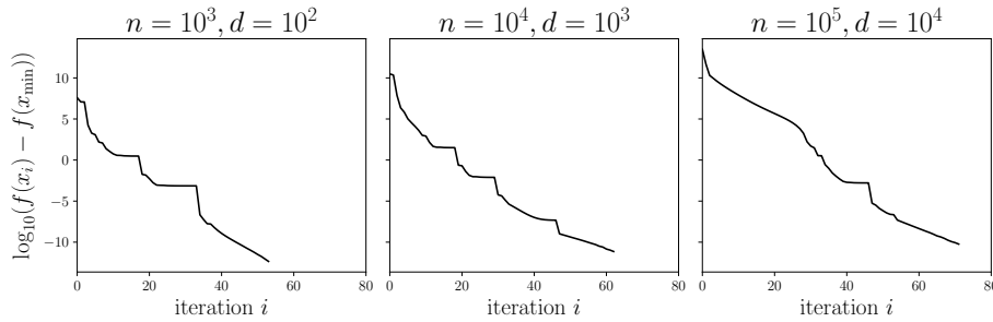
FIG. 1. Convergence rates for p -norm regression are mostly unaffected by the dimension d for these random instances with p = 4 .
