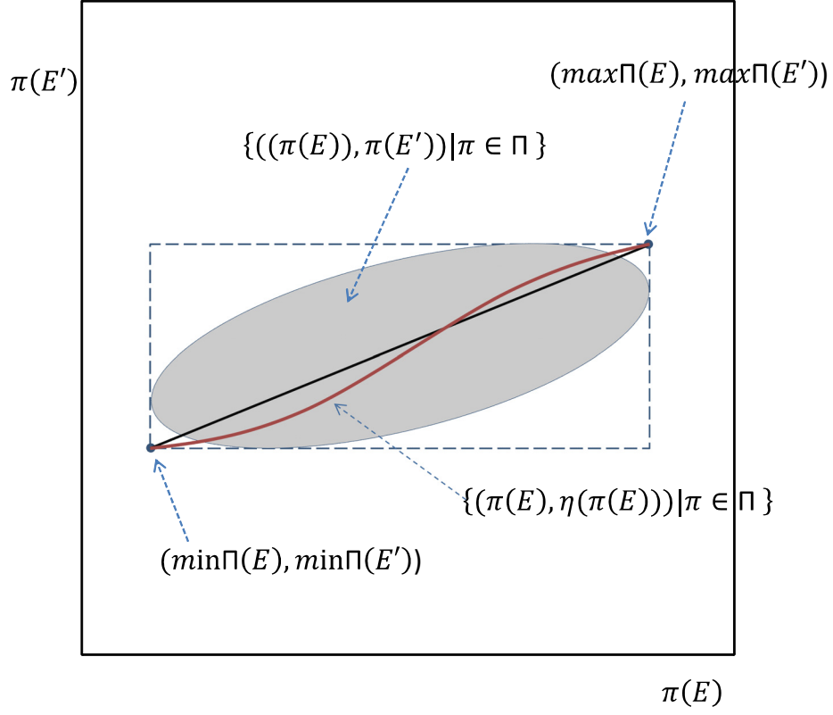
Figure 1: Illustration of E m.a.(II) event than E' for \alpha -MEU and smooth ambiguity.
