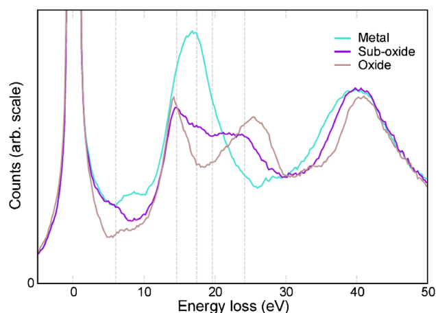
Fig. 3. Experimental low-loss EELS spectra from the metal, sub-oxide, and oxide.
