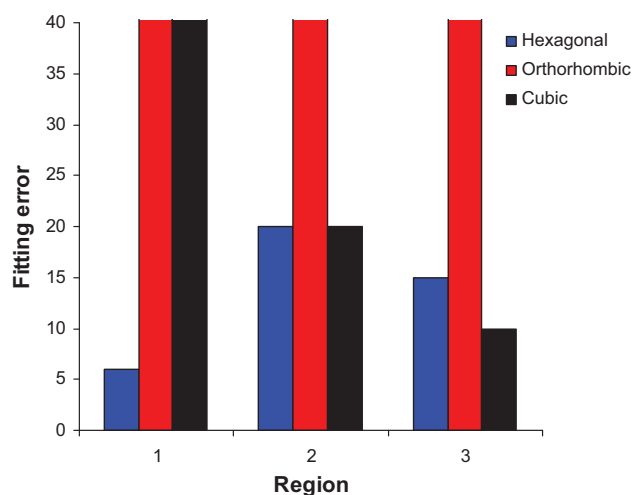
Fig. 2. Fitting error of simulated diffraction data from each of the three different structures with experimental data from three different interface regions.
