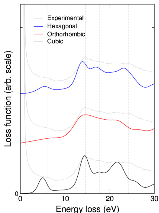
Fig. 4. Comparison of simulated EELS spectra from each of the three candidate ZrO structures with experimental data.
