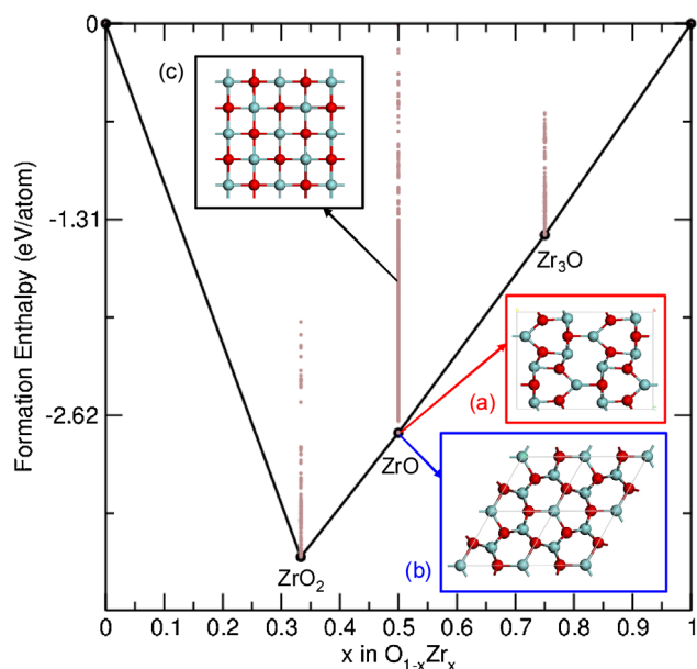
Fig. 1. Convex hull of the O_{1-x}Zr_x system. The two stable forms of ZrO are shown; the orthorhombic structure (a) has Cmcm symmetry ( a = 3.24 \text{ \AA} , b = 12.21 \text{ \AA} , and c = 8.59 \text{ \AA} ) and the hexagonal structure (b) has P-62m symmetry ( a = 5.31 \text{ \AA} and c = 3.20 \text{ \AA} ). The experimentally reported cubic rock salt structure (c) is also shown ( a = 4.62 \text{ \AA} ). Oxygen atoms are shown in red.
