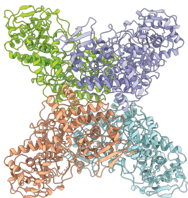
Catalase-Peroxidase (320 kDa)
