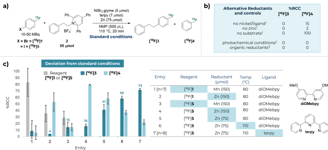
Scheme 1. Optimisation and control reactions of aryl (C) sp 2 -(C) sp 3 cross-coupling of primary alkyl 2,4,6-triphenylpyridinium tetrafluoroborate 2 with [ 18 F]-halo-4-fluoroarenes [ 18 F] 1 and [ 18 F] 5 . a ) Standard Conditions. b ) Alternative reductants and controls. c ) Optimisation reactions with deviations from standard conditions (Scheme 1a).
