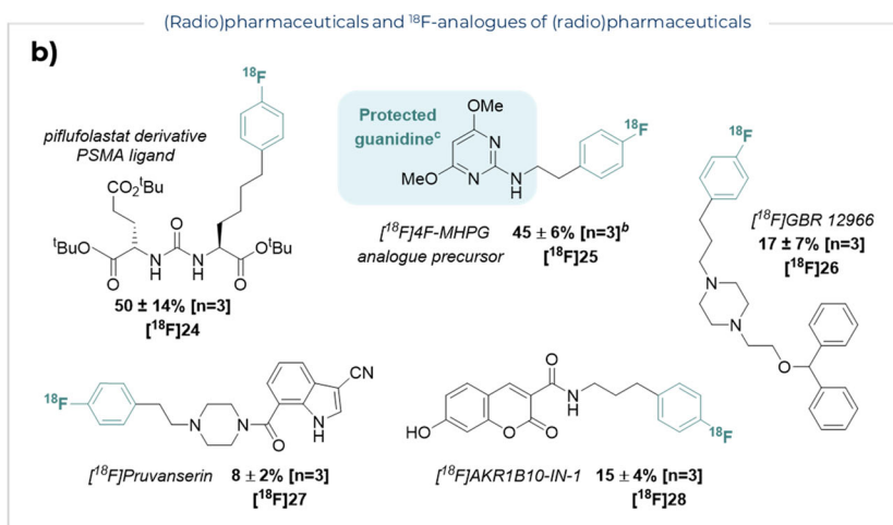
Scheme 2. Alkyl coupling partner scope.
