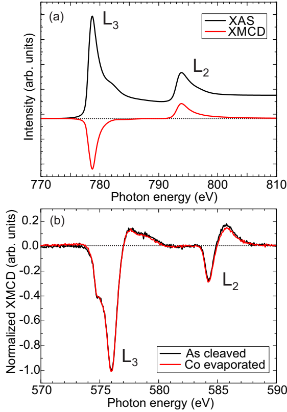
FIG. 2. (Color online) (a) Co L_{2,3} XAS and XMCD for the thin layer of Co, grown on top of the cleaved Cr:Bi 2 Se 3 thin film, measured in TEY at 10 K in a 0.5 T field. The clean, metallic line shapes indicates that no significant intermixing or alloying has taken place. (b) Normalized Cr L_{2,3} XMCD at 10 K in an 8 T field taken before (black curve) and after (red curve) deposition of the Co layer, scaled to matching peak heights at L_3 . It can be seen that the character of the Cr dopants is not affected by the addition of the ferromagnetic overlayer, only the magnetic ordering temperature is enhanced.
