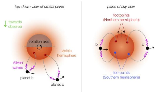
Figure 8. Sketch of the scenario where regions of enhanced emission are induced on the stellar surface of AU Mic via a sub-Alfvénic interaction between the star’s magnetic field and the orbiting planets. In a sub-Alfvénic orbit, a planet can produce Alfvén waves that carry energy back towards the stellar surface along the field line connecting to the planet. If the point where the field line connects to the stellar surface (foot point) appears on the hemisphere visible to the observer (left), enhanced chromospheric emission may appear. As planets b and c both orbit in the closed-field region of the star’s magnetic field (see Kavanagh et al. 2021), they may each produce up to two visible foot points on the stellar disc (right).
