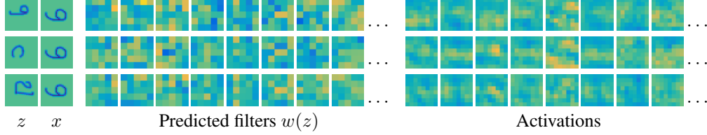
Figure 3: The predicted filters and the output of a dynamic convolutional layer in a single-stream learnnet trained for the OCR task. Different exemplars z define different filters w(z) . Applying the filters of each exemplar to the same input x yields different responses (although in typical operation, the network defined by a single exemplar is applied to many other inputs). Best viewed in colour.
