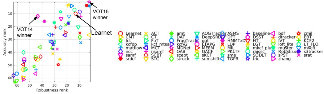
Figure 5: Accuracy-Robustness ranking plot (as produced by the VOT toolkit) for all the 62 trackers that participated to the VOT 2015 [10] challenge. Note that these rankings are produced based on a statistical method described in [10], and being relative rankings they are not comparable across papers; for this reason we supply the raw (absolute) metrics in the main paper. We use the variant B+A of our proposed (siamese) learnet. Best trackers are closer to the top right corner of the plot. Despite being only a proof-of-concept without online update of the model nor temporal constraints, our method is among the best. We remark that the top-ranking tracker, MDNet [15], fine-tunes a network with SGD during tracking, which is computationally expensive (1 frame per second on a GPU), while all our networks operate in feed-forward mode during tracking and run at at least 60 FPS. Moreover, MDNet is trained on videos from other benchmarks that are very similar to the ones of the test set, practice which has since been prohibited by the VOT committee.
