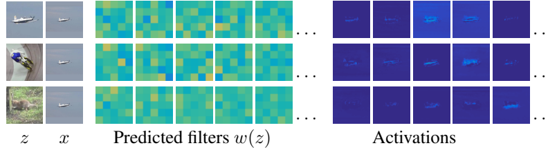
Figure 4: The predicted filters and the output of a dynamic convolutional layer in a siamese learnnet trained for the object tracking task. Best viewed in colour.
