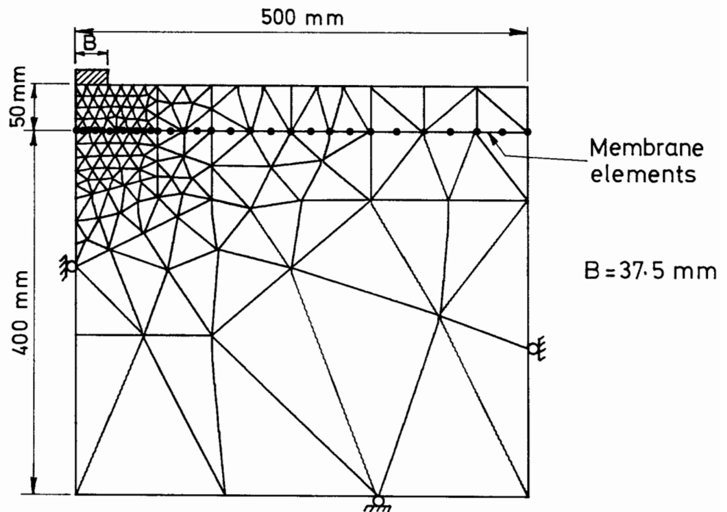
Figure 7.7: Mesh A
