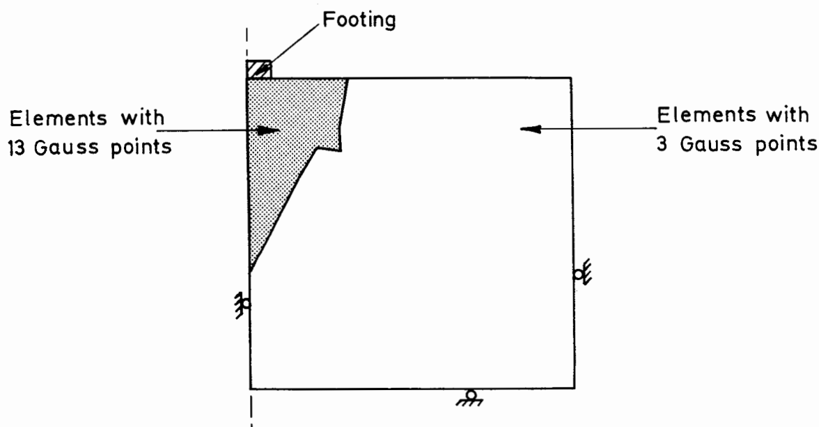
Figure 7.4: Element Gauss Points for Subgrade-Only Calculations
