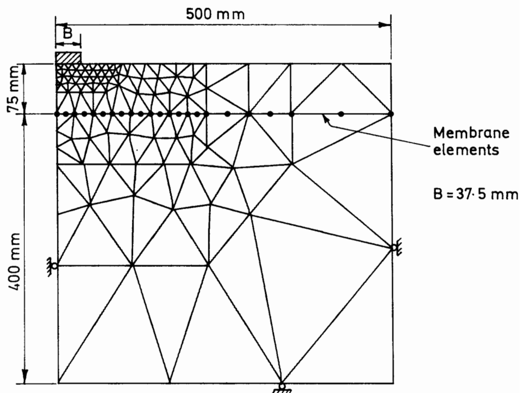
Figure 7.3: Mesh B
