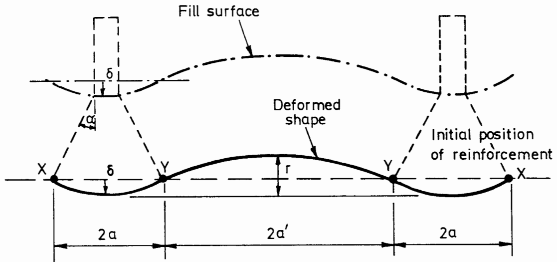
Figure 9.2: Idealised Deformations
