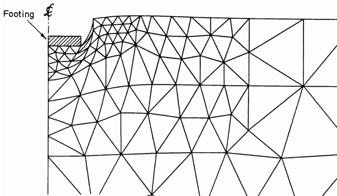
Figure 7.6: Deformed Mesh at End of Calculation S3
