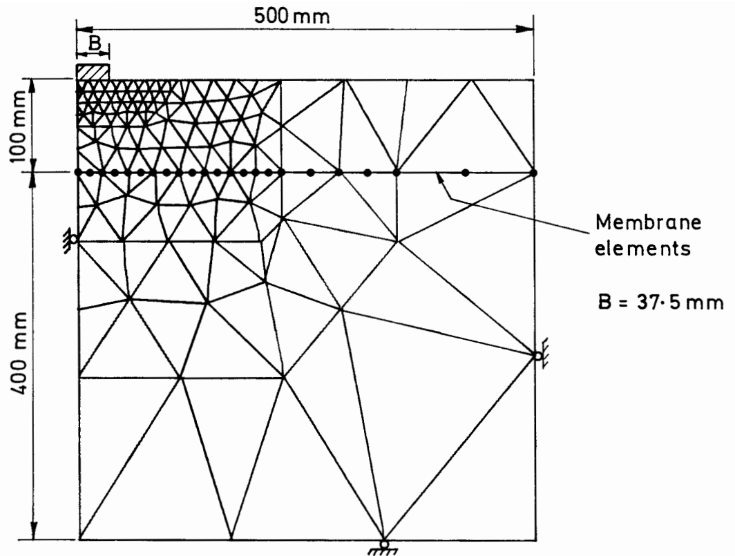
Figure 7.8: Mesh C
