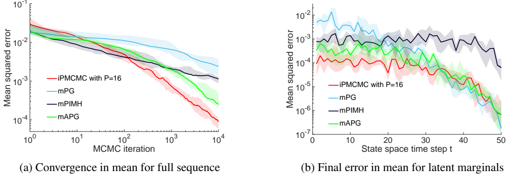
Figure 2. Mean squared error averaged over all dimensions and steps in the state sequence as a function of MCMC iterations (left) and mean squared error after 10^4 iterations averaged over dimensions as function of position in the state sequence (right) for (12) with 50 time sequences. The solid line shows the median error across the 10 tested synthetic datasets, while the shading shows the upper and lower quartiles. Ground truth was calculated using the Rauch–Tung–Striebel smoother algorithm (Rauch et al., 1965).
