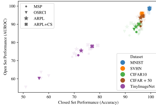
Figure 6: Correlation between open-set and closed-set performances on the standard OSR benchmarks. This plot is similar to fig. 2 but includes scatter points for OSRCI (Neal et al., 2018).
