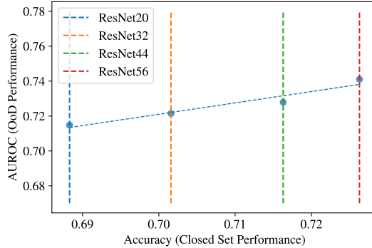
Figure 8: OoD against closed-set performance for four ResNet models trained on CIFAR100, using CIFAR10 as OoD. The plot indicates a similar performance correlation as observed in fig. 3b.
