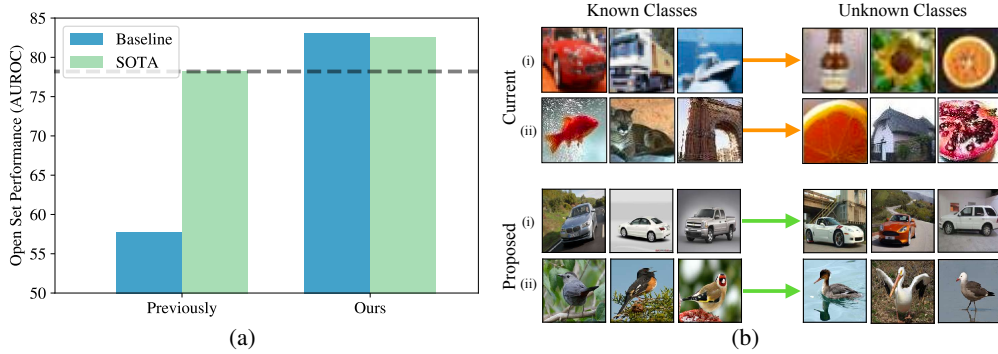
Figure 1: (a) We show that we can push OSR baseline performance to be competitive with or surpass state-of-the-art methods (shown, ARPL + CS (Chen et al., 2021)). (b) We propose the ‘Semantic Shift Benchmark’ datasets for OSR, which are larger scale and give precise definitions of what constitutes a ‘new class’.
