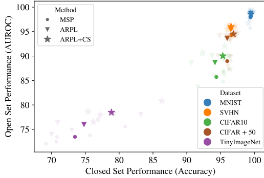
Figure 2: Correlation between closed-set performance (Accuracy) and open-set performance (AUROC). We train three methods on the standard open-set benchmark datasets, including the MSP baseline, ARPL and ARPL + CS (Chen et al., 2021). Foreground points in bold show results averaged across five ‘known/unknown’ class splits for each method-dataset pair (following standard practise in the OSR literature) while background points, shown faint, indicate results from the underlying individual splits.
