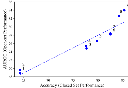
Figure 4: Gains in open-set performance as closed-set performance increases on TinyImageNet.
