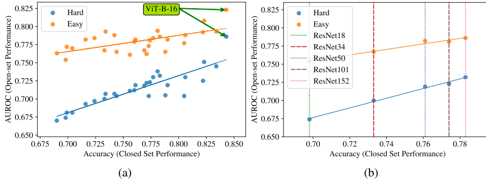
Figure 3: (a) Open-set results on a range of architectures on the ImageNet dataset. ‘Easy’ and ‘Hard’ OSR splits are constructed from the ImageNet-21K-P dataset. (b) ImageNet open-set results within a single model family (ResNet).
