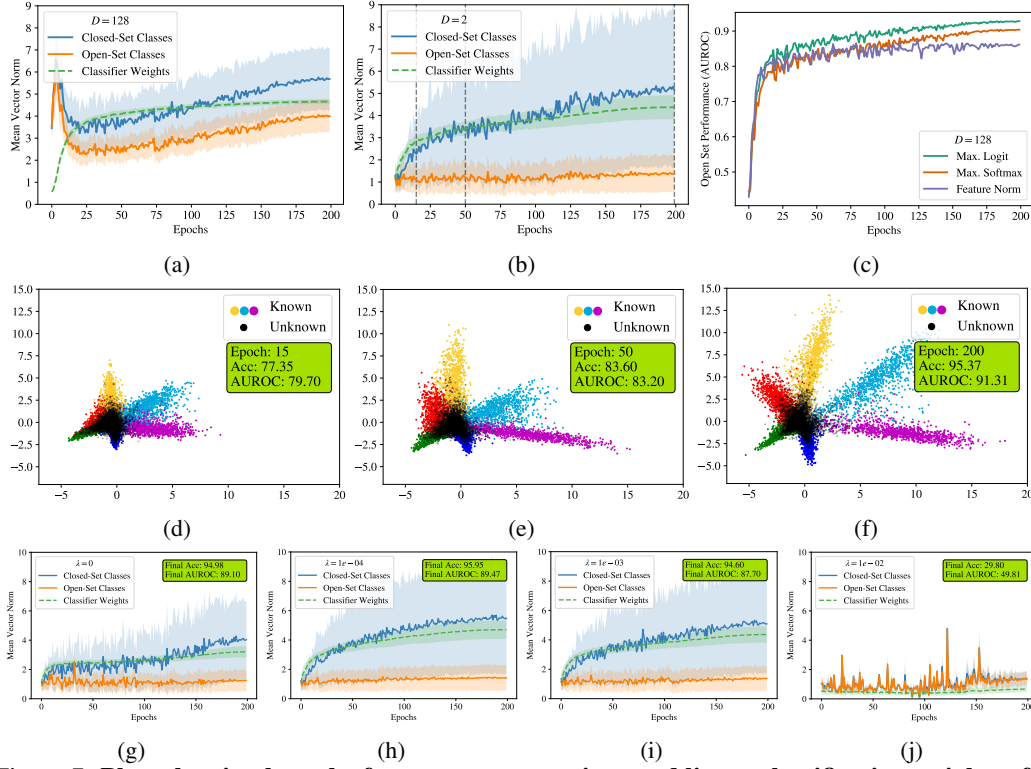
Figure 7: Plots showing how the feature representations and linear classification weights of a deep classifier evolve as training proceeds (CIFAR10 OSR setting). (a), (b) show the average feature norm for seen and unseen classes, as well as the per-class vector norms for the weights in the linear classification head, for models with D = 128 and D = 2 respectively. (c) shows how the open-set performance of the classifier with D = 128 develops as training proceeds, using three different OSR scoring rules. (d), (e), (f) show the feature projections for images from seen and unseen classes at different epochs (indicated by vertical dashed lines in (b)) for the model with D = 2 . We show test images from known classes in colour and unknown classes in black. (g) (h) (i) show how classifier weight and feature norms change as a function of weight decay strength ( \lambda )
