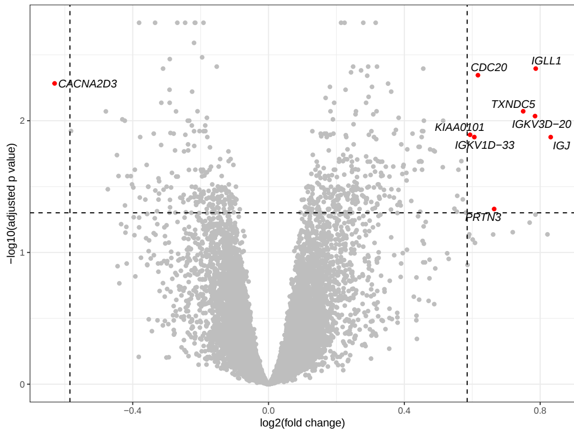
Figure 5.7: Volcano plot showing differentially expressed probes between EBV-positive and EBV-negative GAINs patients with sepsis due to CAP. Probes in red (labelled) are differentially expressed at a fold-change of \geq 1.5 and p-value of < 0.05 . Positive fold change corresponds to upregulation in Epstein-Barr virus-positive individuals.
