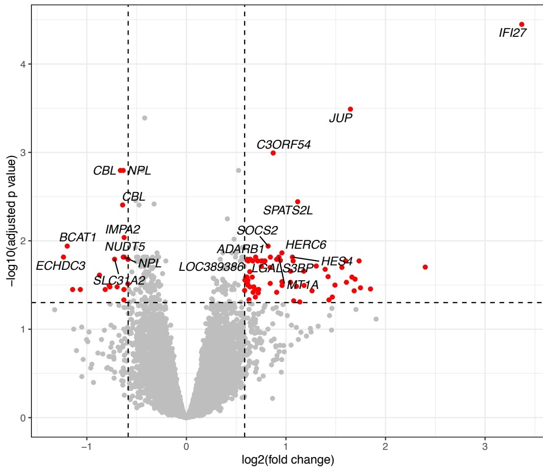
Figure 5.19: Volcano plot of differentially expressed probes in influenza vs bacterial infection for GAINs patients with sepsis due to CAP. Probes in red are differentially expressed at a FDR < 0.05 and fold change \geq 1.5 . Positive fold change corresponds to upregulation in influenza-positive individuals. Top 20 significantly differentially expressed probes are labelled.
