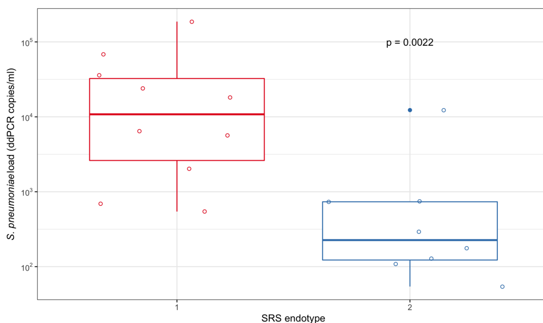
Figure 5.9: Boxplot of Streptococcus pneumoniae load and SRS status in GAINs patients with sepsis due to CAP. Bacterial load is assessed by ddPCR and SRS status is determined from genome-wide gene expression analysis of peripheral blood leukocytes by microarray. The highest bacterial load over the first five days of ICU admission is plotted against the SRS endotype from the first available timepoint after ICU admission.
