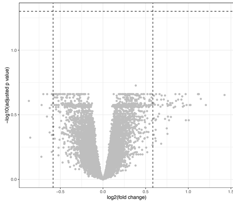
Figure 5.23: Volcano plot of differentially expressed probes in S. pneumoniae vs non- S. pneumoniae infection for GAINs patients with sepsis due to CAP. There were no differentially expressed probes at an FDR <0.05 and fold change \geq 1.5 .
