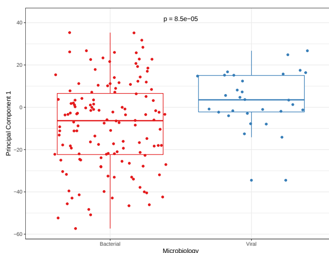
Figure 5.10: Boxplot of SRS at the first available timepoint after ICU admission as a continuous trait against microbiology in GAIN patients with sepsis due to CAP. SRS endotype is determined from genome-wide gene expression analysis of peripheral blood leukocytes by microarray. The values for principal component 1 (PC1) are derived from PCA of the top 10% most variable genes and provide a continuous measure of SRS endotype with higher values representing an SRS2 endotype and lower values representing an SRS1 endotype.
