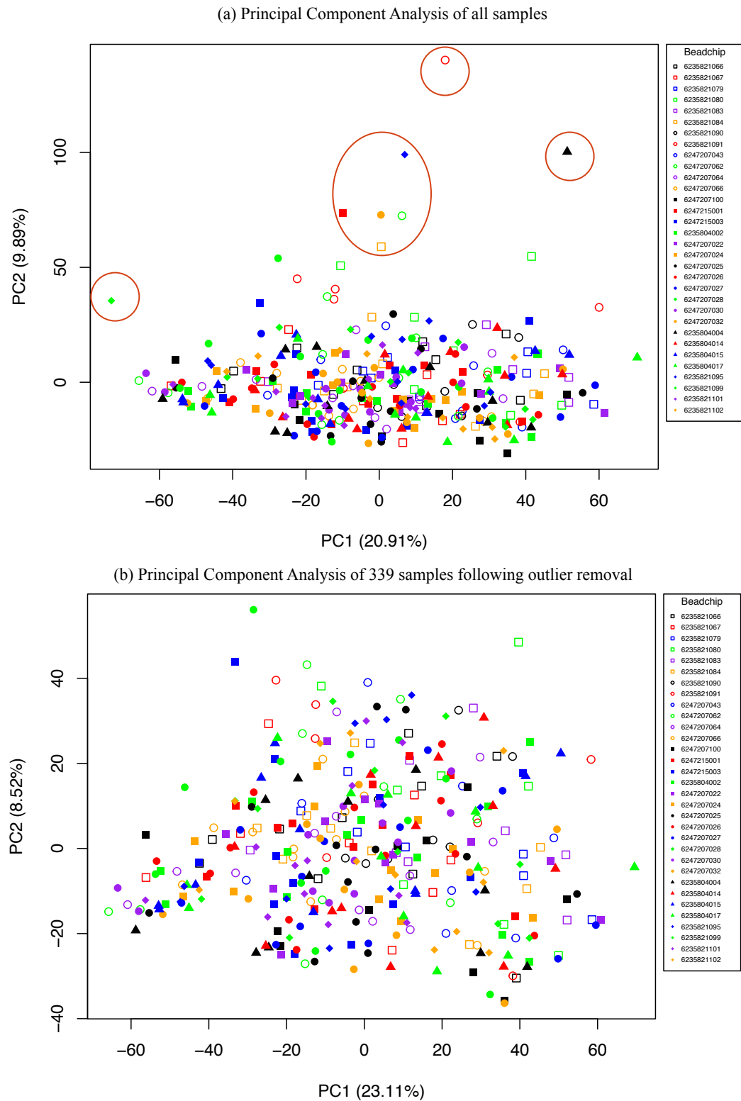
Figure 5.2: Principal Component Analysis: Davenport 2011. The first two principal components of the gene expression data are plotted, with the amount of variance explained by each noted; (a) when all samples are included in the analysis, and (b) after the removal of eight outliers. Samples are coloured according to beadchip and outlying samples are circled in red.
