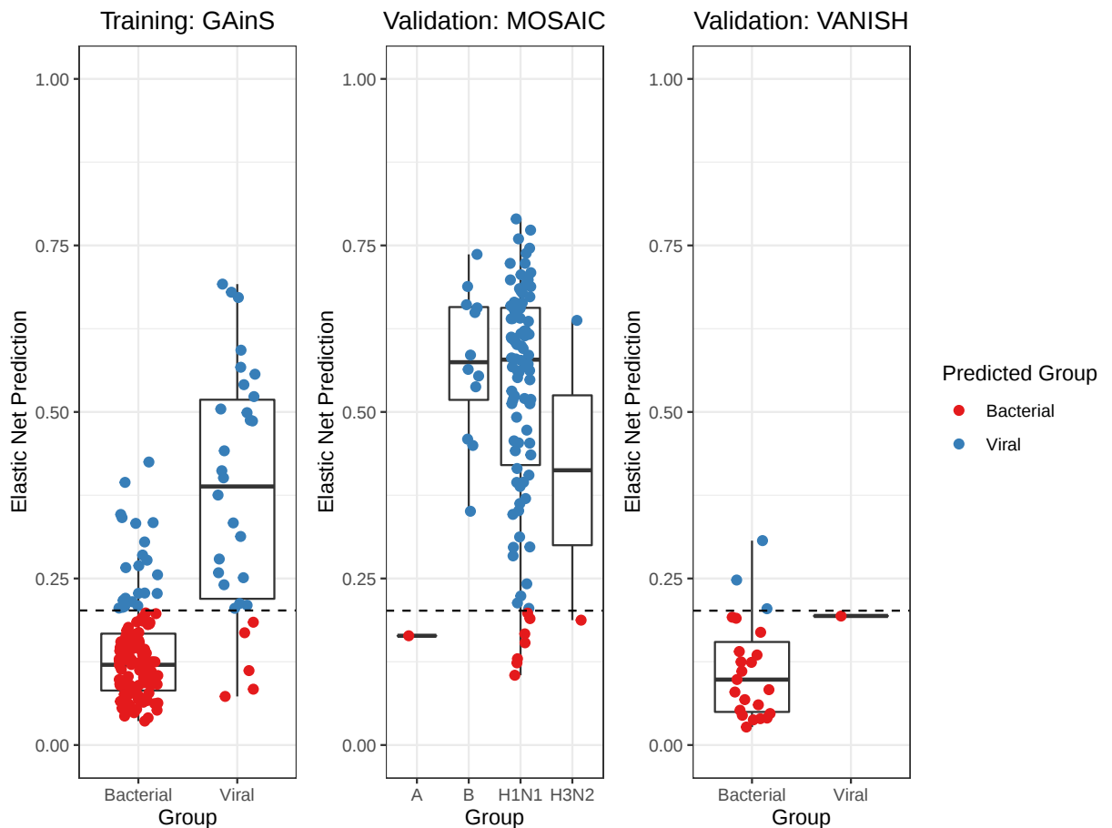
Figure 5.14: Boxplot of predictions from viral vs bacterial infection gene signature in GAinS patients with sepsis due to CAP. Each point corresponds to a patient. Actual microbiological groups are plotted on the x-axis whilst predicted classifications are denoted by point colour. The MOSAIC groupings correspond to influenza virus types. Threshold for discriminating bacterial from viral infection is denoted by the dashed line. The elastic net prediction value (y-axis) can range from 0 (indicating bacterial infection) to 1 (indicating viral infection).
