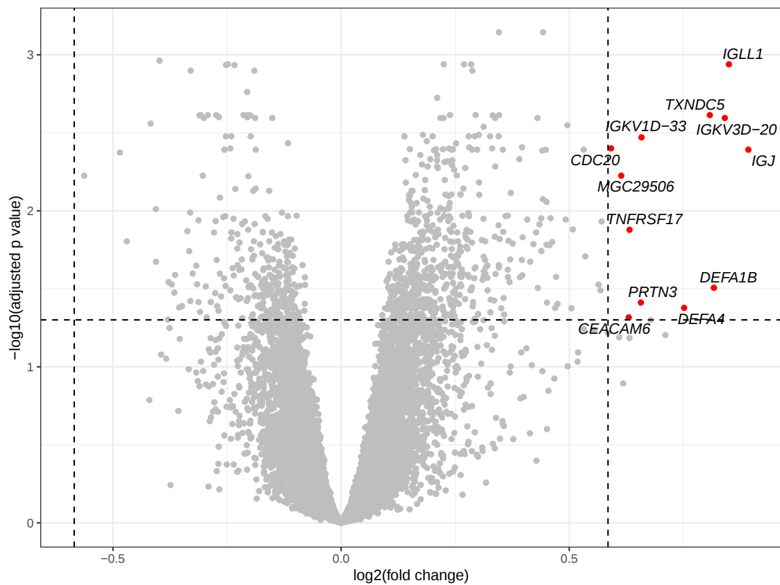
Figure 5.8: Volcano plot showing differentially expressed probes between EBV-positive and EBV-negative GAINs patients with sepsis due to CAP, with SRS endotype included in the linear model. Probes in red (labelled) are differentially expressed at a fold-change of \geq 1.5 and p-value of < 0.05 . Positive fold change corresponds to upregulation in Epstein-Barr virus-positive individuals.
