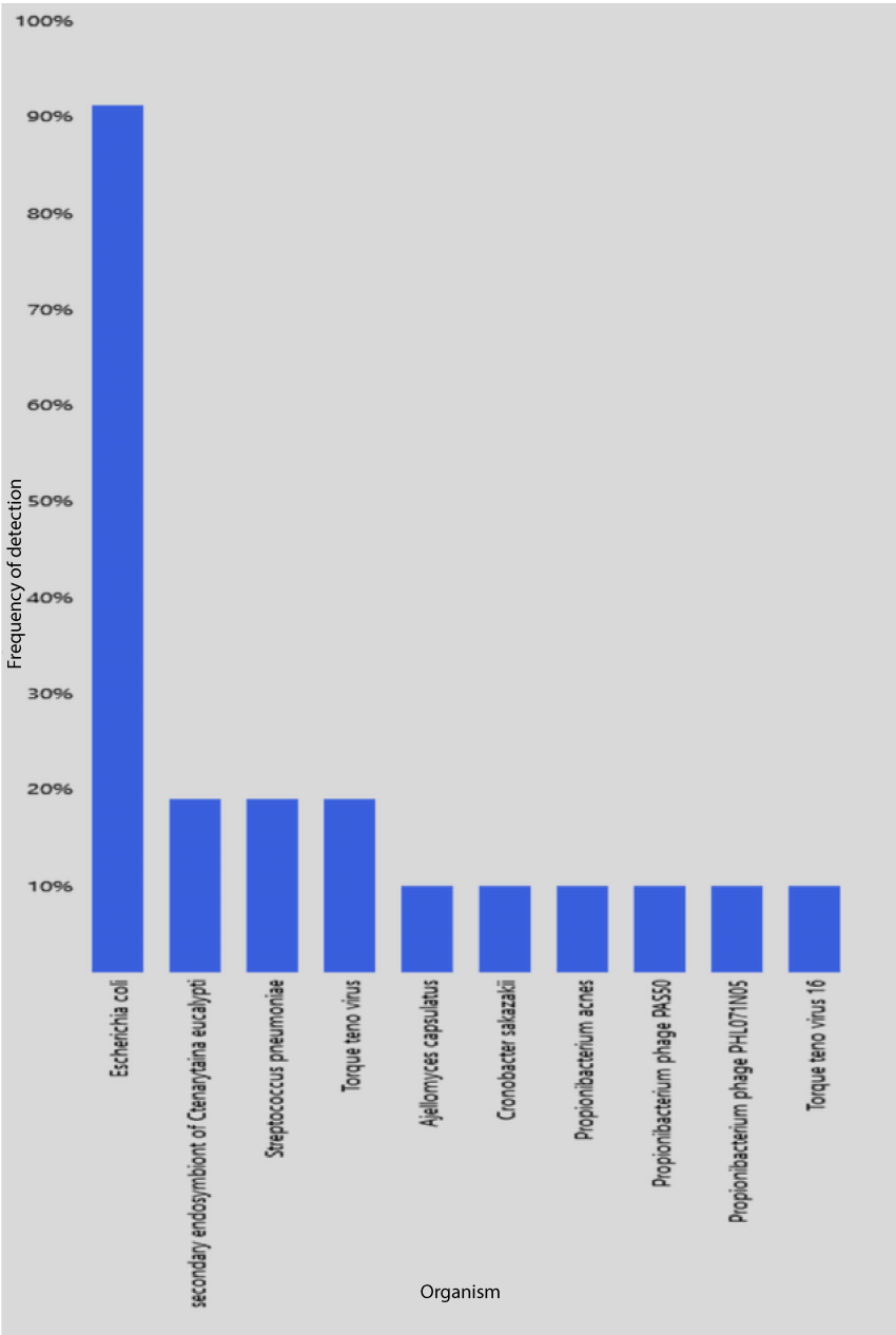
Figure 4.7: Summary of Axiom Microbiome Array results. All organisms detected in any of the 10 samples are depicted in the bar chart with the frequency of detection displayed on the y-axis.
