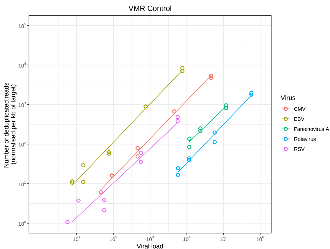
Figure 3.7: Relationship between viral load and sequencing yield in Viral Multiplex Reference samples. The VMR was sequenced at a range of dilutions in two replicates. For the five viruses in the VMR that had been quantified by the NIBSC using qPCR, the relationship between viral load and normalised sequencing yield is plotted.
