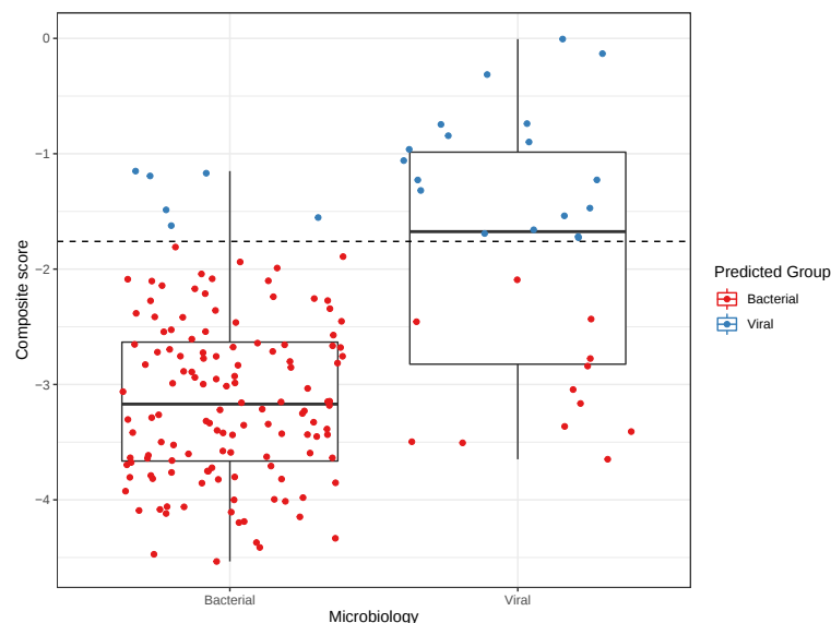
Figure 5.16: Boxplot of predictions from Sweeney seven-gene set. Each point corresponds to a patient. Actual microbiological groups are plotted on the x-axis whilst predicted classifications are denoted by point colour. Threshold for discriminating bacterial from viral infection (-1.76) is denoted by the dashed line. The composite score (y-axis) is derived from calculating the geometric mean of viral genes minus the geometric mean of bacterial genes, multiplied by the ratio of viral genes to bacterial genes (3/4).
