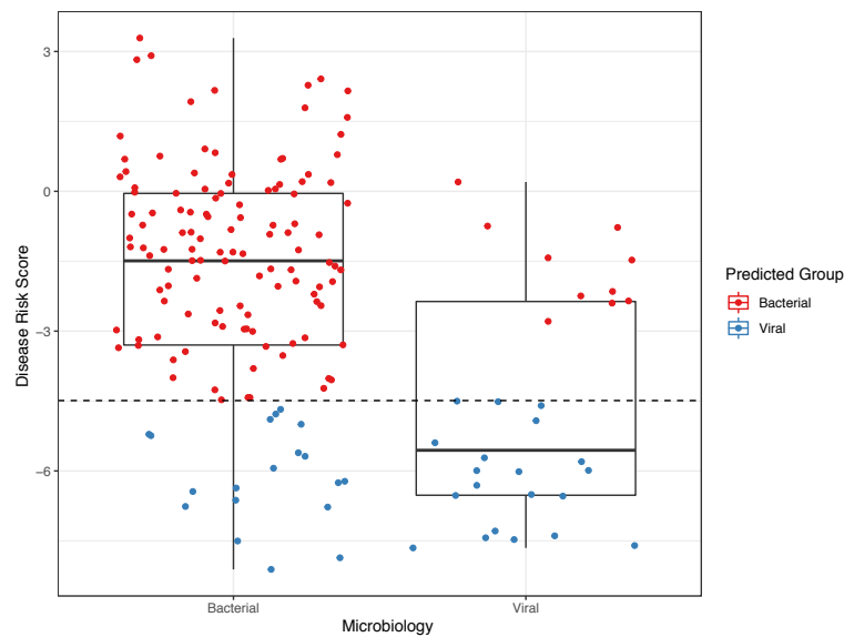
Figure 5.18: Boxplot of predictions from Herberg disease risk score. Each point corresponds to a patient. Actual microbiological groups are plotted on the x-axis whilst predicted classifications are denoted by point colour. Threshold for discriminating bacterial from viral infection (-4.49) is denoted by the dashed line. The composite score (y-axis) is derived from the disease risk score of FAM89A expression minus IFI44L expression.
