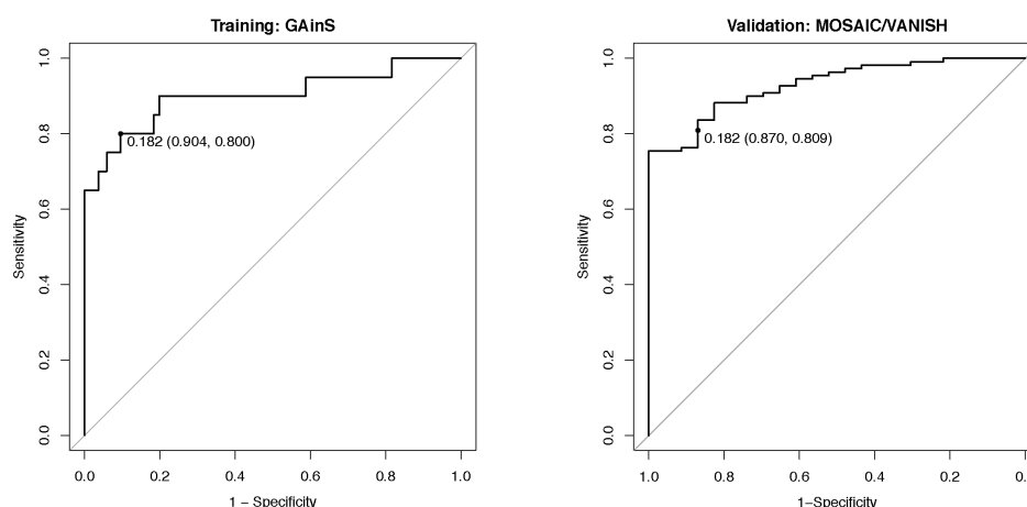
Figure 5.21: ROC analysis for influenza vs bacterial infection signature. The threshold for discriminating bacterial from influenza infection is noted (0.182), together with the specificity and sensitivity at that threshold in brackets. AUC for the training cohort was 90.1% (95% CI 80.4%-99.8%) whilst AUC for the combined validation cohort was 92.9% (95% CI 88.5%-97.4%). MR was 10.9% for the training cohort and 18% for the validation cohort.
