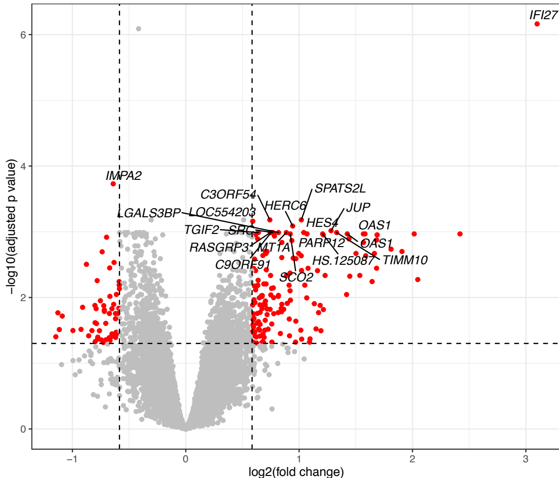
Figure 5.11: Volcano plot of differentially expressed probes in viral vs bacterial infection in GAIN patients with sepsis due to CAP. Probes in red are differentially expressed at a FDR <0.05 and fold change ≥1.5. Positive fold change corresponds to upregulation in individuals with viral infection. Top 20 significantly differentially expressed probes are labelled.
