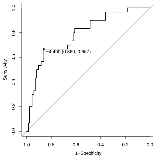
Figure 5.17: ROC analysis for Herberg disease risk score. The threshold for discriminating bacterial from viral infection is noted (-4.49), together with the specificity and sensitivity at that threshold in brackets. AUC for the GAINs cohort was 79% (95% CI 70%-88%).
