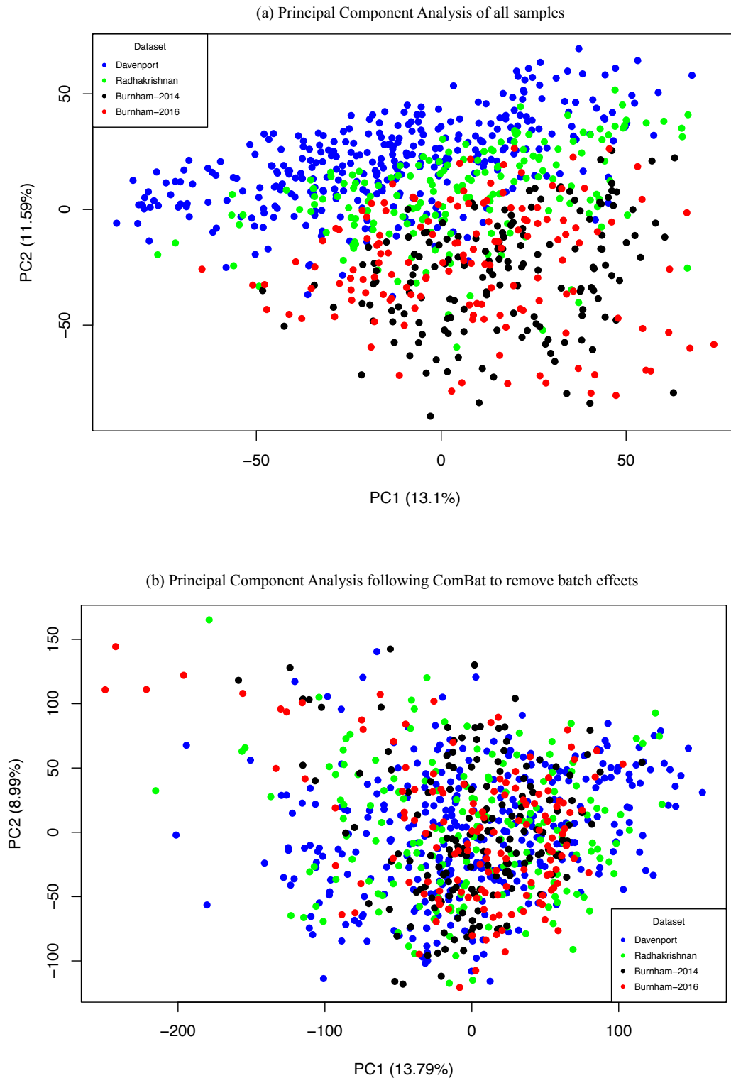
Figure 5.3: Principal Component Analysis: Combined dataset of 816 samples from GAINs CAP and FP patients. The first two principal components of the gene expression data are plotted, with the amount of variance explained by each noted; (a) prior to batch effects being removed, and (b) after removal of batch effects by ComBat. Samples are coloured according to the four datasets: Radhakrishnan (n=175), Davenport (n=339), Burnham-2014 (n=159), Burnham-2016 (n=143).
