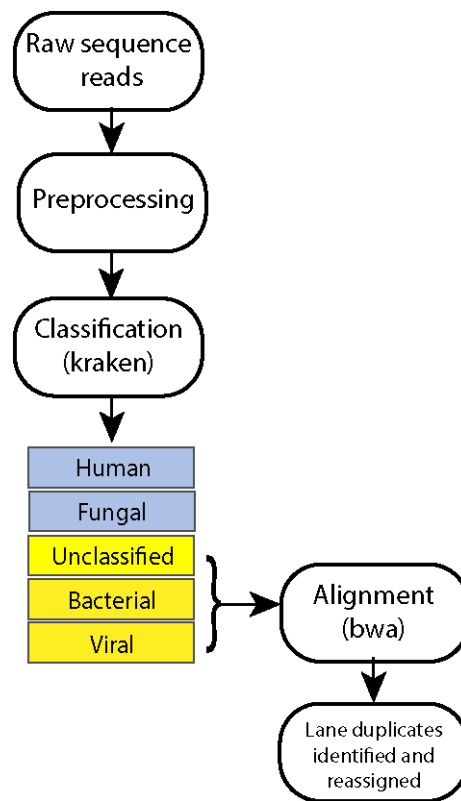
Figure 3.9: Data processing pipeline.
