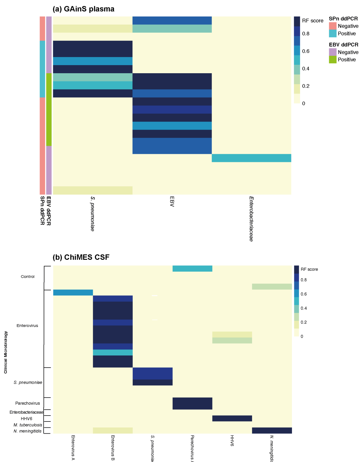
Figure 4.3: Performance of Castanet : GAINs/ChiMES test dataset. Performance of Castanet in clinical samples with a positive microbiology diagnosis. The test dataset included 50 samples: (a) 22 plasma samples (20 GAINs, 2 sepsis-negative controls); (b) 28 CSF samples (24 ChiMES, 4 meningitis-negative controls). The combined overall test dataset specificity and sensitivity was 0.986 and 0.867 respectively. Only organisms detected in each sample set are included as columns in each panel. RF=random forest; HHV6=human herpes virus 6; SPn= Streptococcus pneumoniae
