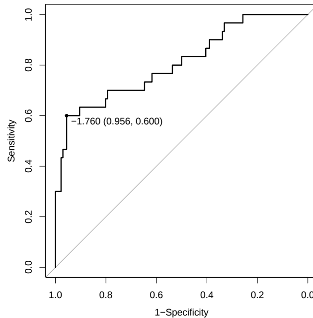
Figure 5.15: ROC analysis for Sweeney seven-gene set. The threshold for discriminating bacterial from viral infection is noted (-1.76), together with the specificity and sensitivity at that threshold in brackets. AUC for the GAINs cohort was 81% (95% CI 71%-90%).
