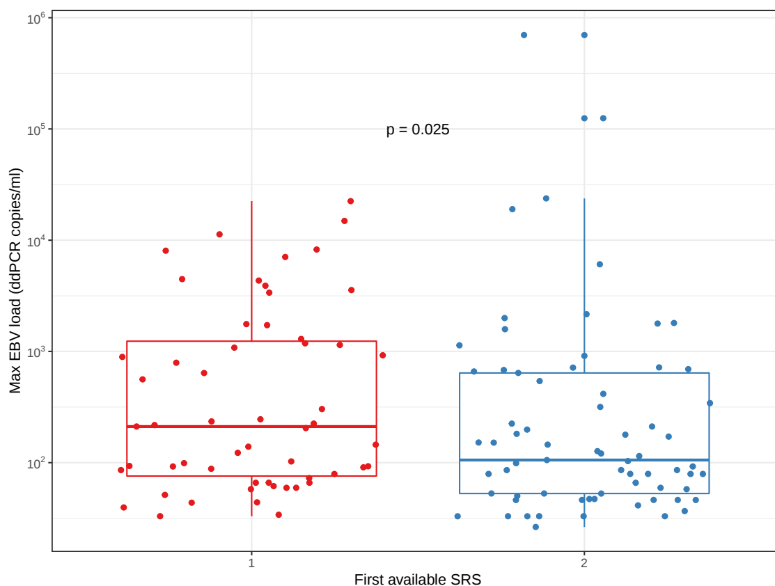
Figure 5.6: Boxplot of maximum EBV load over the first 5 days of ICU admission (ddPCR) against SRS status at the first available timepoint after ICU admission. GAINs patients with sepsis due to CAP were analysed with respect to EBV viral load by ddPCR and SRS endotype by genome-wide gene expression microarray analysis from peripheral blood leukocytes.
