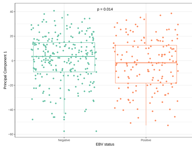
Figure 5.5: Boxplot of SRS at the first available timepoint as a continuous trait against EBV status over the first five days of ICU admission. GAINs patients with sepsis due to CAP for whom gene expression data and EBV status are available are included here (n=391). The values for principal component 1 (PC1) provide a continuous measure of SRS endotype with higher values representing an SRS2 endotype and lower values representing an SRS1 endotype.
