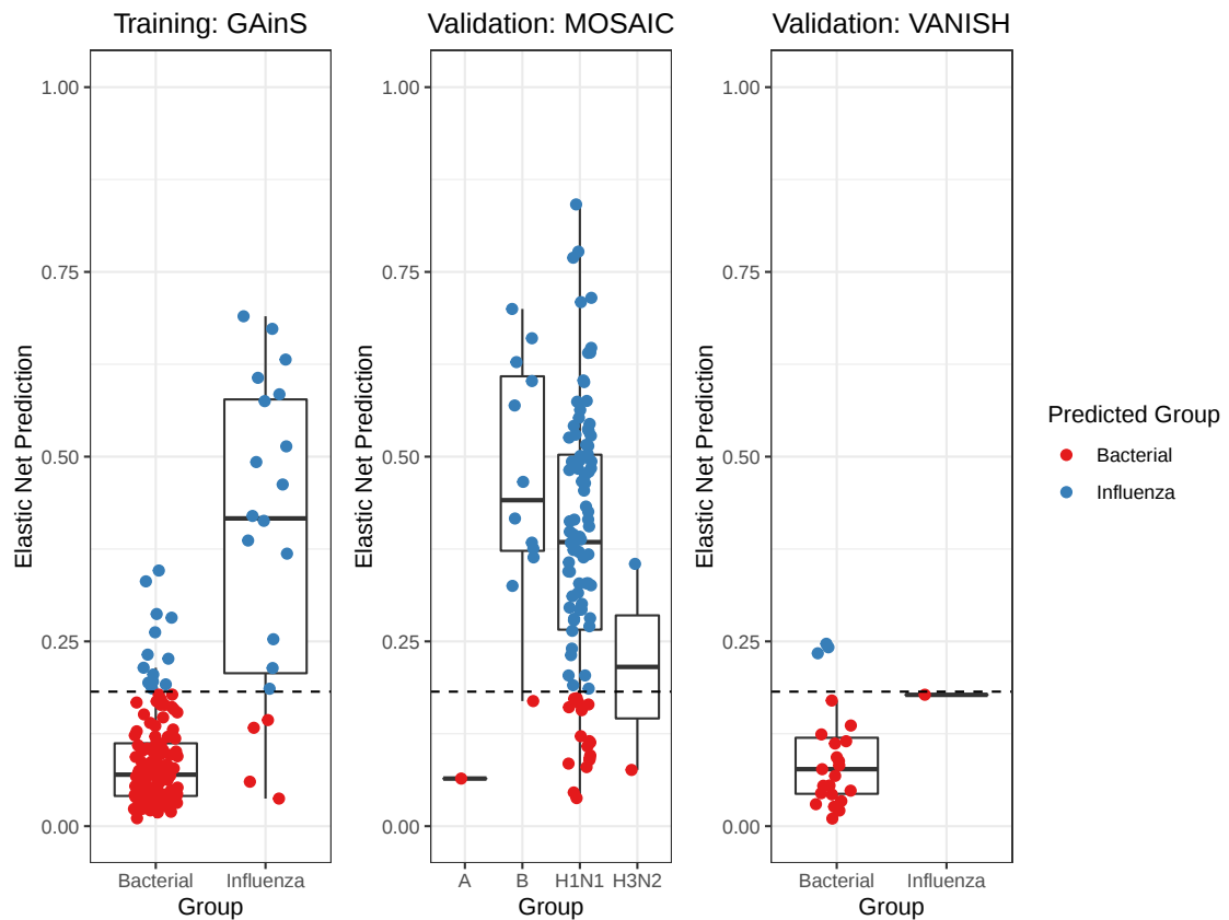
Figure 5.22: Boxplot of predictions from influenza vs bacterial infection gene signature in GAINs patients with sepsis due to CAP. Each point corresponds to a patient. Actual microbiological groups are plotted on the x-axis whilst predicted classifications are denoted by point colour. The MOSAIC groupings correspond to influenza virus types. Threshold for discriminating bacterial from influenza infection is denoted by the dashed line. The elastic net prediction value (y-axis) can range from 0 (indicating bacterial infection) to 1 (indicating influenza infection).
