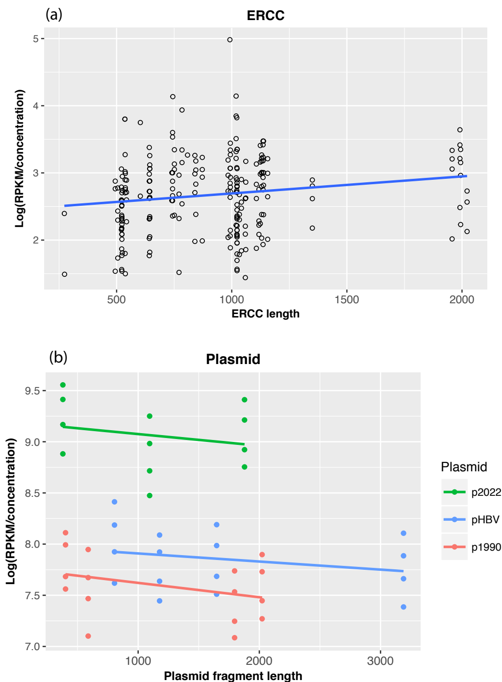
Figure 3.4: Relationship between sequencing yield and fragment length. (a) ERCC, (b) plasmid. The y-axis displays read count normalised for fragment length, total read count per sample, and fragment concentration. RPKM = reads per kilobase of fragment per million reads.
