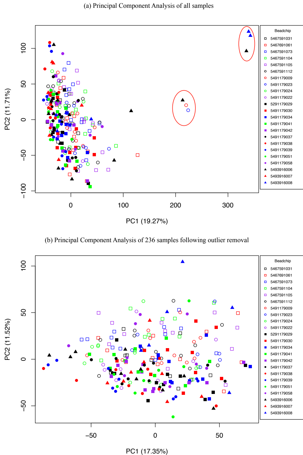
Figure 5.1: Principal Component Analysis: Radhakrishnan 2010. The first two principal components of the gene expression data are plotted, with the amount of variance explained by each noted; (a) when all samples are included in the analysis, and (b) after the removal of six outliers. Samples are coloured according to beadchip and outlying samples are circled in red.
