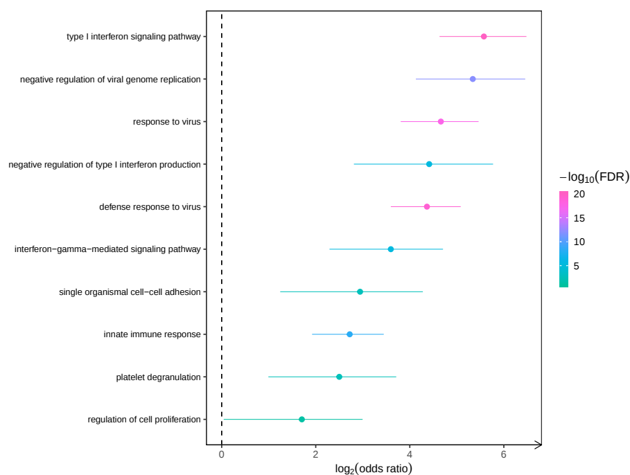
Figure 5.12: Pathway enrichment for viral infection in GAINs patients with sepsis due to CAP. The differentially expressed probes between patients with viral and bacterial infection were used to determine pathway enrichment with XGR. The top ten most enriched pathways using the Gene Ontology database are shown.
