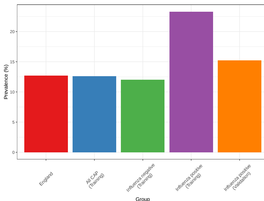
Figure 5.24: Bar graph of HLA-B*35 prevalence in GAIN patients with sepsis due to CAP. The percentage of individuals with at least one HLA-B*35 allele is plotted on the y-axis.
