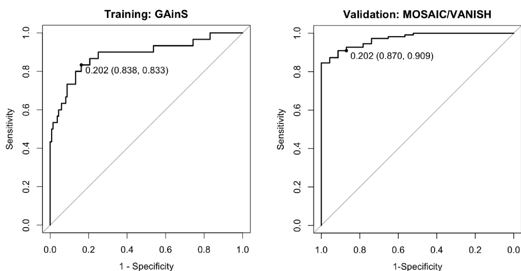
Figure 5.13: ROC analysis for viral vs bacterial infection signature in GAINs patients with sepsis due to CAP. The threshold for discriminating bacterial from viral infection is noted (0.202), together with the specificity and sensitivity at that threshold in brackets. AUC for the training cohort was 88.6% (95% CI 80.7%-96.5%) whilst AUC for the combined validation cohort was 97.1% (95% CI 94.6%-99.5%). MR was 16.3% for the training cohort and 9.8% for the validation cohort.
