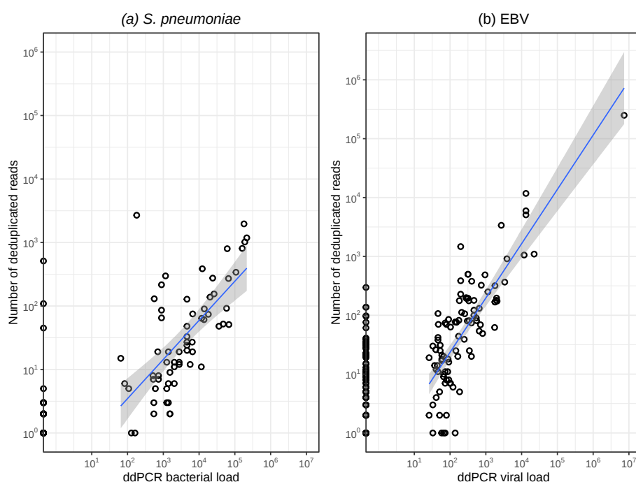
Figure 4.5: Relationship between organism load and sequencing yield in sepsis samples. De-duplicated read yield was plotted against pathogen load, estimated by ddPCR in samples from a subset of cases in which (a) Streptococcus pneumoniae (n=102) or (b) Epstein-Barr virus (EBV) (n=199) was detected by sequencing. A linear relationship between pathogen load and sequencing yield was observed for each organism ( S. pneumoniae : Pearson's R^2 = 0.449 , p = 8.8 \times 10^{-5} ; EBV: Pearson's R^2 = 0.702 , p = 2.9 \times 10^{-16} .)
