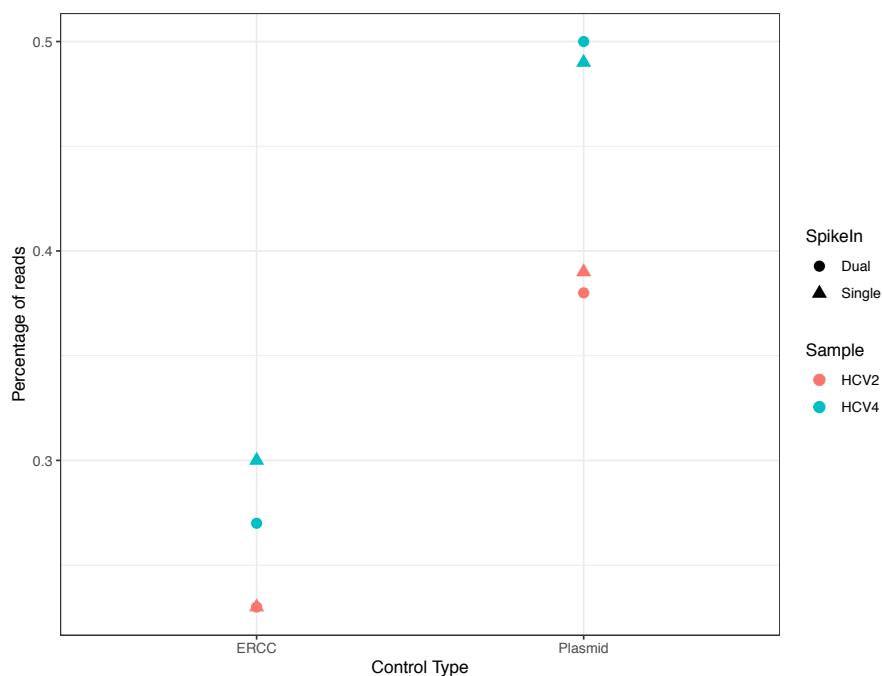
Figure 3.3: Sequencing yield of controls Yield of ERCC and plasmid compared between aliquots receiving single and dual spike-ins.
