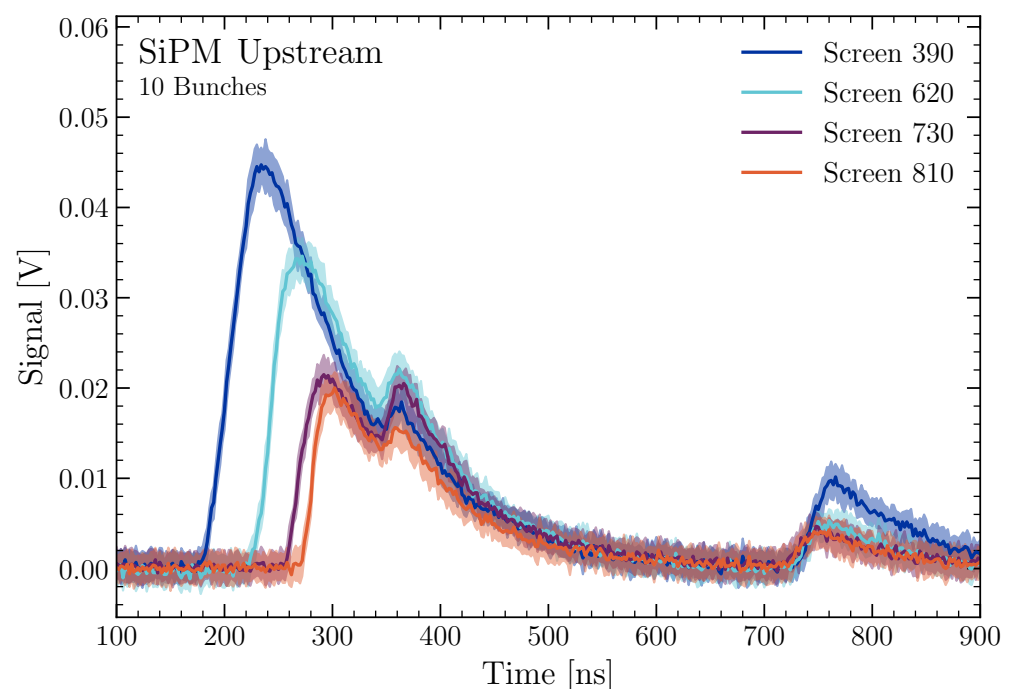
Figure 8. A plot showing the measured upstream waveforms, read out with a SiPM at 43 V for loss signals created by a 10 bunch beam. The time in nanoseconds is shown on the x-axis, with the signal in volts on the y-axis. To visualise statistical fluctuations, the standard deviation on the waveforms are given by the transparent bands.
