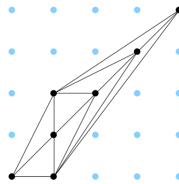
Figure 1: Triangulation of the toric diagram for Y^{4,2} . The number of gauge groups in the associated quiver theory is given by the number of triangles, which in this case is equal to eight.
