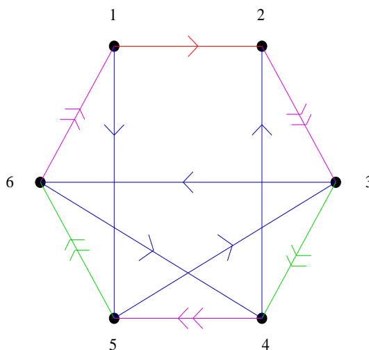
Figure 9: Quiver diagram for Y^{3,2} .
