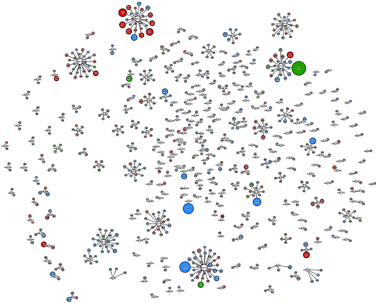
Fig. 5. User-Post bipartite graph for the FB-AG group. Users are visualized as white nodes where the size represent how active the user is. Posts are coloured (red, green, blue) based on the sentiment analysis of the text (negative, positive, neutral, respectively).
