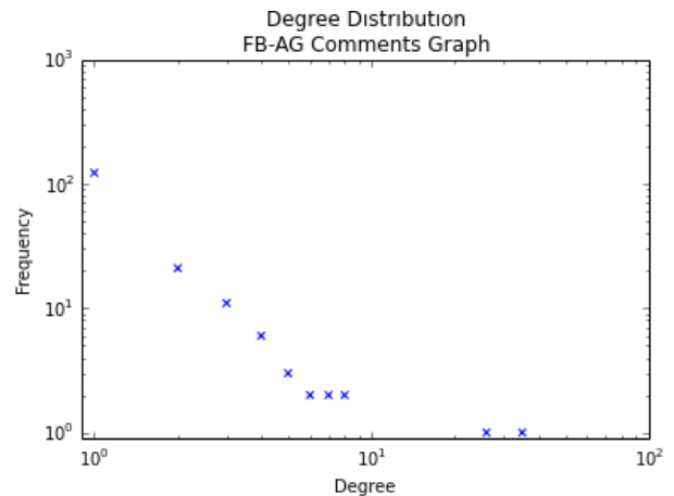
Fig. 3. Facebook-AG Comments Network Degree Distribution.
