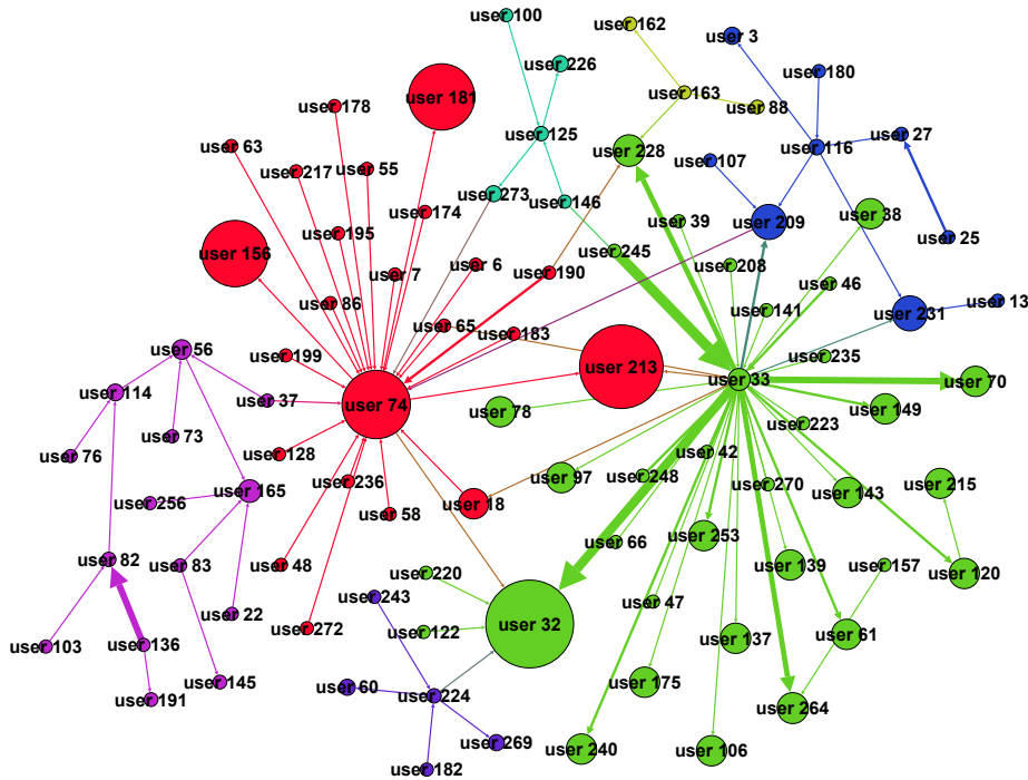
Fig. 4. Facebook-AG Comments Network- Nodes size represent the nodes Eigenvector Centrality
