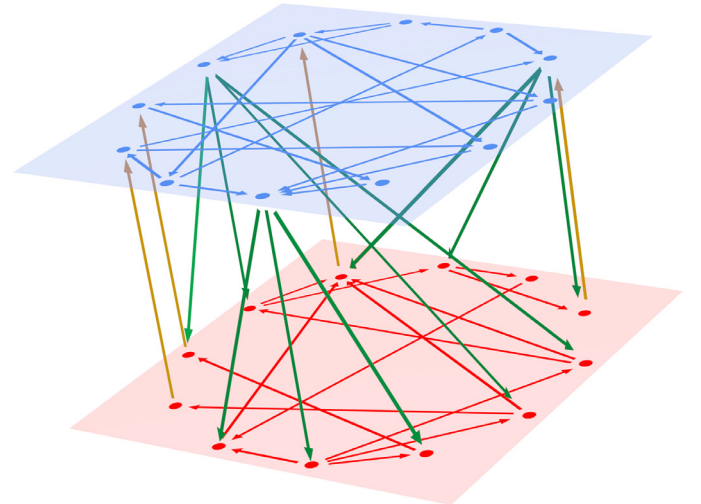
Fig. 2. The duplex network underlying the shock transmission matrix A . The nodes represent institutions and the edges represent the shock transmission between institutions. In this two-layer system, the top layer represents the liquidity shock network (in blue) and the bottom layer the valuation shock network (in red). The green and yellow arrows represent interactions between these two networks; the green arrow represents conversions of shocks from liquidity to valuation, whereas yellow arrows represent the conversion of shocks from valuation to liquidity. The shock transmission matrix is a weighted adjacency matrix that describes both layers and their interactions simultaneously.
