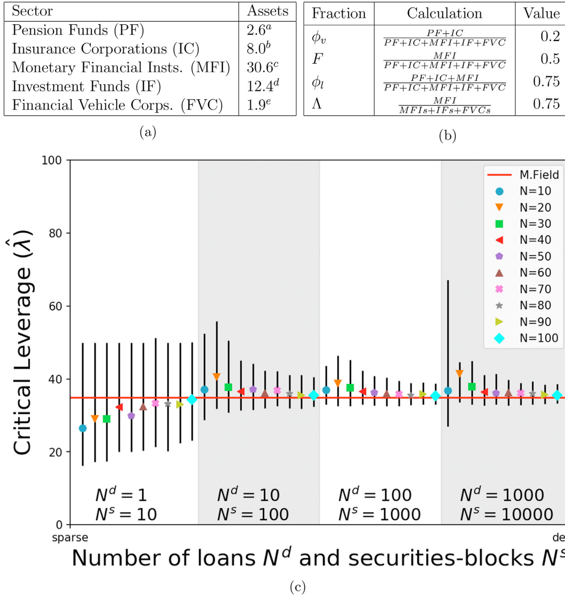
Fig. 4. Comparison of the mean field model to randomly generated financial systems. The plot compares the critical leverage (horizontal line) predicted by the mean field model, Eq. (15), to the critical leverages of randomly generated financial systems. For various combinations of the number of loans N^d , the number of securities-blocks N^s and the number of institutions N , we generate 500 random systems and plot the median (using various markers to indicate the number of institutions) and the 15 th to 85 th percentile interval (vertical bars) of the distribution of critical leverages. The simulated values converge to the predictions of the mean-field model as N^d , N^s , N increase. a Source: http://sdw.ecb.europa.eu/reports.do?node=1000005664 ; accessed November 3 rd 2018 b Source: http://sdw.ecb.europa.eu/reports.do?node=1000005659 ; accessed November 3 rd 2018 c Source: http://sdw.ecb.europa.eu/reports.do?node=1000005718 ; accessed November 3 rd 2018 d Source: http://sdw.ecb.europa.eu/reports.do?node=1000003516 ; accessed November 3 rd 2018 e Source: http://sdw.ecb.europa.eu/reports.do?node=1000003621 ; accessed November 3 rd 2018
