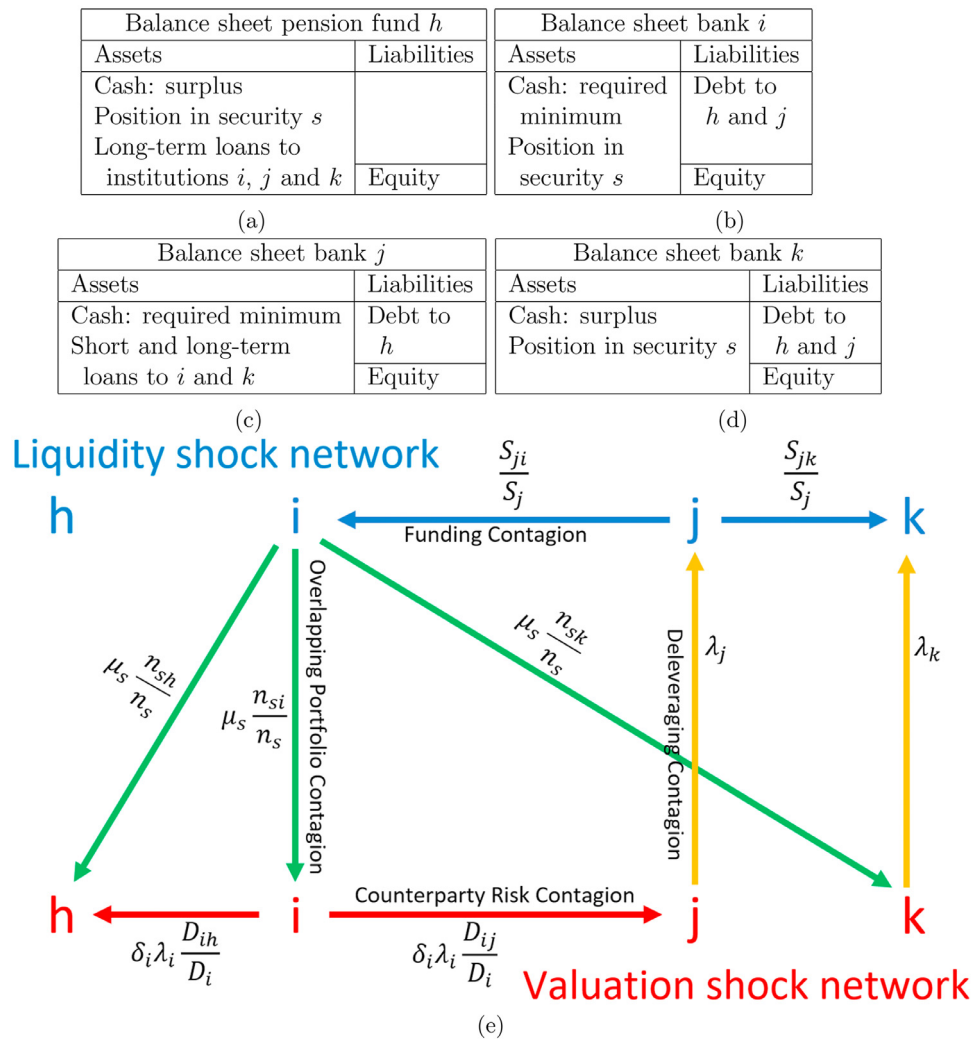
Fig. 3. A stylized example illustrating the interaction of multiple channels of contagion. Consider four institutions, h , i , j and k , whose balance sheets are given at the top of the figure. Each institution's liquidity is represented by a node in the liquidity shock network, while each institution's solvency is represented by a node in the valuation shocks network. The label of an edge indicates the type of contagion transmitted (each node transmits a single type of contagion so only one of a node's out-edges is labeled) and the expression next to the edge represents the size of the interaction. The out-edges of a node in the liquidity shock network give the node's response to liquidity shocks and are dictated by the asset that sits at the top of the institution's pecking order. Similarly, out-edges in the valuation shock network give the response to valuation shocks as given by the institution's leverage strategy: unleveraged (institution h ), passively leveraged (institution i ), or leverage targeting (institutions j and k ).
