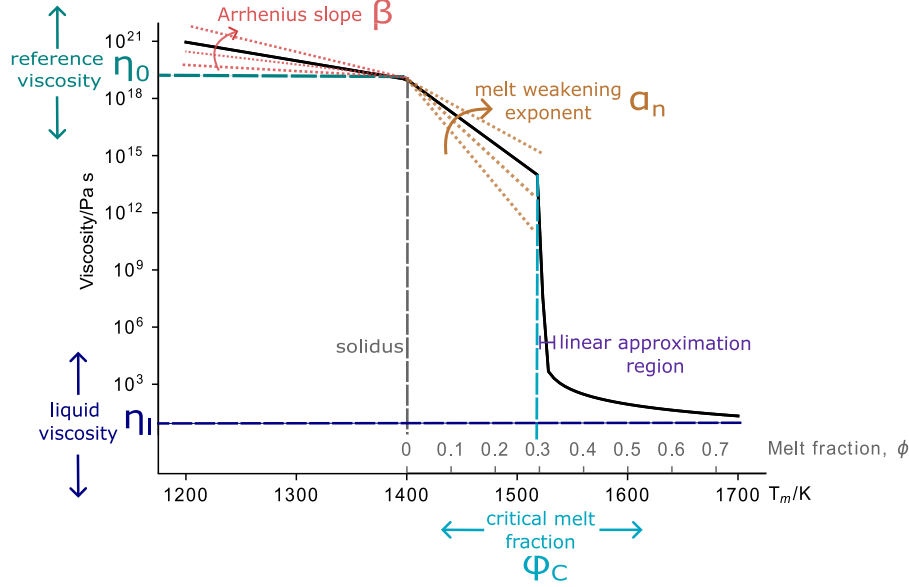
Fig. 2. Variation of mantle viscosity with temperature (solid black line) for \eta_0 = 10^{19} Pa s, \phi_C = 0.3 , \beta = 0.0225 K ^{-1} , \alpha_n = 30 , and \eta_l = 10 Pa s. The effect of varying each parameter is shown by the coloured arrows and lines. The grey, upper ticks on the horizontal axis indicates the equivalent melt fraction for temperatures above the solidus for mantle solidus and liquidus temperatures of 1400 K and 1800 K, respectively. (For interpretation of the references to colour in this figure legend, the reader is referred to the web version of this article.)
