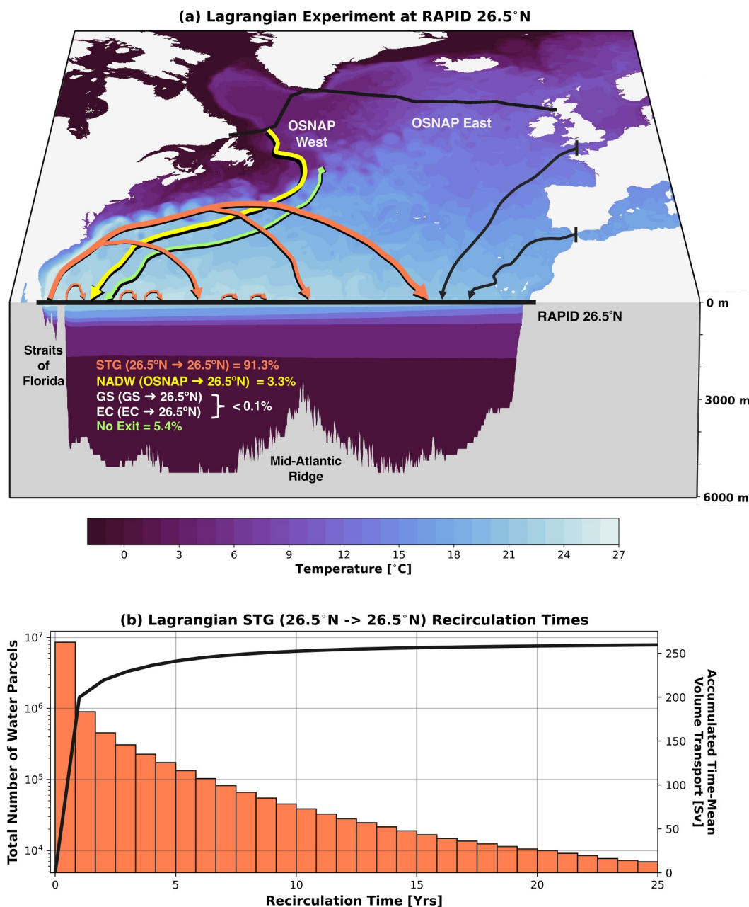
Figure 1. (a) Schematic representation of the Lagrangian pathways north of the RAPID array at 26.5°N. (b) Distribution of recirculation times for STG water parcels returning to 26.5°N within the 25-year maximum advection period. The solid black line overlaid shows the accumulation of the time-mean volume transport (Sv) of the STG pathway as a function of water parcel recirculation time.
