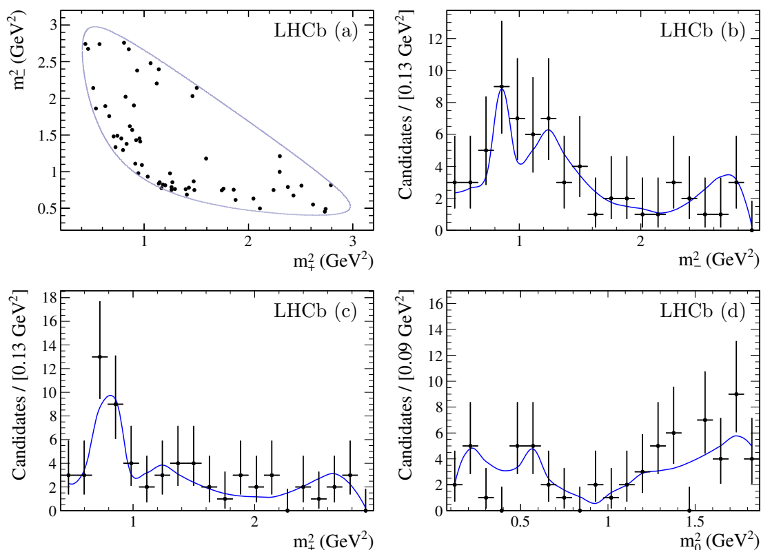
Figure 3. Selected B^0 \rightarrow DK^{*0} candidates, shown as (a) the Dalitz plot, and its projections on (b) m_-^2 , (c) m_+^2 and (d) m_0^2 . The line superimposed on the projections corresponds to the fit result and the points are data.
