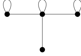
Fig. 7. The graph 2-Wrench.
