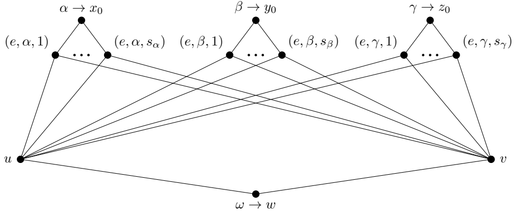
Fig. 6. The graph J(e) for e = \{u, v\} . A label of the form a \rightarrow b means that the vertex a \in V(G) is pinned to b \in V(H) since S_a = \{b\} .
