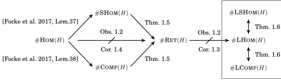
Fig. 1. Approximate counting complexity landscape. An arrow from a problem A to a problem B means that there exists an AP-reduction from A to B . A struck through arrow corresponds to a reduction with a separation. The references for the reduction and the separation are given above and below the arrow, respectively.
