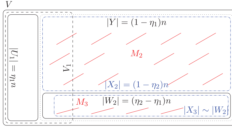
FIGURE 3 | A diagram illustrating the inclusion relationships and relative sizes of the sets V, V_1, U_1, Y, X_2, W_2, X_3 constructed during Stages I–III in the proof of Theorem 1.4, in addition to the location of the matchings M_2, M_3 .
