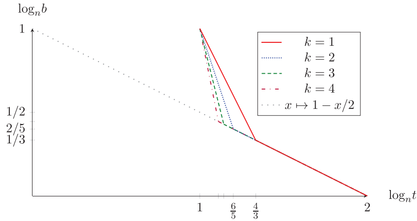
FIGURE 2 | Budget thresholds for C_{2k+1}, C_{2k+2} .
