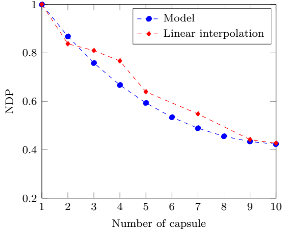
Figure 6: Comparison of the predicted normalized differential pressure (NDP) based on a linear interpolation and our model for ten capsules in counter-current configuration.
