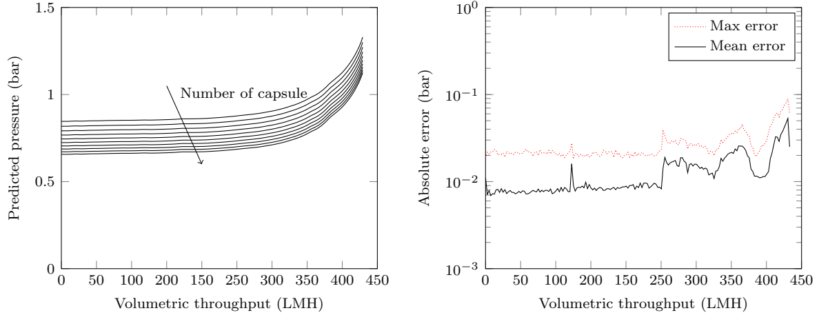
(a) Prediction for a ten-capsule co-current depth filter, (b) Maximum and mean absolute error between the predicted and measured pressures for all capsules
