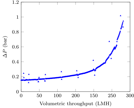
(a) Measured differential pressure when challenging a single capsule with a homogenized/whole-yeast mixture at 300 LMH
