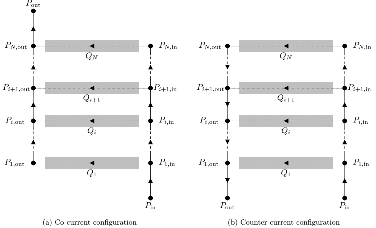
Figure 1: Schematic of a multi-capsule depth filter in co-current (left) and counter-current (right) configuration. Each capsule is represented by a horizontal line, with the shaded rectangles representing the depth filters. The fluid enters the device at the inlet, marked by P_{in} , and leaves it at the outlet, marked by P_{out} .
