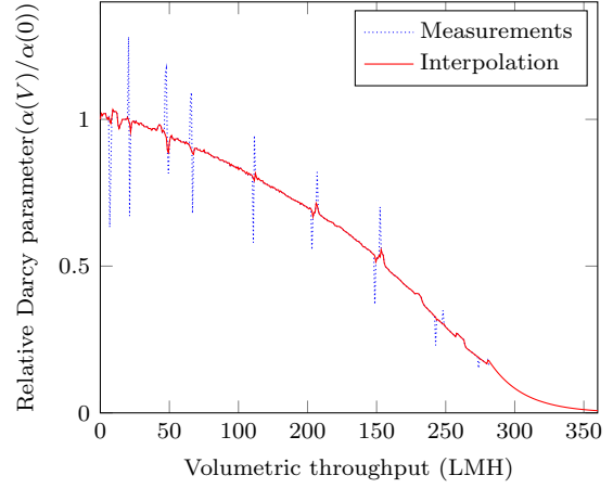
(b) Interpolated and normalized Darcy parameter in dependency of the volumetric throughput
