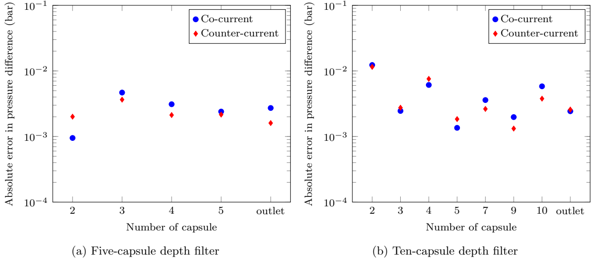
Figure 2: Validating the model. We plot the average error between the predicted and measured pressure at each capsule based on clean-water flow tests with 100, 200 and 300 LMH.
