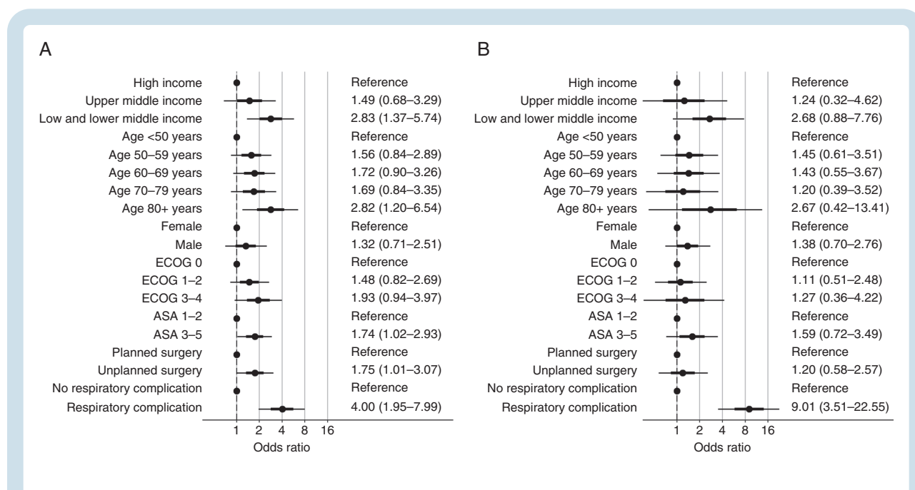
Figure 2. Bayesian multilevel logistic regression models on 30-day postoperative mortality in 1010 patients. (A) Forest plot of odds ratios from the Bayesian multilevel logistic regression on 30-day postoperative mortality using informative priors. (B) Forest plot showing odds ratios from sensitivity analysis using weakly informative priors to assess the influence of informative priors on the posterior distributions of the odds ratios.
