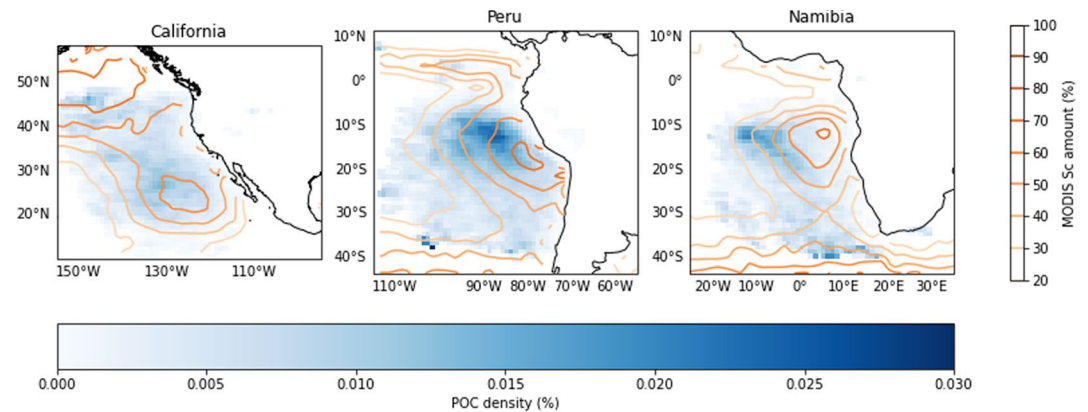
Figure 3. The percentage density of detected POCs in the three regions of interest with the MODIS climatological stratocumulus amount overlaid. The POC data set represents an average between 2005 and 2018, while the MODIS stratocumulus amount is averaged over 2003–2011. MODIS, Moderate Resolution Imaging Spectrometer; POC, pockets of open cell.
