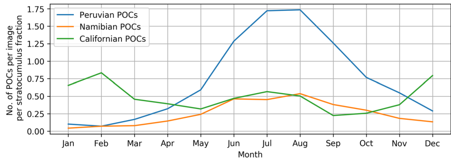
Figure 2. Temporal distribution of POC occurrences detected in MODIS true-color imagery by our algorithm for the three regions studied, normalized by the number of images used and the average stratocumulus cloud amount in that region. MODIS, Moderate Resolution Imaging Spectrometer; POC, pockets of open cell.
