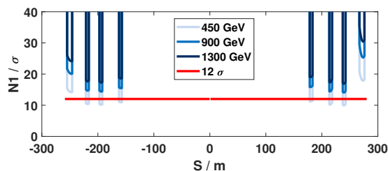
Figure 3: Beam stay clear in IR4 matching quadrupoles for various injection energies
