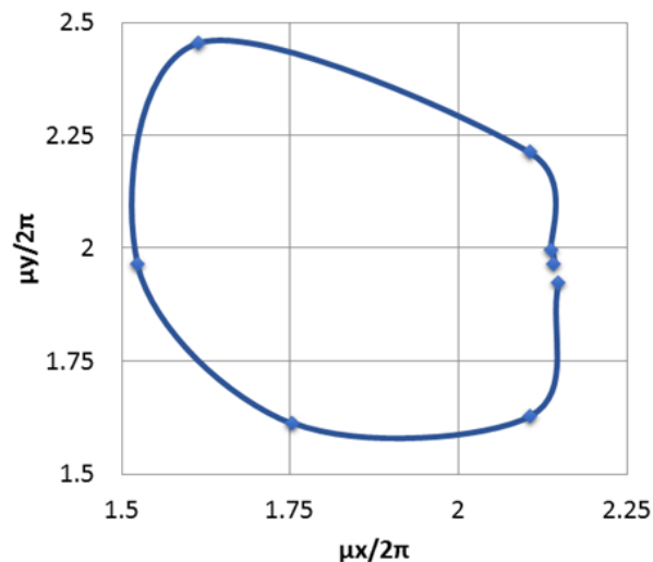
Figure 5: Diagram showing tune range achievable by using Q4 in RF insertion
