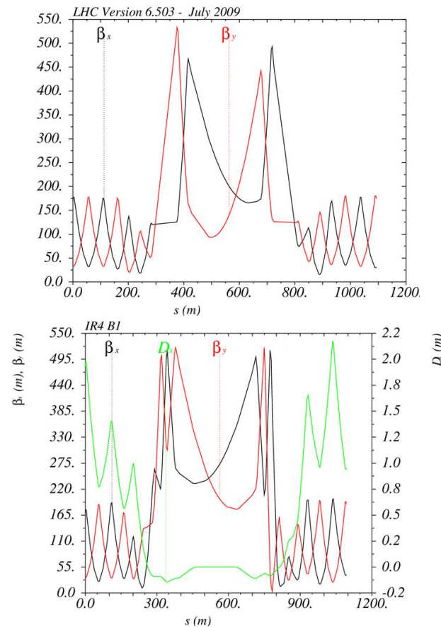
Figure 2: Comparison between the \beta functions in LHC (above) and HE-LHC IR4
