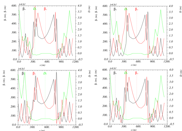
Figure 4: Optics of IR4 matched to change the phase advance in the IR as much as possible
