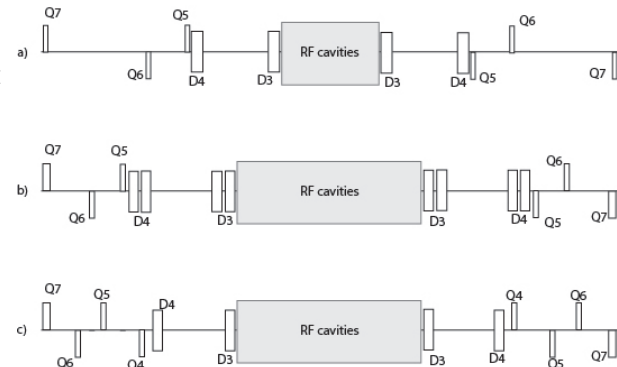
Figure 1: Diagrams of the different designs of IR4 for beam 1. a) IR4 in current LHC, b) IR4 design doubling the number of dipoles, c) IR4 final design using FCC technology and additional quadrupoles for tuning.
