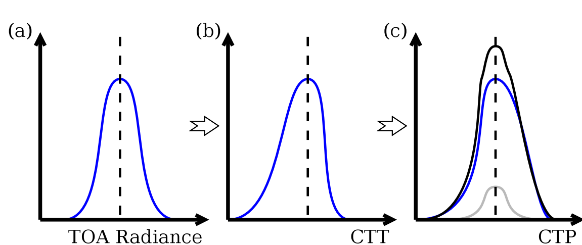
Fig. 2: Distorting the distribution of error when measuring cloud top radiance, temperature or pressure.
