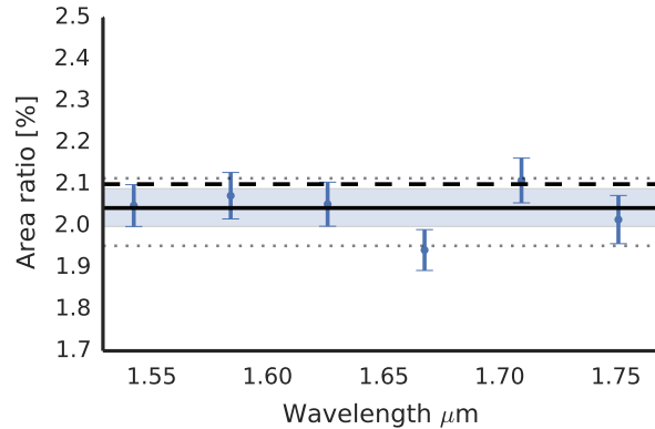
Figure 10. WASP-19b transmission spectrum from the mock dataset. The dots show the area ratio posterior medians, the errorbars correspond to the 68% posterior central intervals, the continuous black line shows the wide H-band area ratio posterior median, the shaded region its 68% posterior central interval, and the slashed black line the prior mean. The dotted lines show the area ratio values set to fourth and fifth passbands, while all other passbands have the same area ratio as the wide passband.
