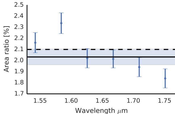
Figure 8. WASP-19b transmission spectrum estimated from the partial transit. The dots show the area ratio posterior medians, the errorbars correspond to the 68% posterior central intervals, the continuous black line shows the posterior median for the wide H-band area ratio, the shaded region its 68% posterior central interval, and the slashed black line the prior mean.
