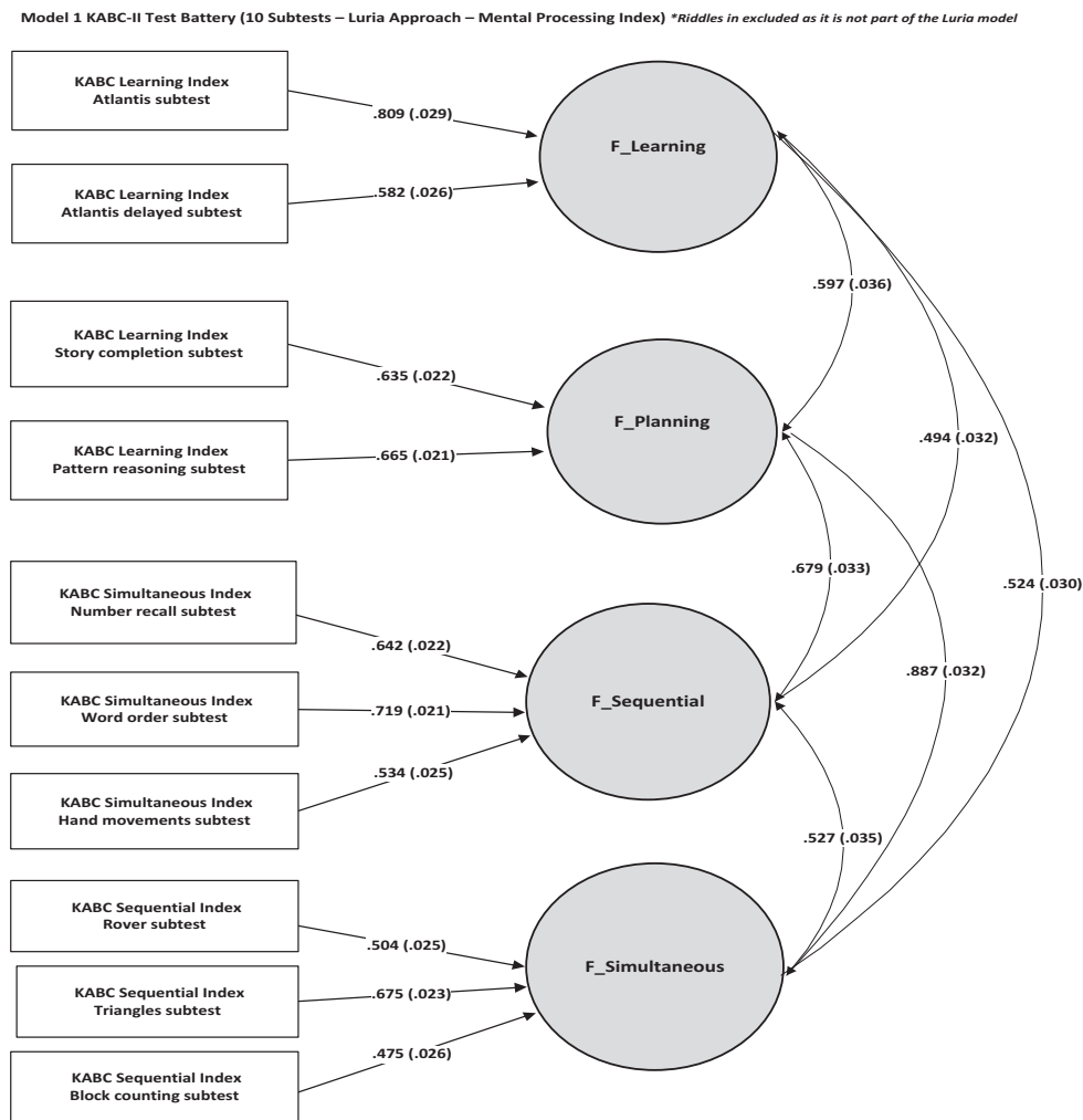
Figure 3. Cognitive model.
