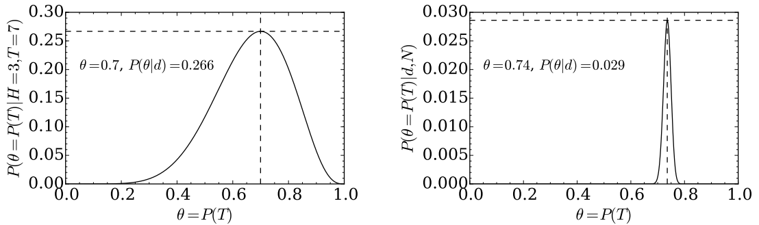
Figure 2.3: The unnormalised posterior probability calculated for multiple hypotheses for the probability of tossing a tails, P(T) in the case of 10 data points (left) and 1000 data points (right). The dashed lines in both cases show the posterior probability values at the peak of the distribution.
