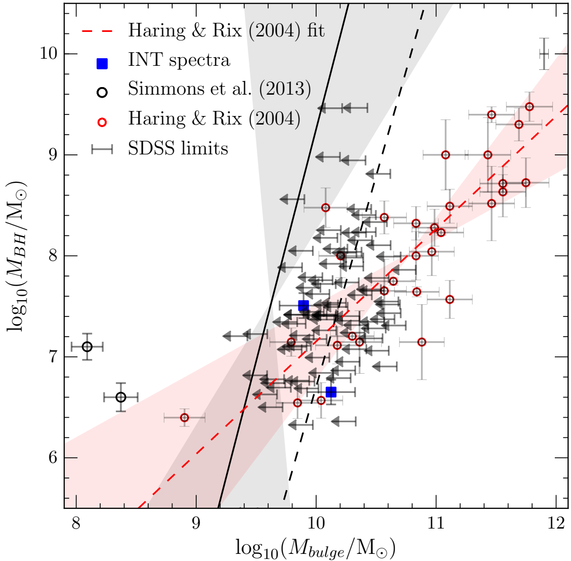
Figure 4.19: The upper limits on the calculated stellar bulge masses are plotted against the black hole mass for the BULGELESS sample. The best fit to these upper limits and two-dimensional errors using linear regression methods (solid line) is shown with \pm 3\sigma (grey shaded). The dashed line shows the fit if the upper limits are not treated as such. I also show the best fit found using this same method to the early-type galaxies of Häring & Rix (2004) (dashed line) with \pm 3\sigma (red shaded) and the measured values shown by the red circles. Despite the fact that the BULGELESS galaxies are predominantly disc dominated they will be most likely to lie above the Häring & Rix (2004) relationship found for bulge dominated systems (see discussion in Section 4.2.4).
