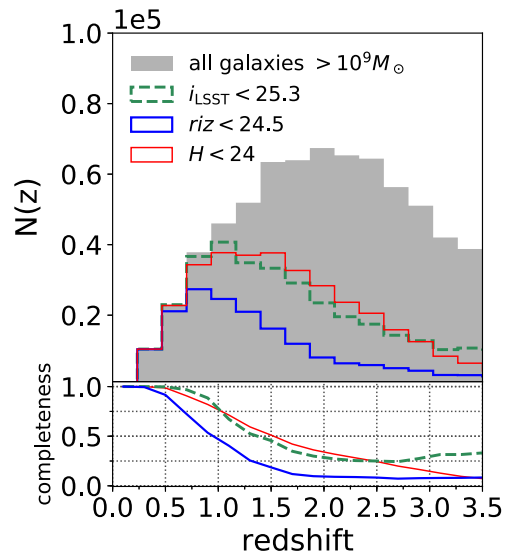
Figure 8. Redshift distribution N(z_{\text{sim}}) of HORIZON-AGN simulation (grey histogram, M > 10^9 M_{\odot} ) along with the N(z) of different sub-samples selected at H < 24 , riz < 24.5 , and i < 25.3 (upper red, lower blue, and green dashed histograms). For each sub-sample, the completeness fraction as a function of z_{\text{sim}} is shown in the bottom panel using same colours.
