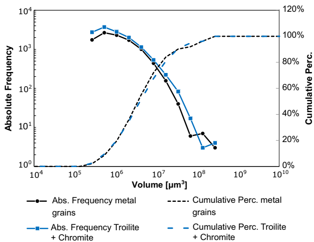
FIGURE 5. Grain size frequency distribution for metal phases and troilite+chromite phases. Cumulative frequency curves are also reported. The two phases display similar grain size distribution, with troilite+chromite being characterized by a larger number of grains per size class overall.
