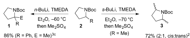
Scheme 1. Lithiation–Electrophile Trapping of \alpha -Substituted N -Boc-pyrrolidines 2
