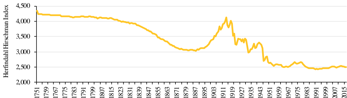
Figure 5: Hirschman–Hirfendahl concentration index of global energy supplies
